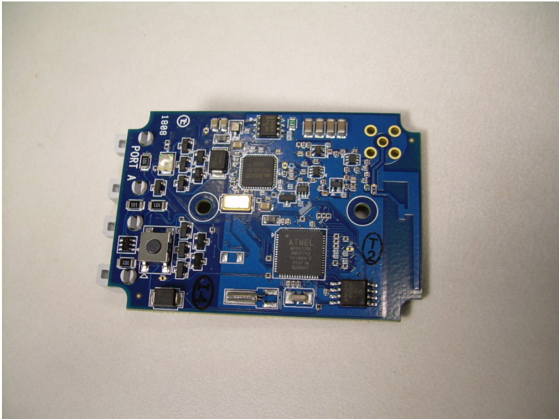
Bottom Side of the PCB with PCB Trace Antenna
