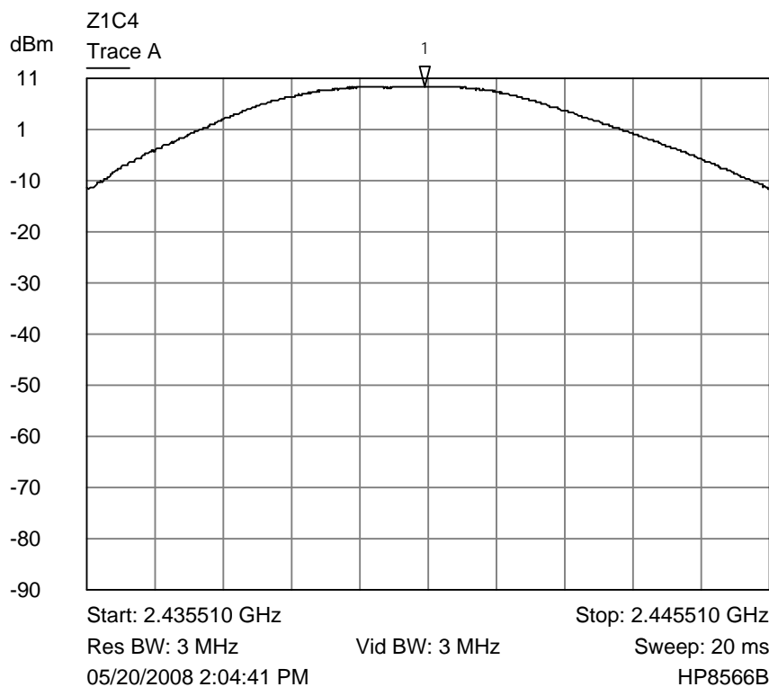
Trace A fMiddle channel output power plot
