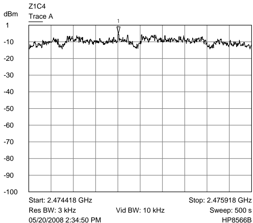
Trace A Upper channel 3 kHz power spectral density plot
