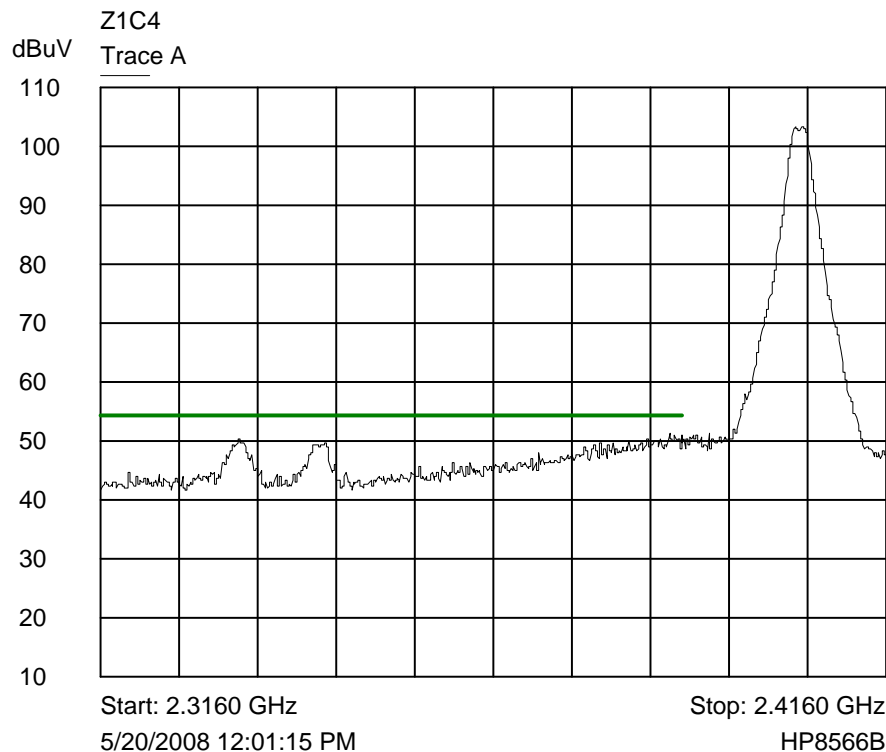
Trace A Radiated lower band edge - corrected - peak detection vs average limit
