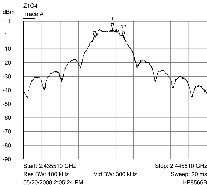
Trace A fMiddle channel bandwidth plot
