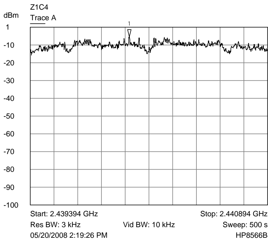
Trace A fMiddle channel 3kHz power spectral density plot
