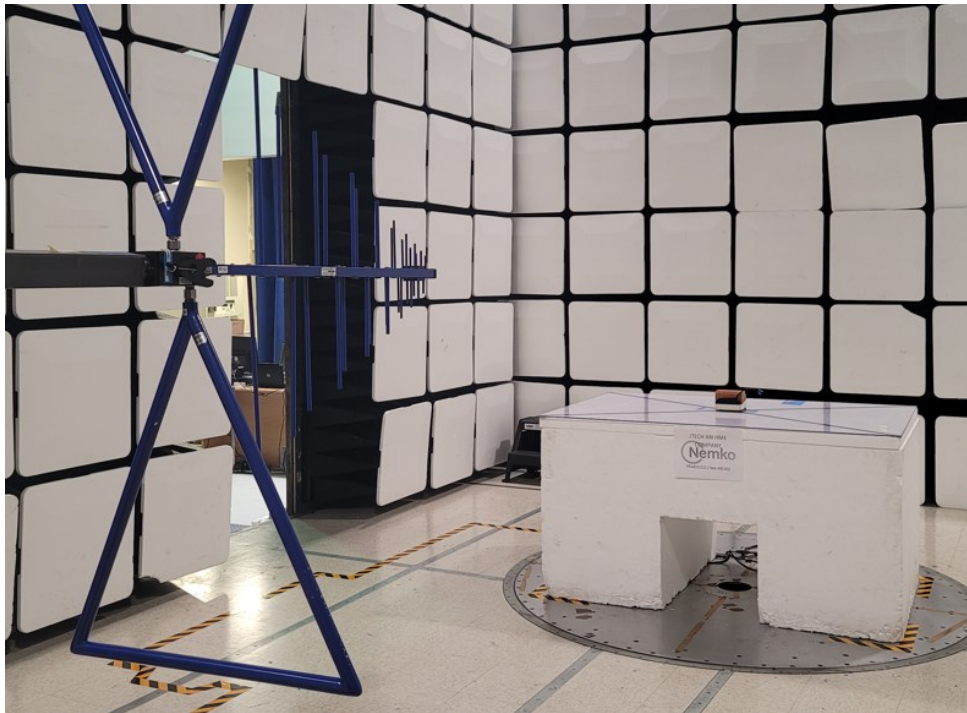
Figure 2 - Radiated emissions below 1 GHz (0.03 – 1 GHz), front view.
