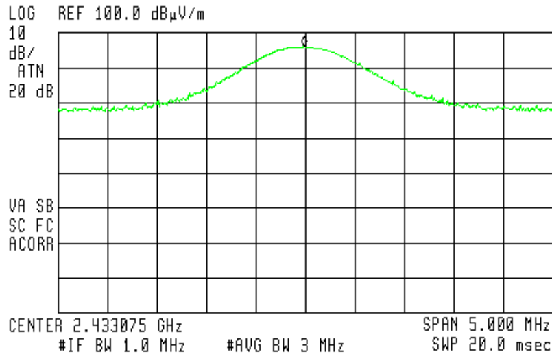
Figure 11 2433 MHz
