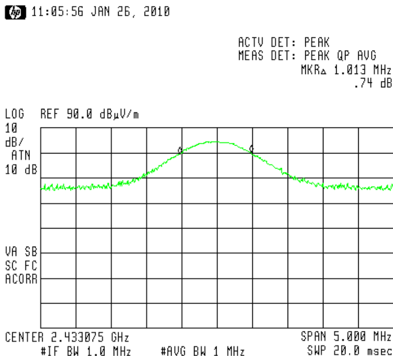
Figure 8. 2433 MHz
