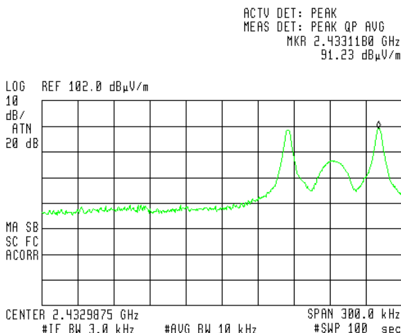
Figure 20 — 2433 MHz
