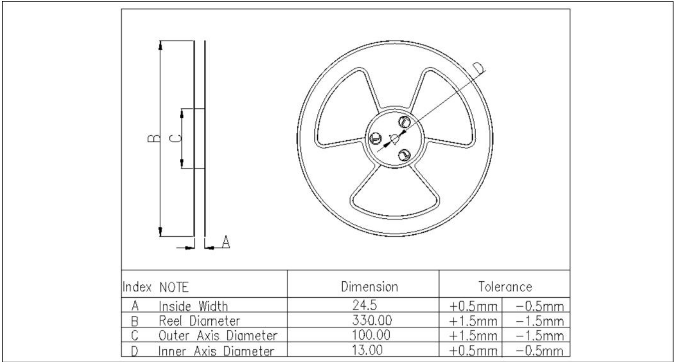
Figure 10 Reel dimensions
