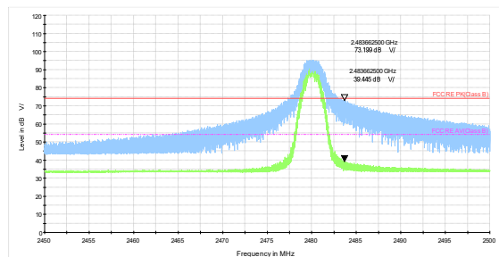
3DH5-Channel 78: Peak + Average
