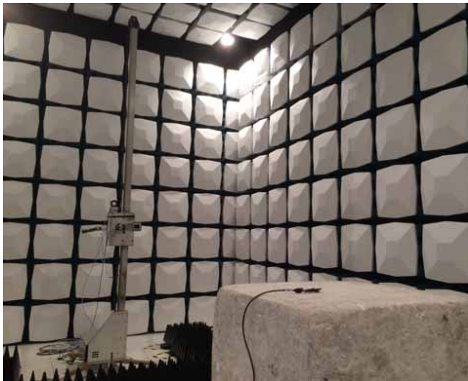
Description: Radiated Emission Test Setup for 18~40GHz
