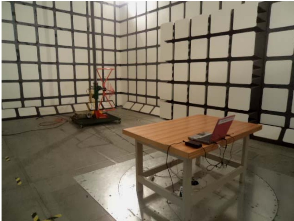
Below 1 GHz: Radiated Emissions (Charging Mode) - Rear View
