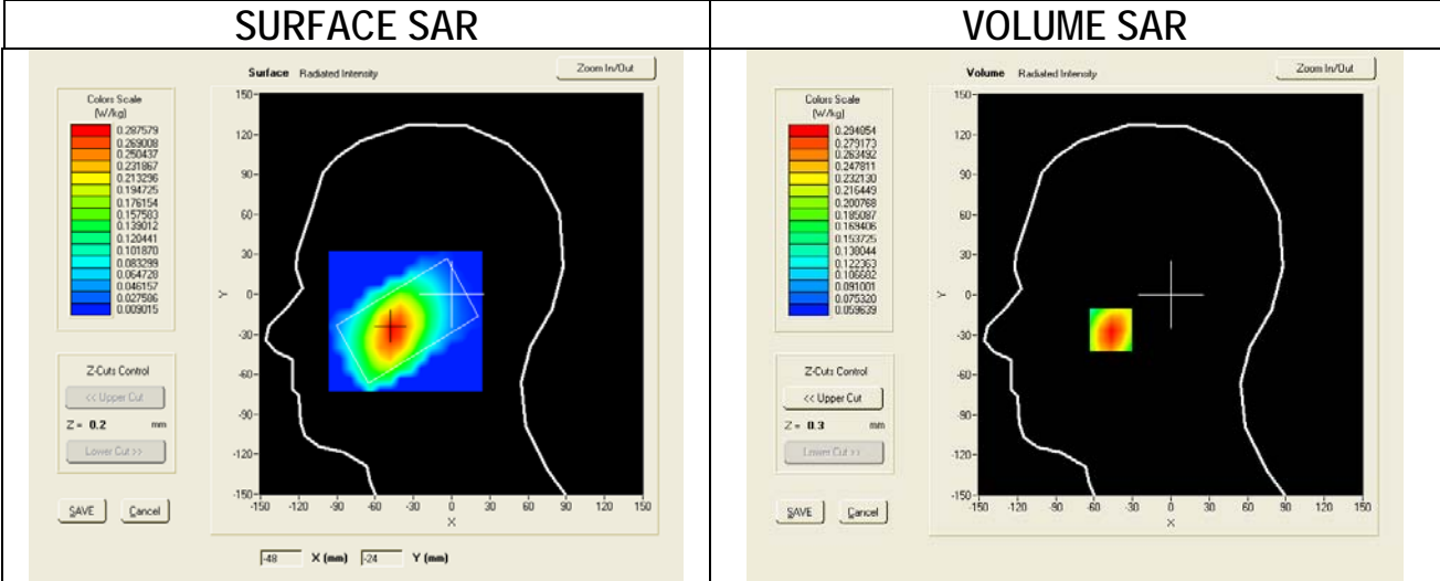
SAR, Z Axis Scan (X = -47, Y = -26)
