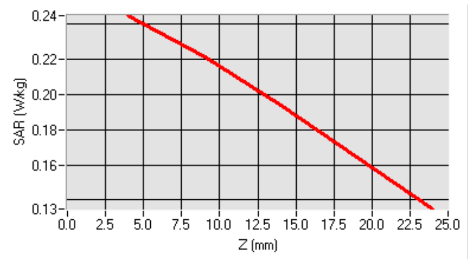
SAR, Z Axis Scan (X = -48, Y = -32)
