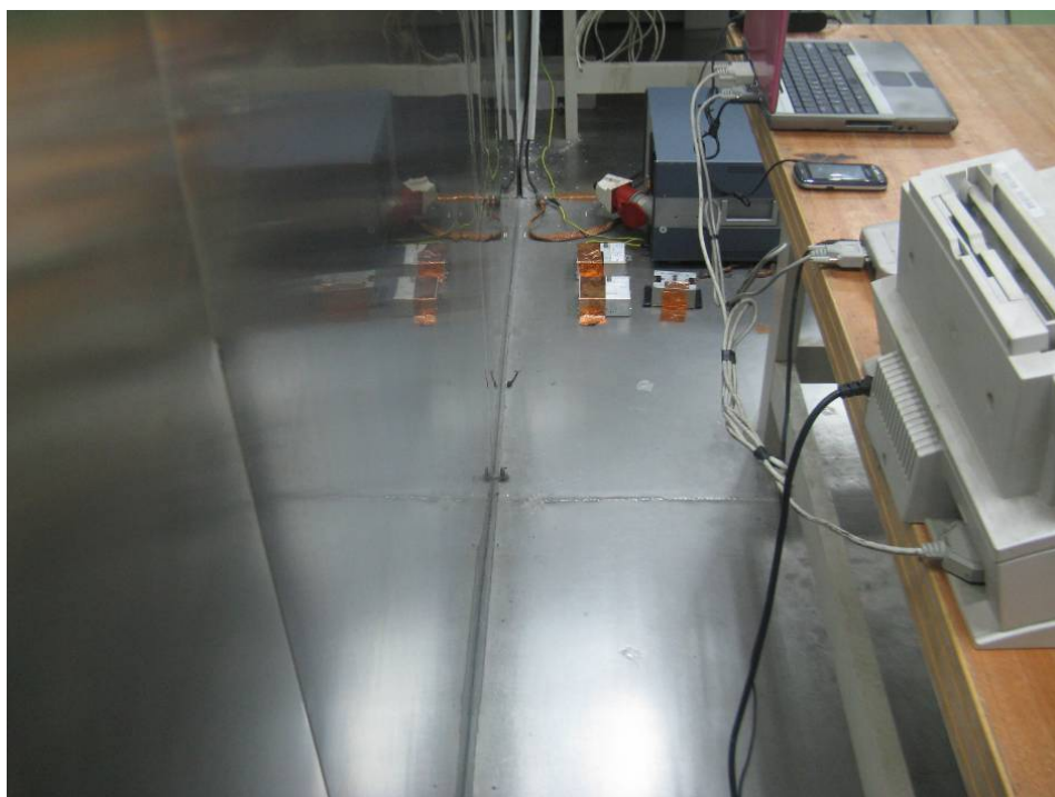
Conduction Emissions - Side View (Downloading Mode)
