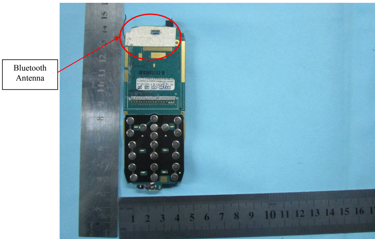
Mainborad With Shielding - Rear View
