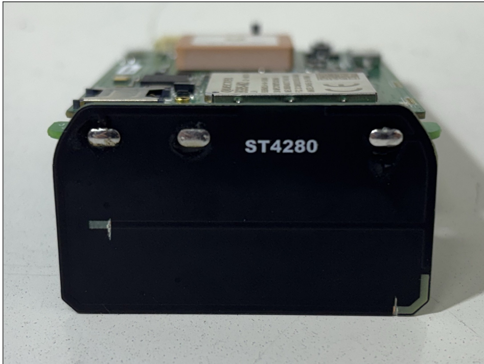
Top view of PCB Antenna
