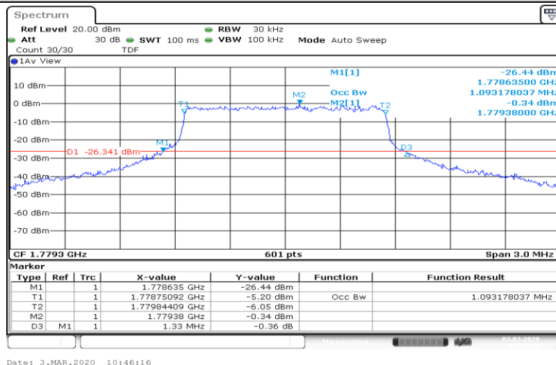
Band66-1.4MHz-QPSK-132665-6RB#0-1.093
