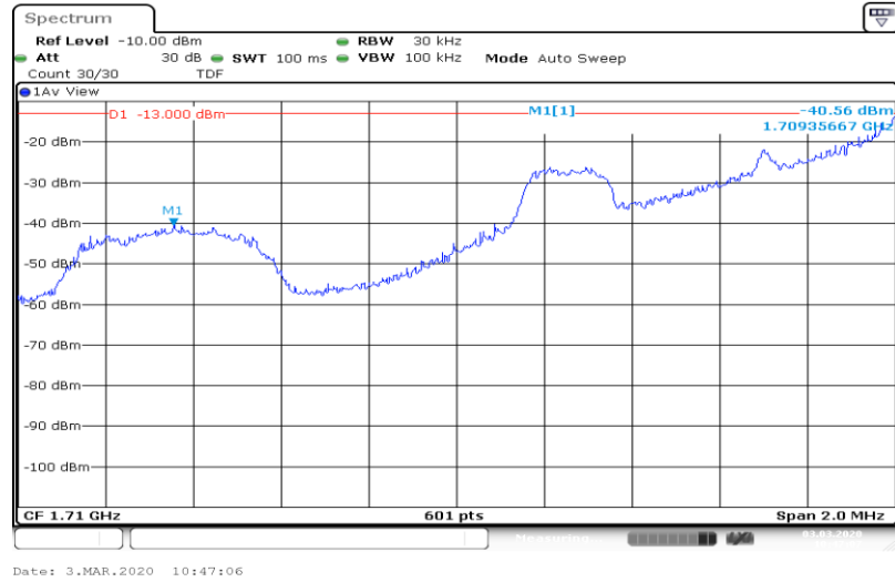
Band66-1.4MHz-QPSK-131979-1RB#0
