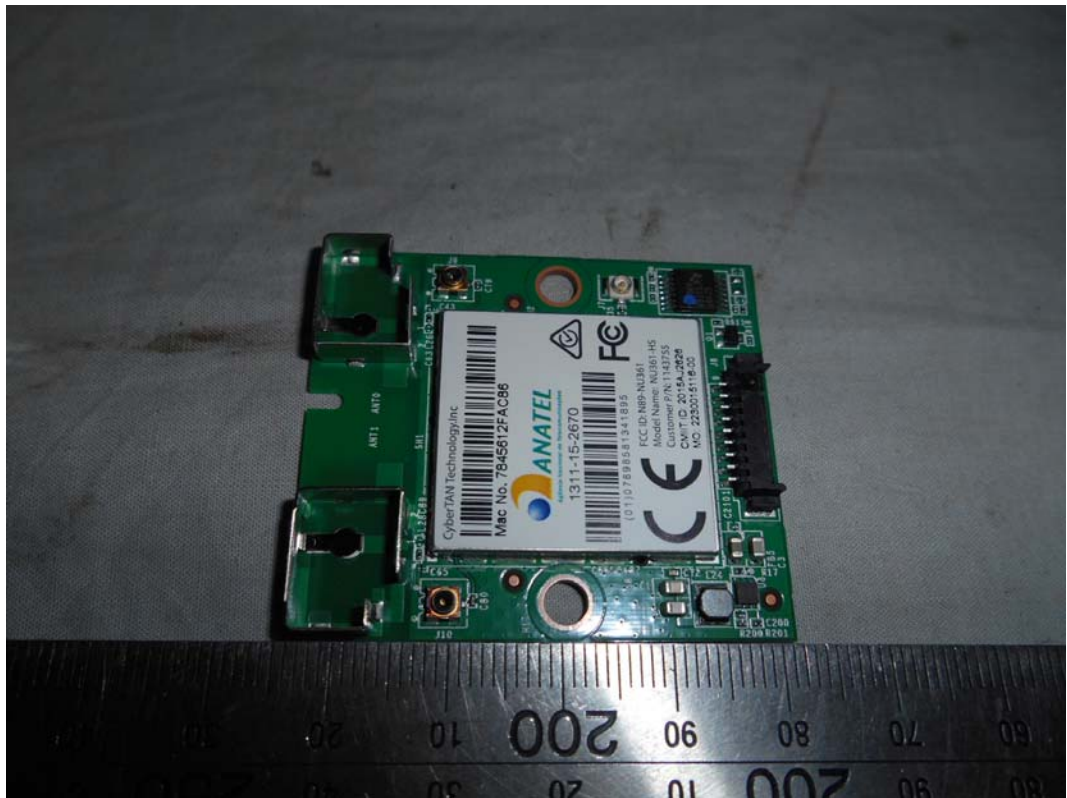
FIGURE 13 LED LCD TV (M/N: LC-50N6000U) RF BOARD (COMPONENT SIDE)
