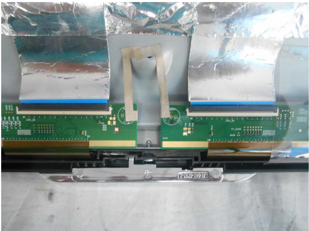
FIGURE 25 LED LCD TV (M/N: LTDN55K3201GUWUS) DEBUG #2
