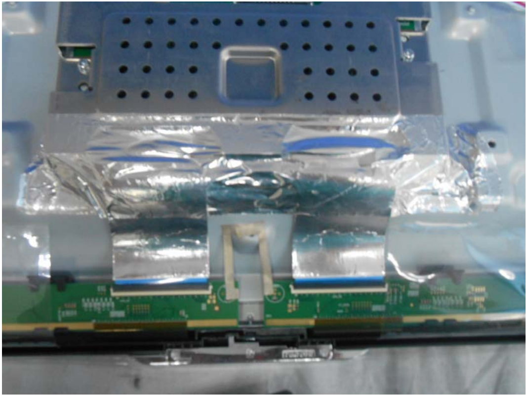
FIGURE 24 LED LCD TV (M/N: LTDN55K3201GUWUS) DEBUG #1
