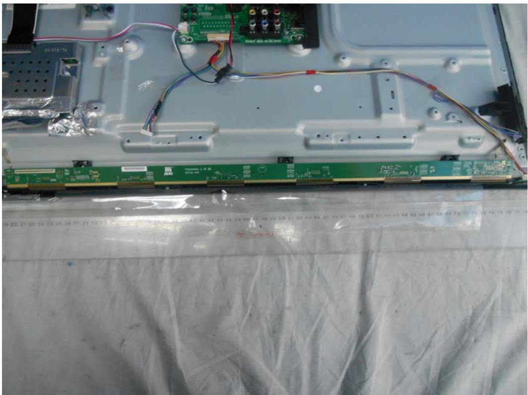
FIGURE 21 LED LCD TV (M/N: LTDN55K3201GUWUS) CONTROL BOARD #2 (COMPONENT SIDE)
