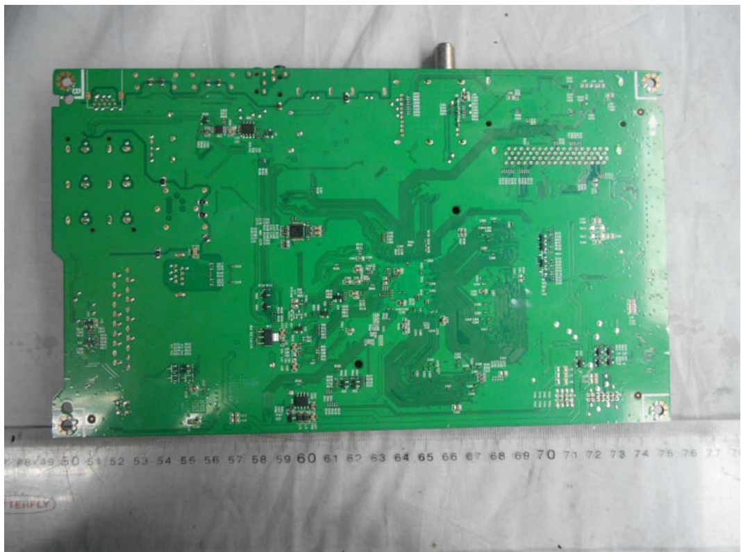
FIGURE 5 LED LCD TV (M/N: LTDN55K3201GUWUS) MAIN BOARD (SOLDERED SIDE)
