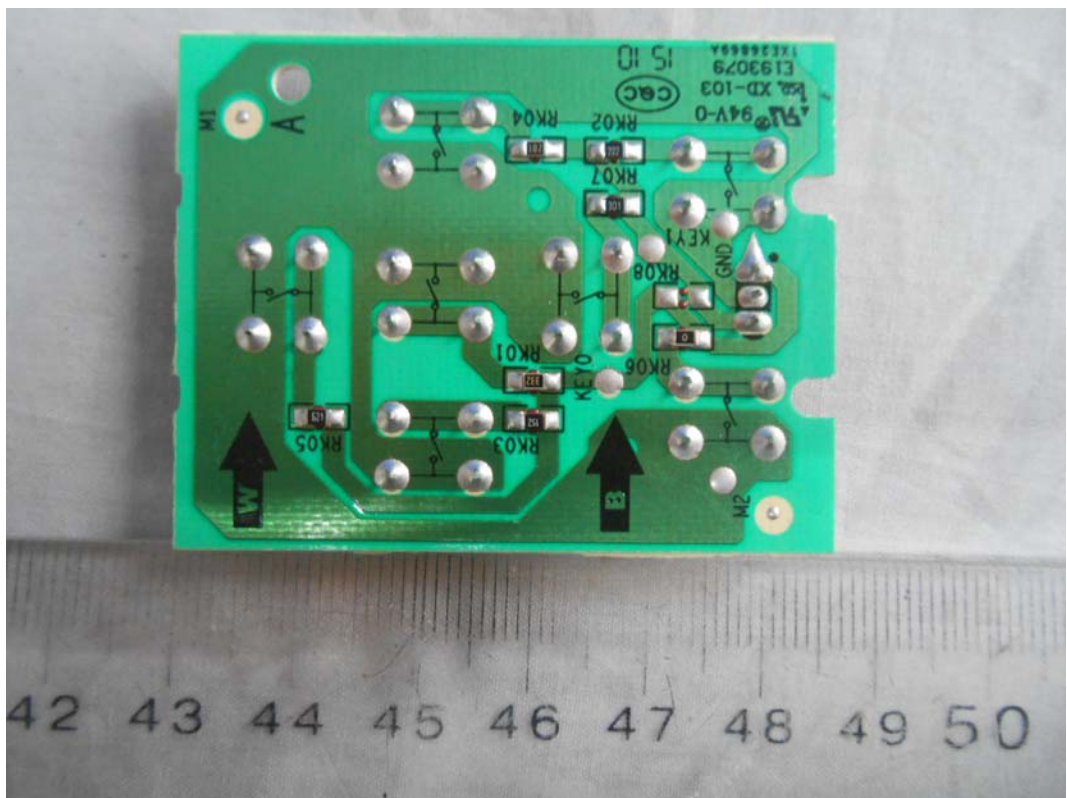
FIGURE 19 LED LCD TV (M/N: LTDN55K3201GUWUS) KEY BOARD (SOLDERED SIDE)
