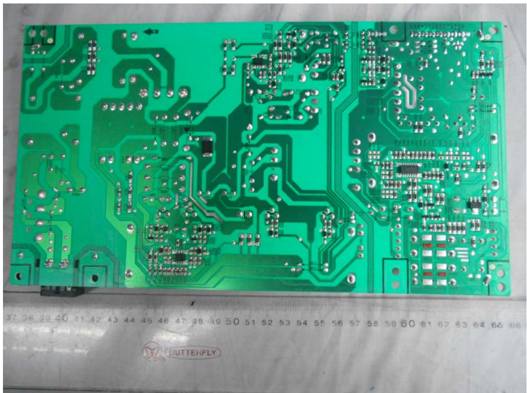
FIGURE 15 LED LCD TV (M/N: LTDN55K3201GUWUS) POWER BOARD (SOLDERED SIDE)
