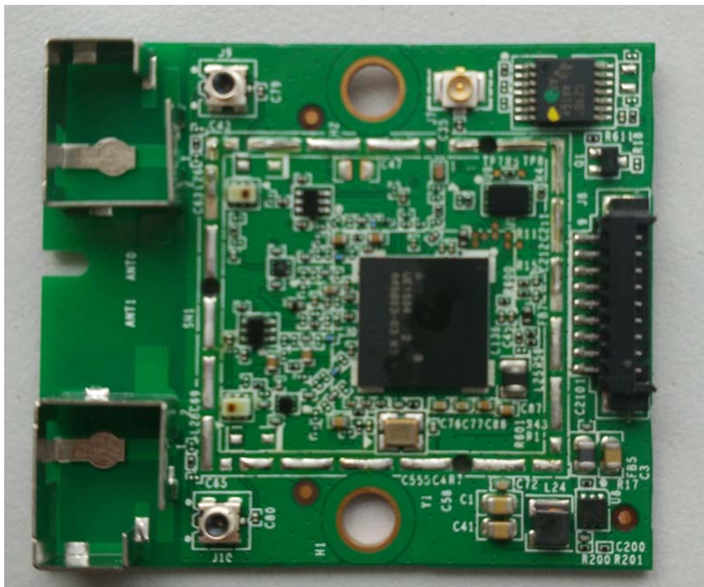
FIGURE 13 LED LCD TV (M/N: LTDN55K3201G UWUS) RF MODULE WITHOUT SHIELDING
