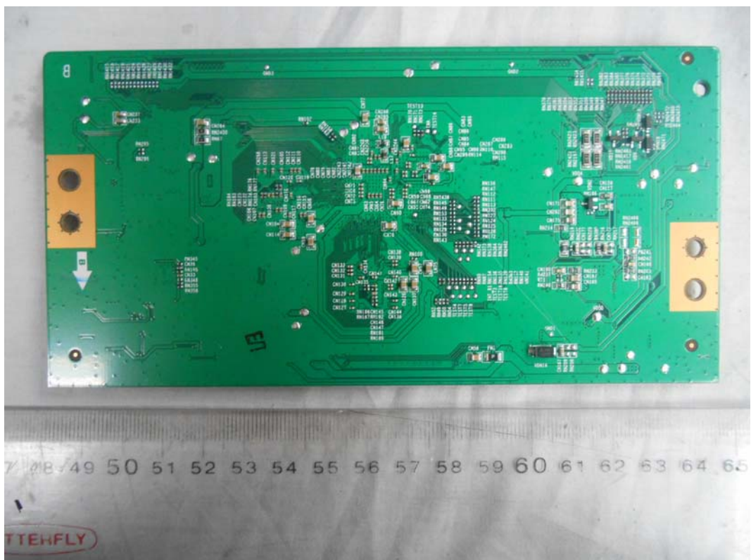
FIGURE 17 LED LCD TV (M/N: LTDN55K320IGUWUS) SIGNAL BOARD (SOLDERED SIDE)
