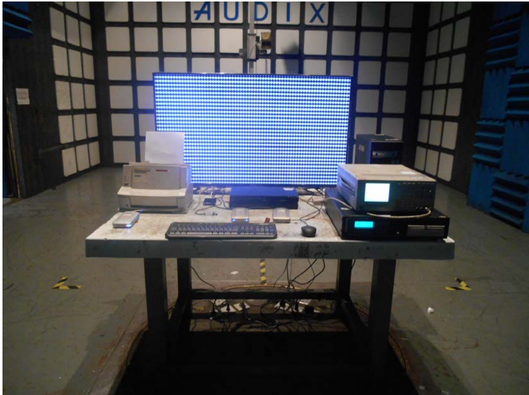
FRONT VIEW OF RADIATED EMISSION TEST (HIGH 1GHz)
