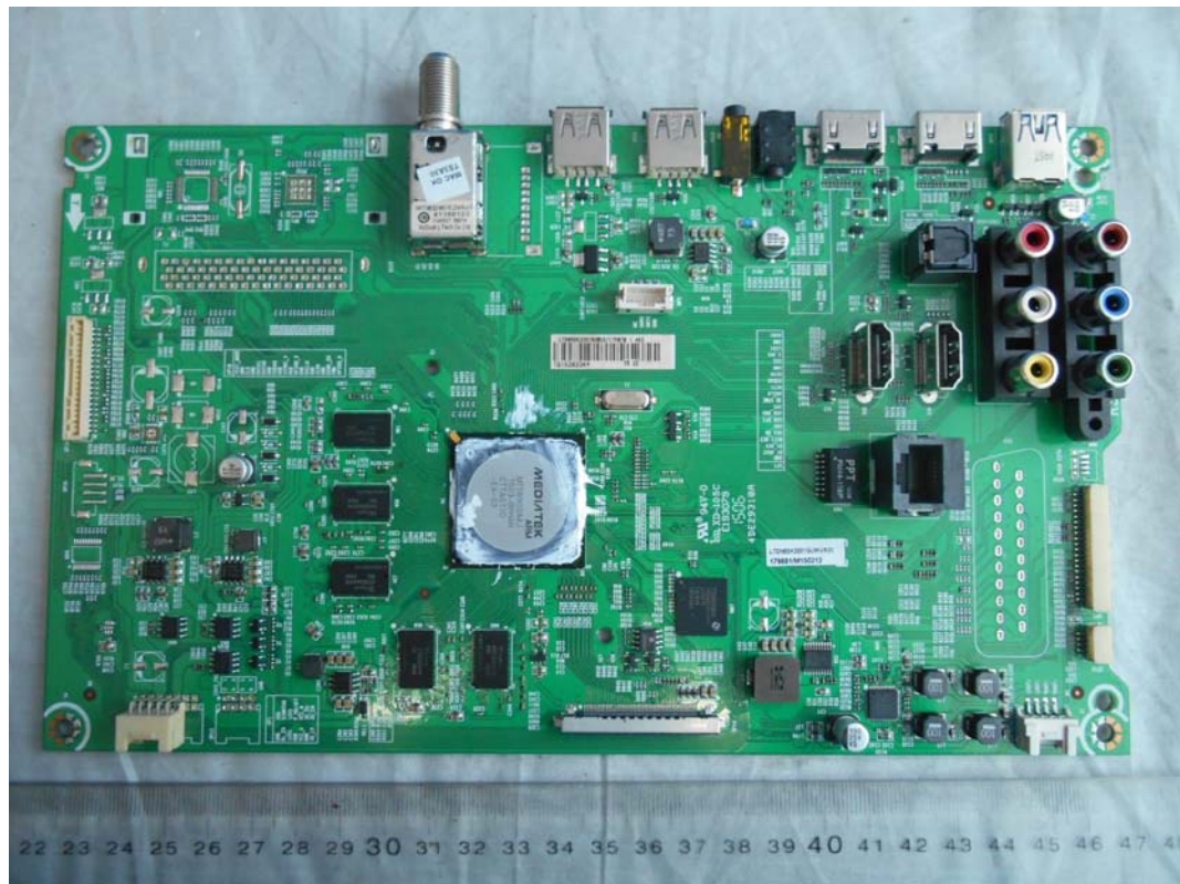
FIGURE 4 LED LCD TV (M/N: LTDN50K3201GUWUS) MAIN BOARD (COMPONENT SIDE)
