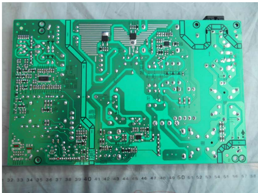
FIGURE 20 LED LCD TV (M/N: LTDN50K3201GUWUS) POWER BOARD (SOLDERED SIDE)
