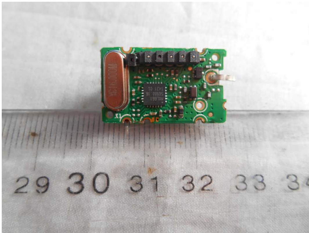
FIGURE 8 LED LCD TV (M/N: LTDN50K3201GUWUS) TUNER BOARD (COMPONENT SIDE)
