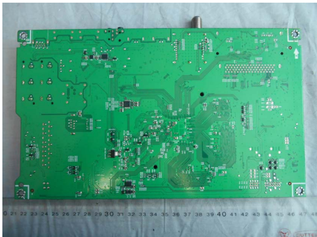
FIGURE 5 LED LCD TV (M/N: LTDN50K3201GUWUS) MAIN BOARD (SOLDERED SIDE)
