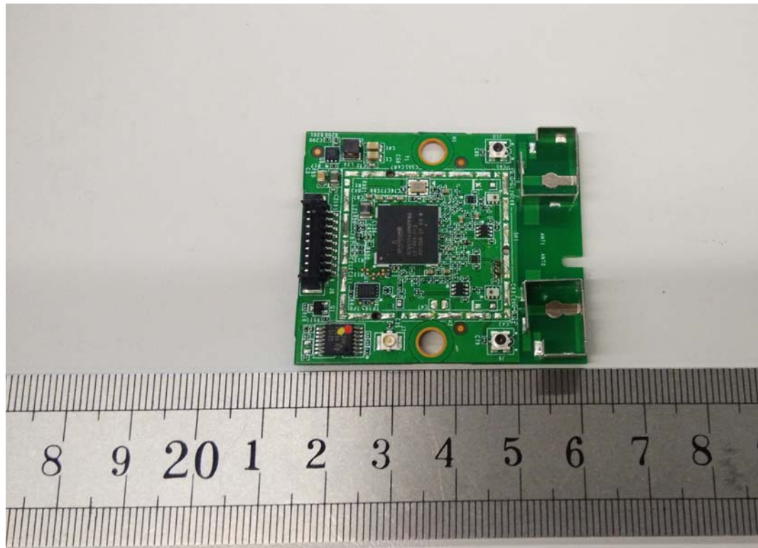
FIGURE 14 LED LCD TV (M/N: LTDN50K3201GUWUS) RF BOARD (COVER REMOVED)
