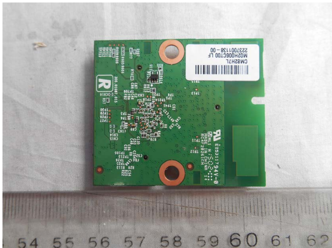
FIGURE 13 LED LCD TV (M/N: LTDN50K3201GUWUS) RF BOARD (SOLDERED SIDE)
