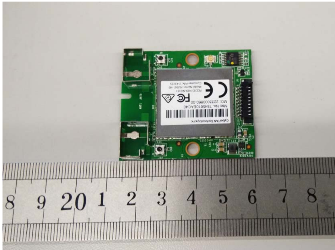
FIGURE 12 LED LCD TV (M/N: LTDN50K3201GUWUS) RF BOARD (COMPONENT SIDE)
