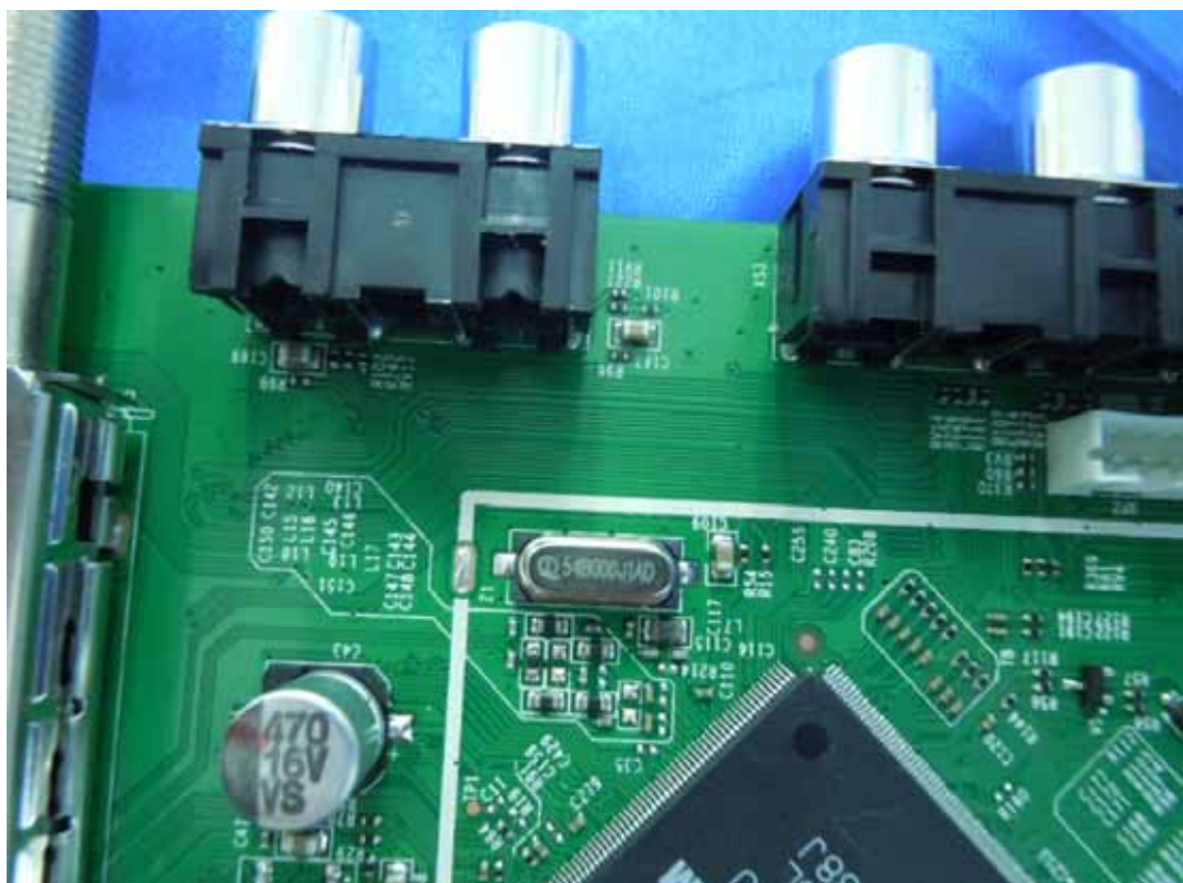
FIGURE 7 LED LCD TV (M/N: LTDN46K20US) CRYSTAL ON MAIN BOARD
