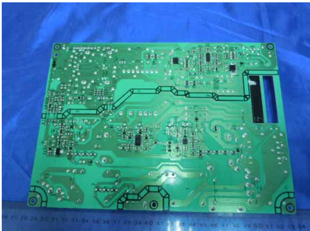
FIGURE 3 LED LCD TV (M/N: LTDN46K20US) POWER BOARD (SOLDERED SIDE)
