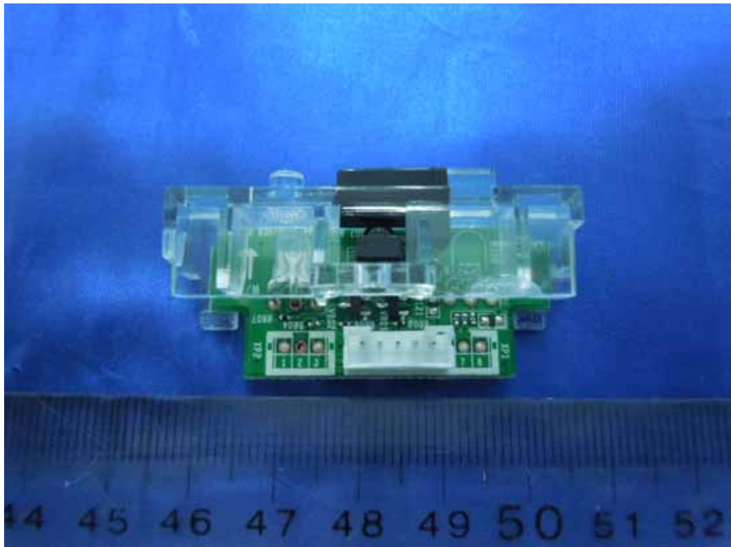
FIGURE 11 LED LCD TV (M/N: LTDN46K20US) IR BOARD (COMPONENT SIDE)
