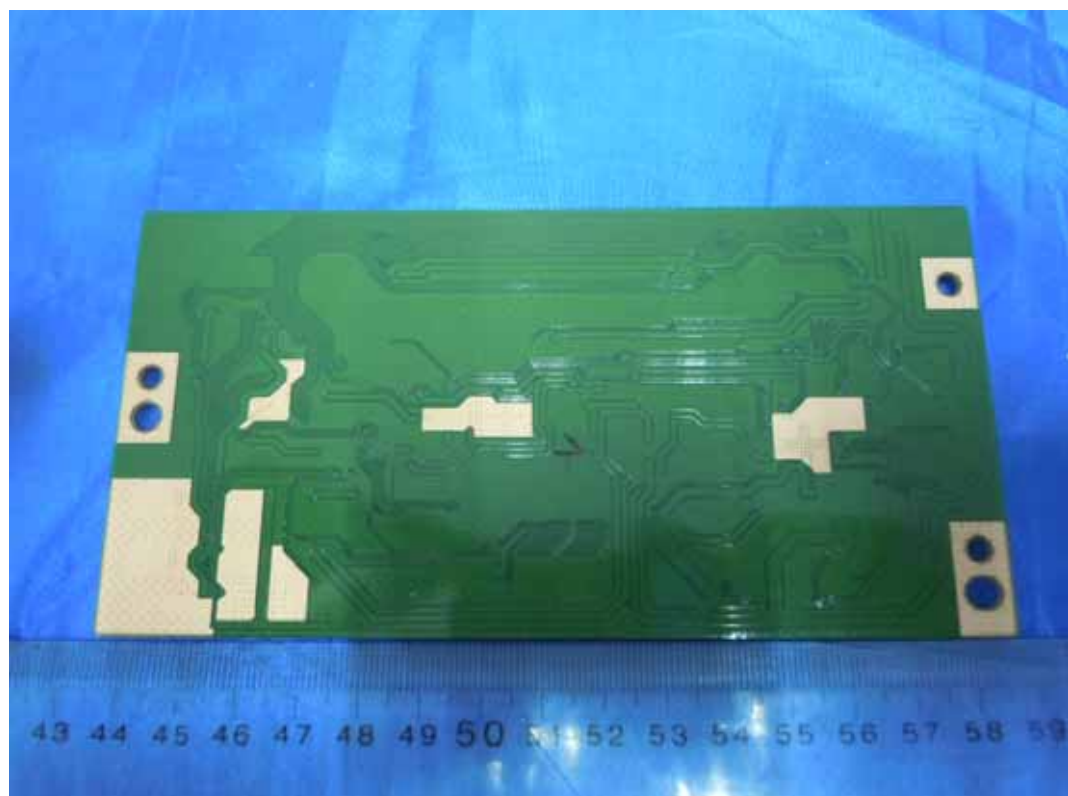
FIGURE 14 LED LCD TV (M/N: LTDN46K20US) PANEL BOARD (SOLDERED SIDE)
