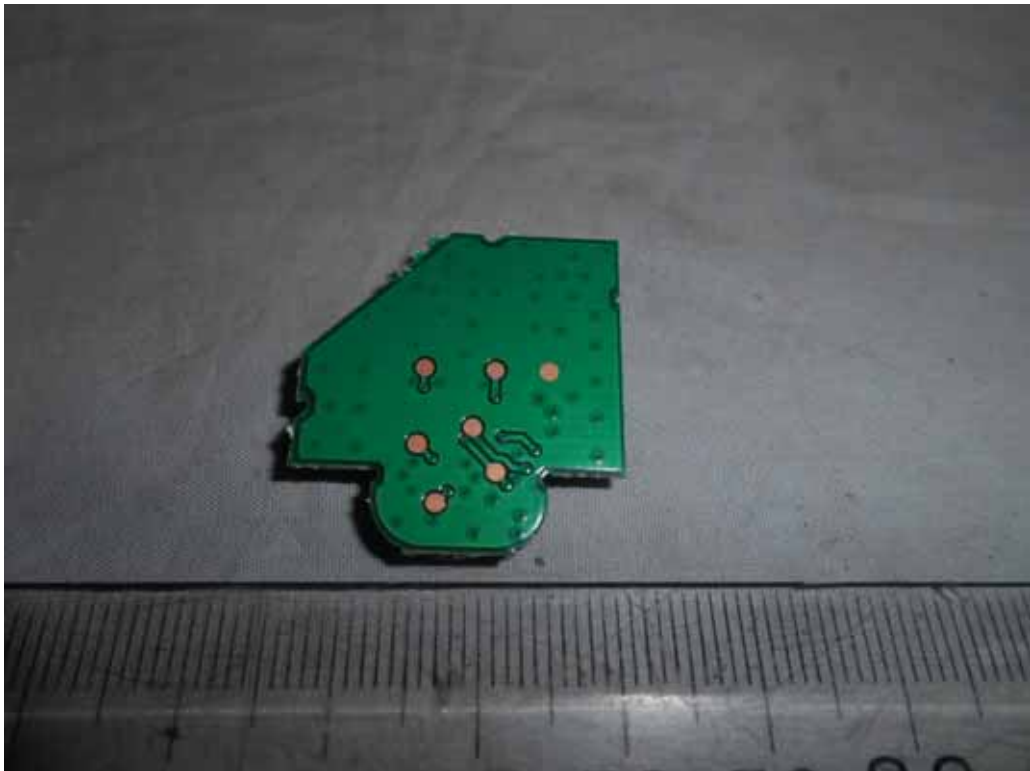
FIGURE 16 LED LCD TV (M/N: LTDN40K2207WUS) IR BOARD (SOLDERED SIDE)
