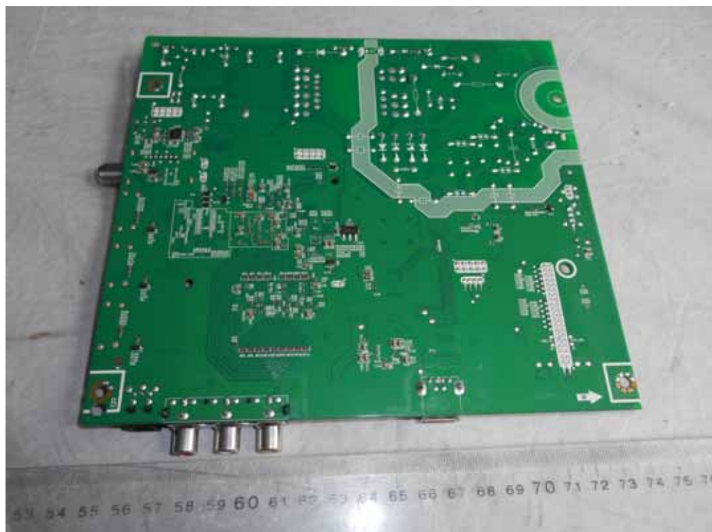
FIGURE 4 LED LCD TV (M/N: LTDN40K2207WUS) MAIN BOARD (SOLDERED SIDE)
