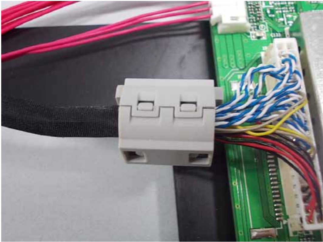
FIGURE 17 LED LCD TV (M/N: LTDN46K360US) DEBUG #1
