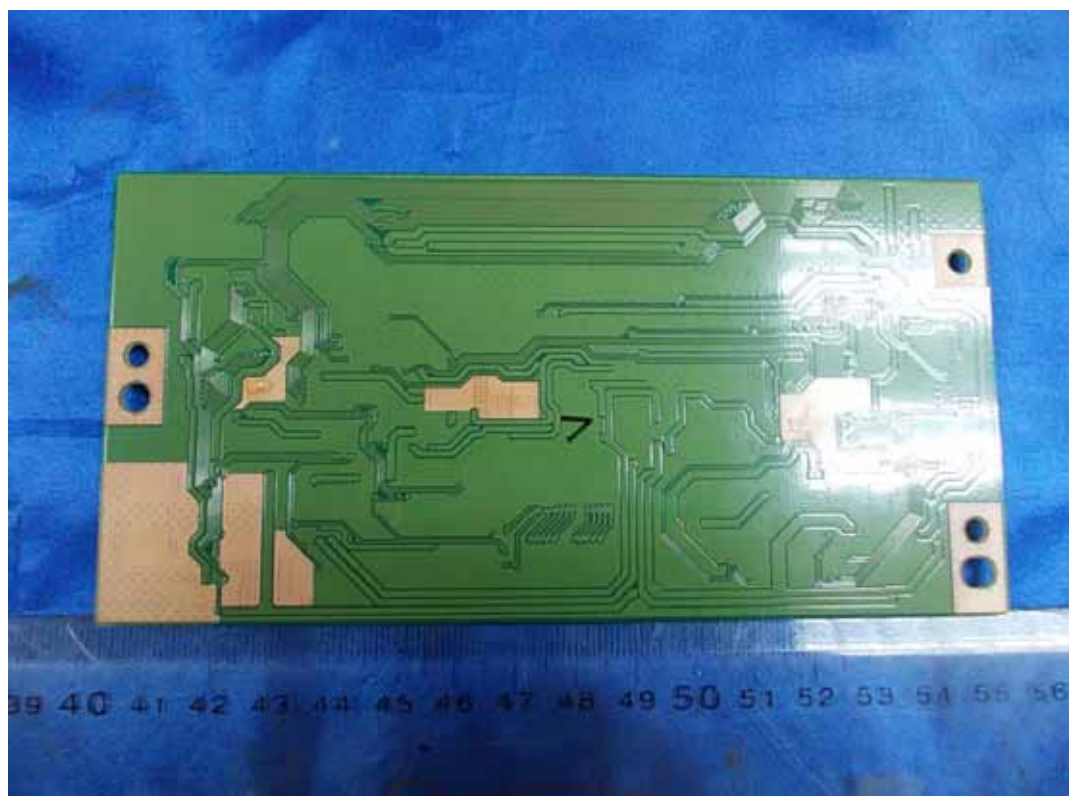
FIGURE 14 LED LCD TV (M/N: LTDN46K360US) LCD PANEL CONTROL BOARD (SOLDERED SIDE)
