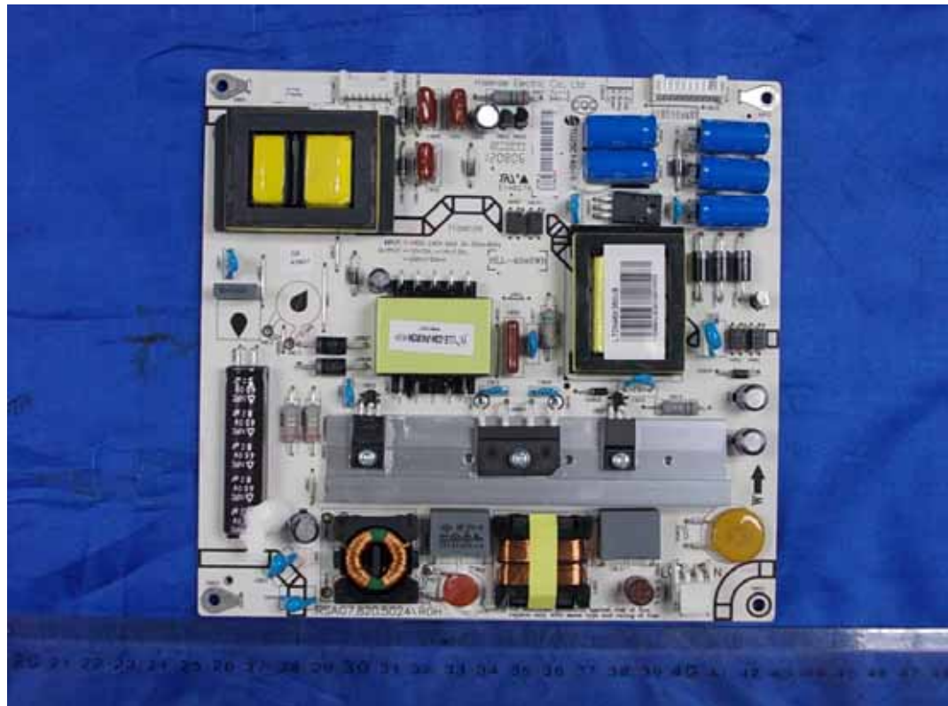
FIGURE 2 LED LCD TV (M/N: LTDN46K360US) POWER BOARD (COMPONENT SIDE)
