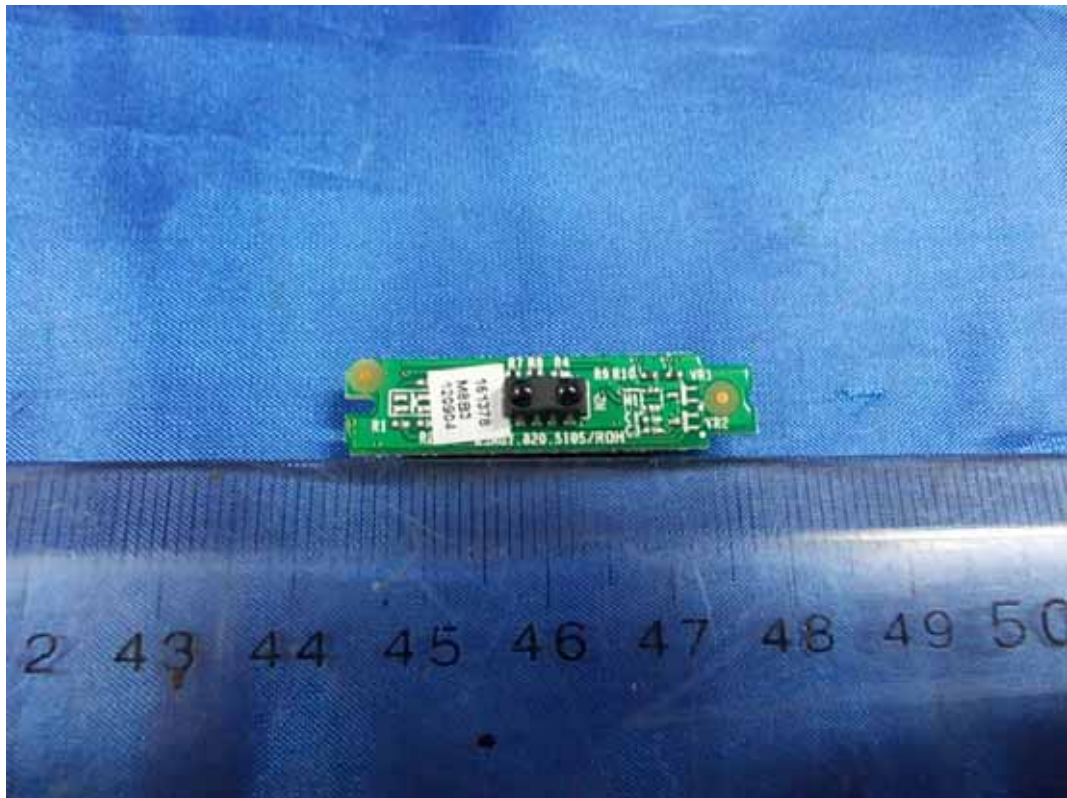
FIGURE 11 LED LCD TV (M/N: LTDN46K360US) IR BOARD (COMPONENT SIDE)
