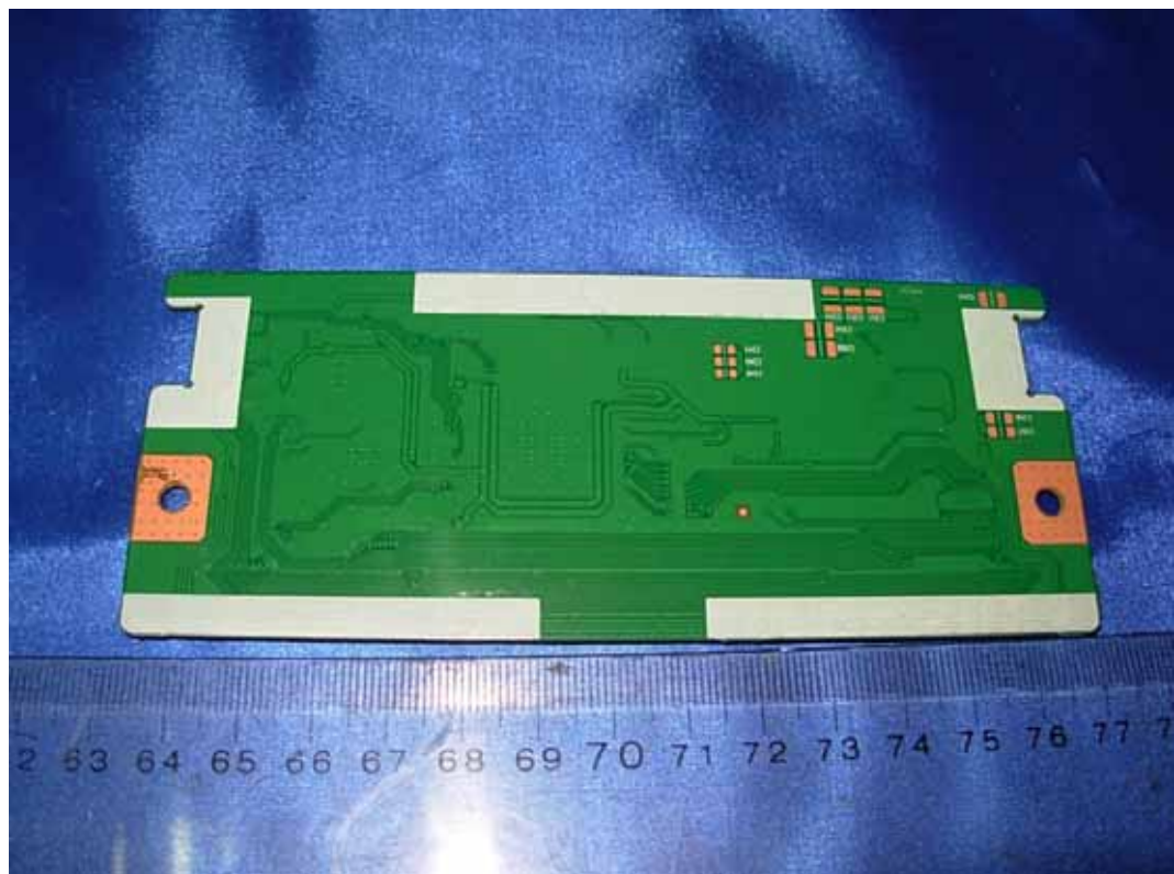
FIGURE 10 LCD TV (M/N: LTDN42V77US) CONTROL BOARD (SOLDERED SIDE)
