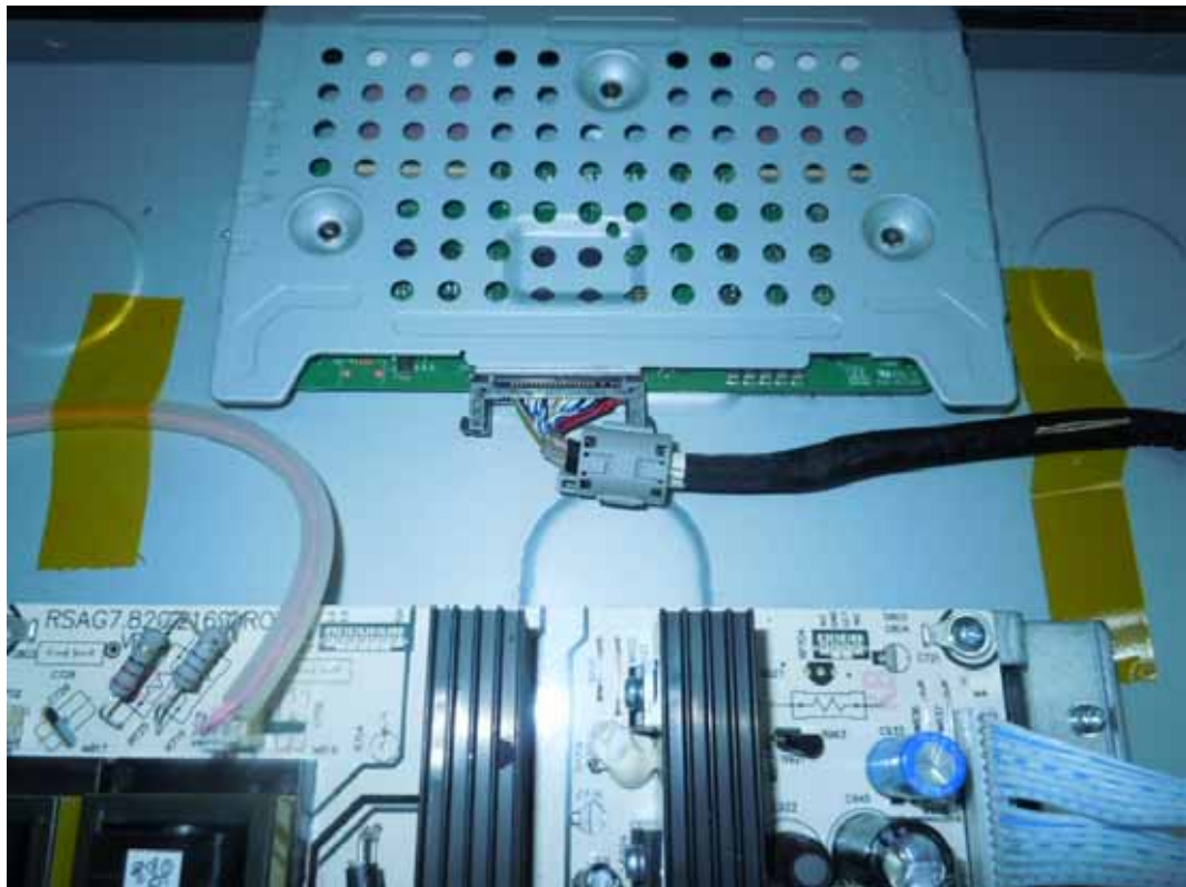
FIGURE 17 LCD TV (M/N: LTDN42V77US) DEBUG 3
