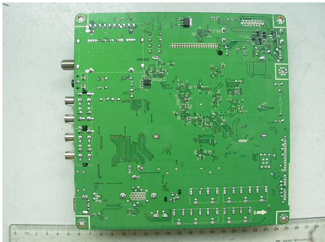
FIGURE 5 LCD TV (M/N: LTDN42V68US) MAIN BOARD (SOLDERED SIDE)
