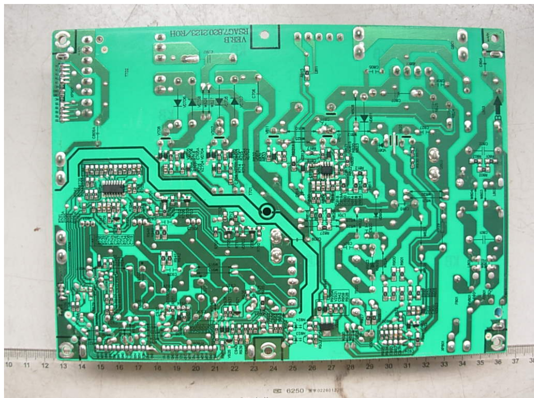
FIGURE 3 LCD TV (M/N: LTDN42V68US) POWER BOARD (SOLDERED SIDE)
