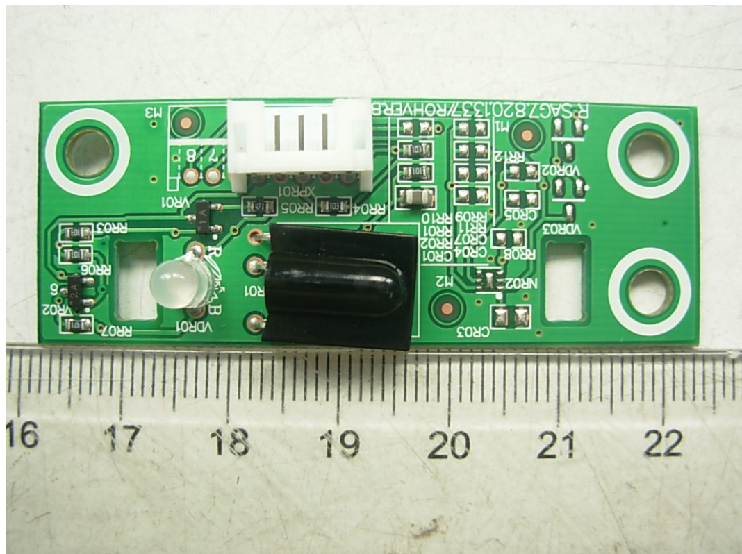
FIGURE 8 LCD TV (M/N: LTDN42V68US) IR BOARD (COMPONENT SIDE)
