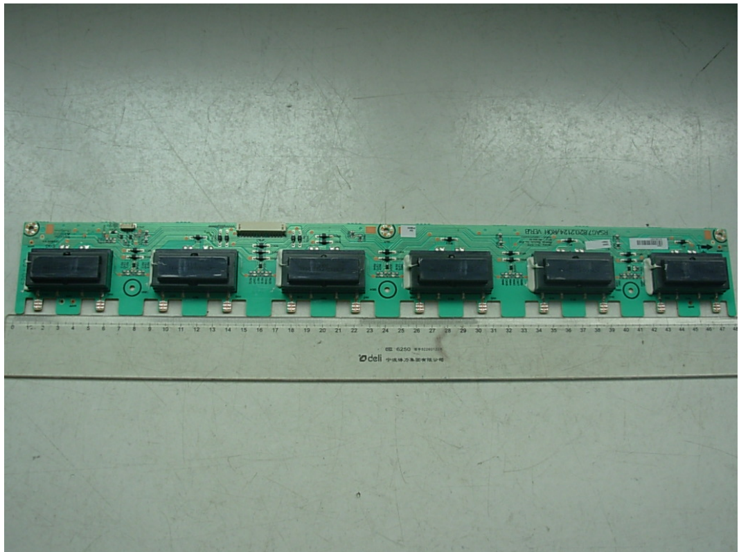
FIGURE 12 LCD TV (M/N: LTDN42V68US) HIGH VOLTAGE SIGNAL BOARD (COMPONENT SIDE)
