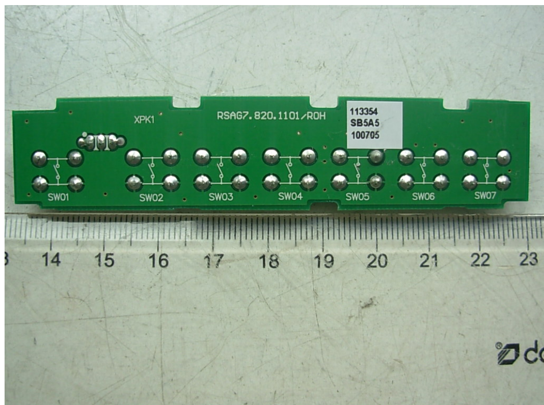
FIGURE 11 LCD TV (M/N: LTDN42V68US) KEY BOARD (SOLDERED SIDE)
