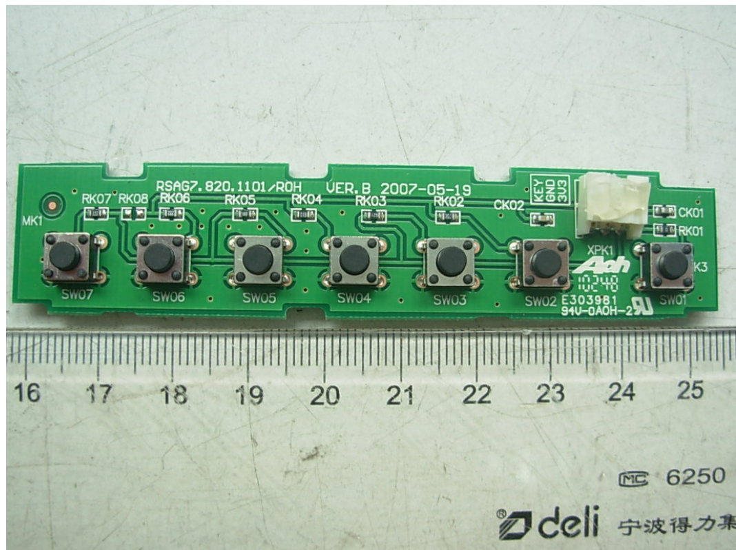
FIGURE 10 LCD TV (M/N: LTDN42V68US) KEY BOARD (COMPONENT SIDE)
