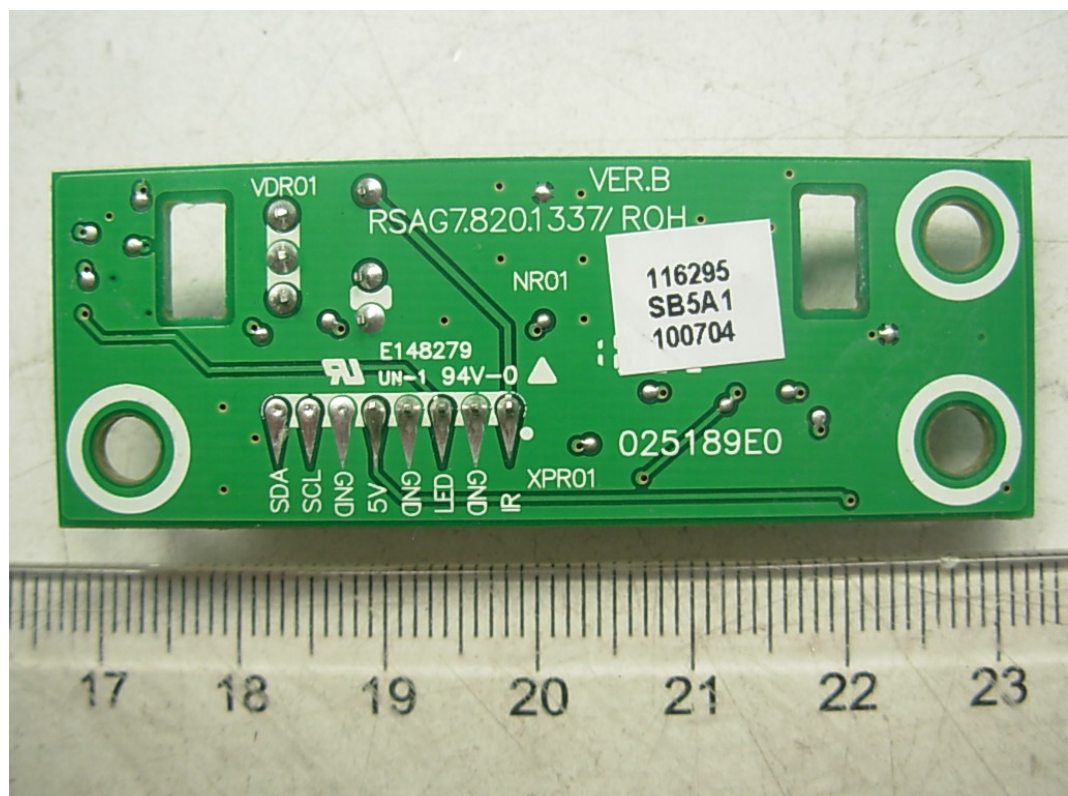
FIGURE 9 LCD TV (M/N: LTDN42V68US) IR BOARD (SOLDERED SIDE)
