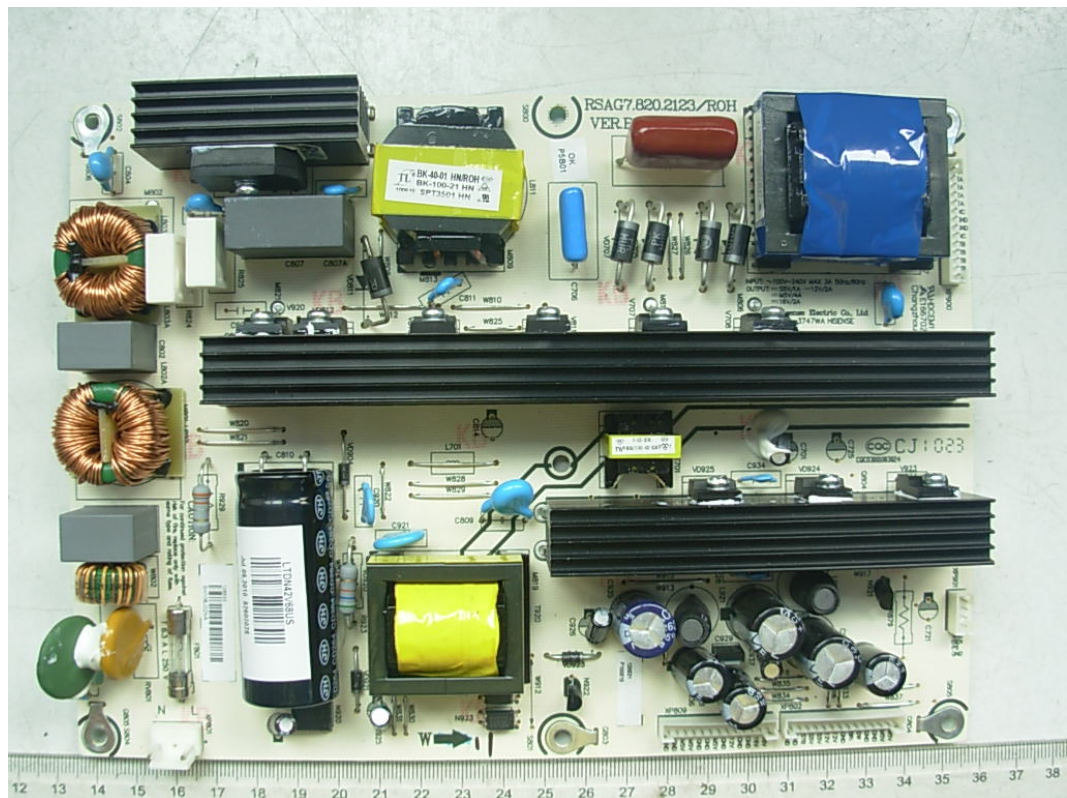
FIGURE 2 LCD TV (M/N: LTDN42V68US) POWER BOARD (COMPONENT SIDE)
