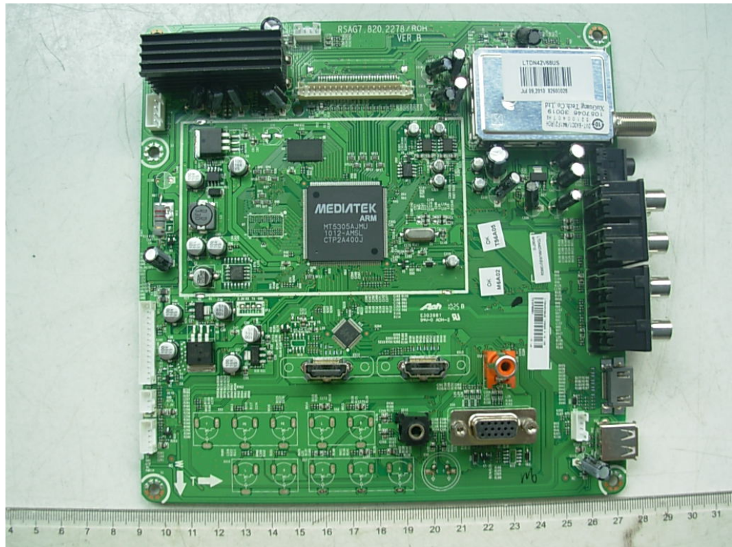
FIGURE 4 LCD TV (M/N: LTDN42V68US) MAIN BOARD (COMPONENT SIDE)
