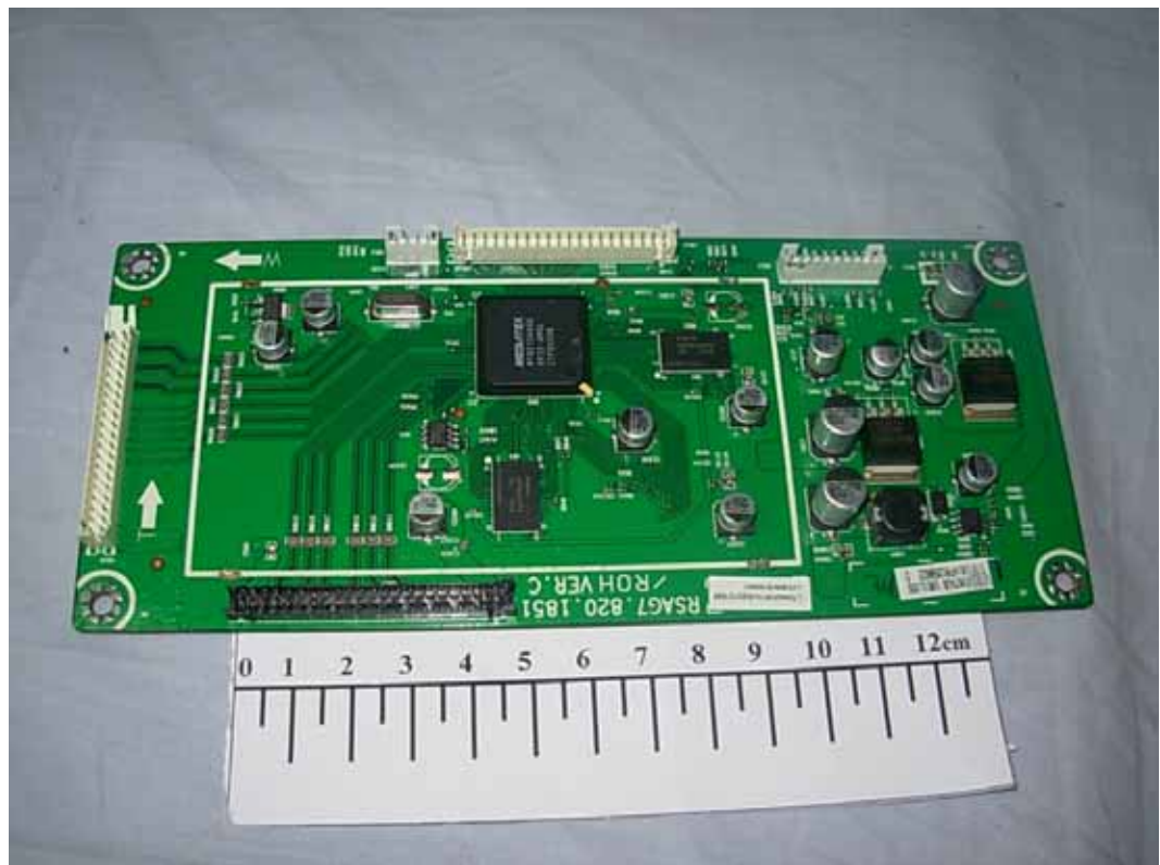
FIGURE 11 LCD TV (M/N: LTDN42V87XUS) LCD PANEL CONTROL BOARD #1 (COMPONENT SIDE)
