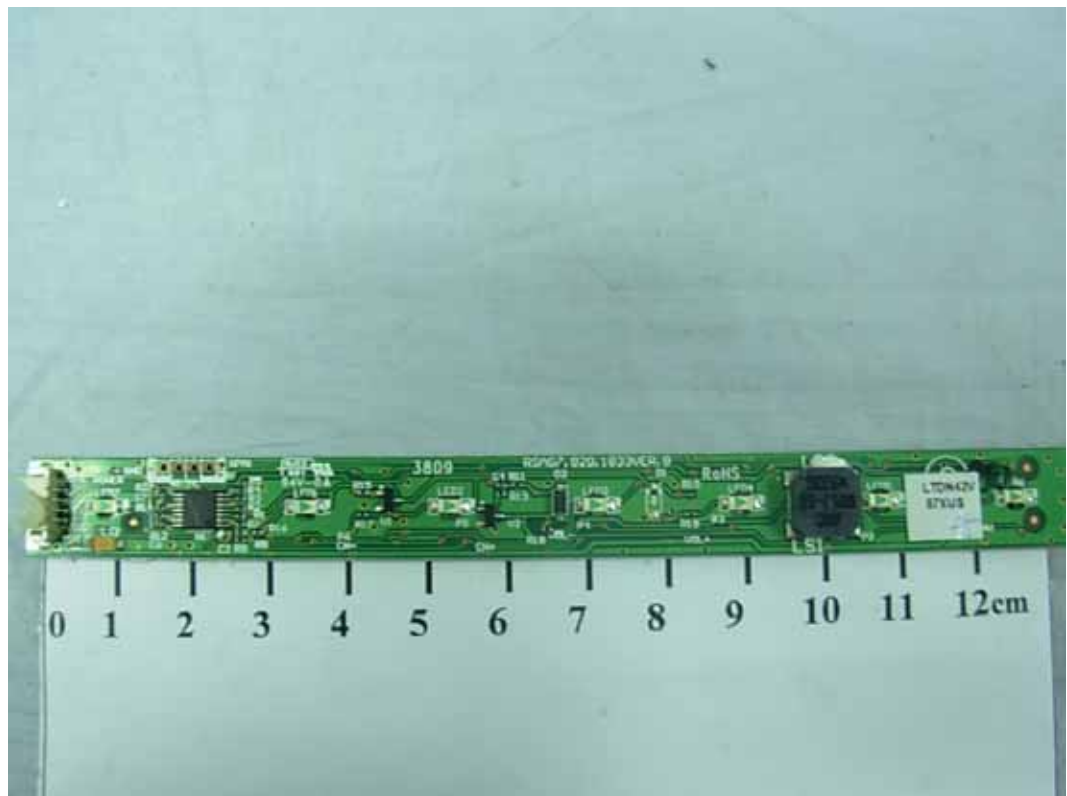
FIGURE 17 LCD TV (M/N: LTDN42V87XUS) KEY BOARD (COMPONENT SIDE)
