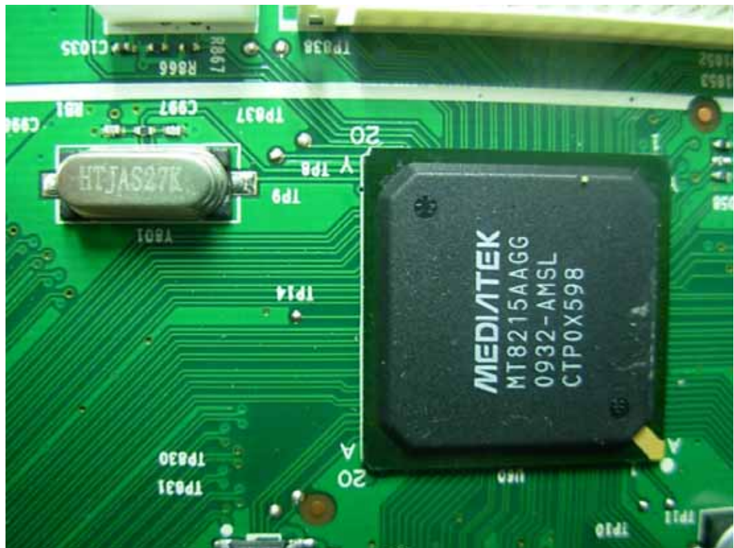
FIGURE 13 LCD TV (M/N: LTDN42V87XUS) CHIP & CRYSTAL ON LCD PANEL CONTROL BOARD #1
