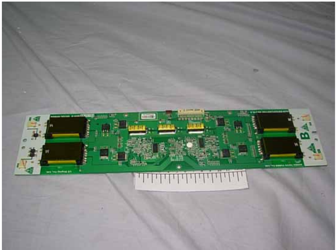
FIGURE 4 LCD TV (M/N: LTDN42V87XUS) HIGH VOLTAGE SIGNAL BOARD (COMPONENT SIDE)
