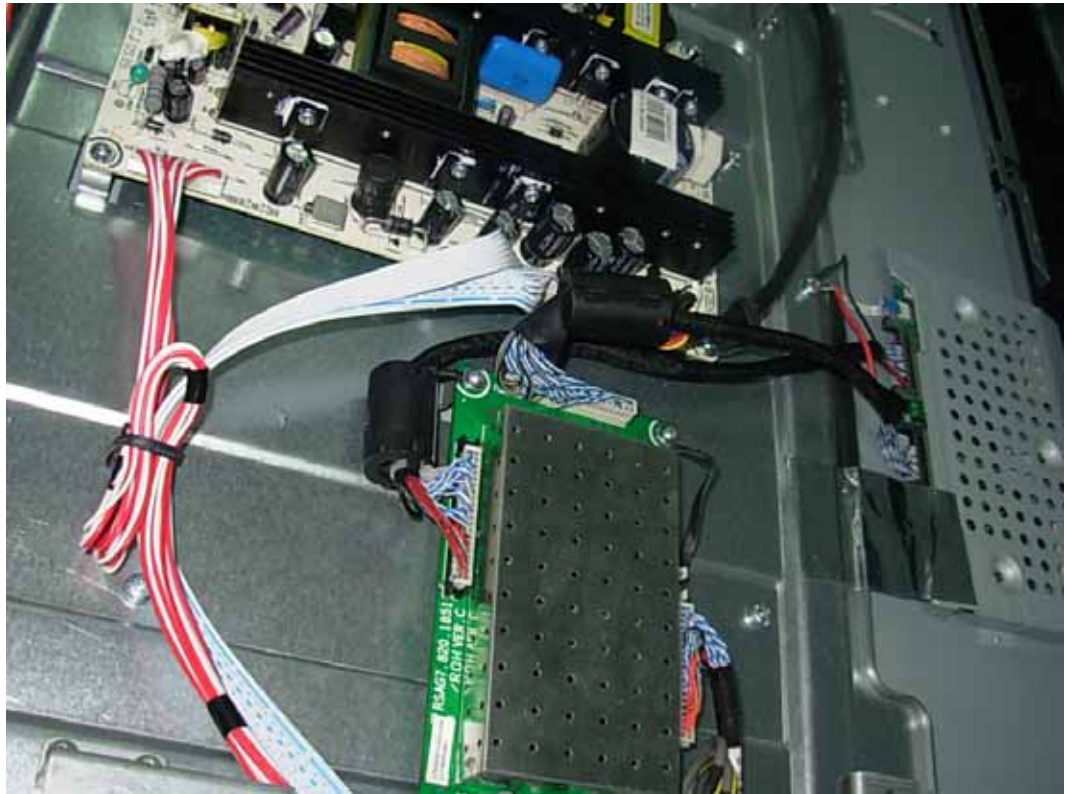
FIGURE 21 LCD TV (M/N: LTDN42V87XUS) DEBUG #1
