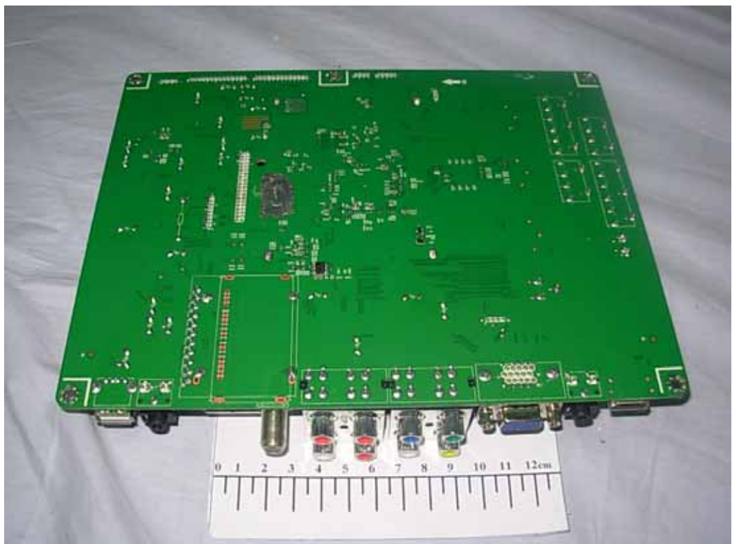
FIGURE 7 LCD TV (M/N: LTDN42V87XUS) MAIN BOARD (SOLDERED SIDE)
