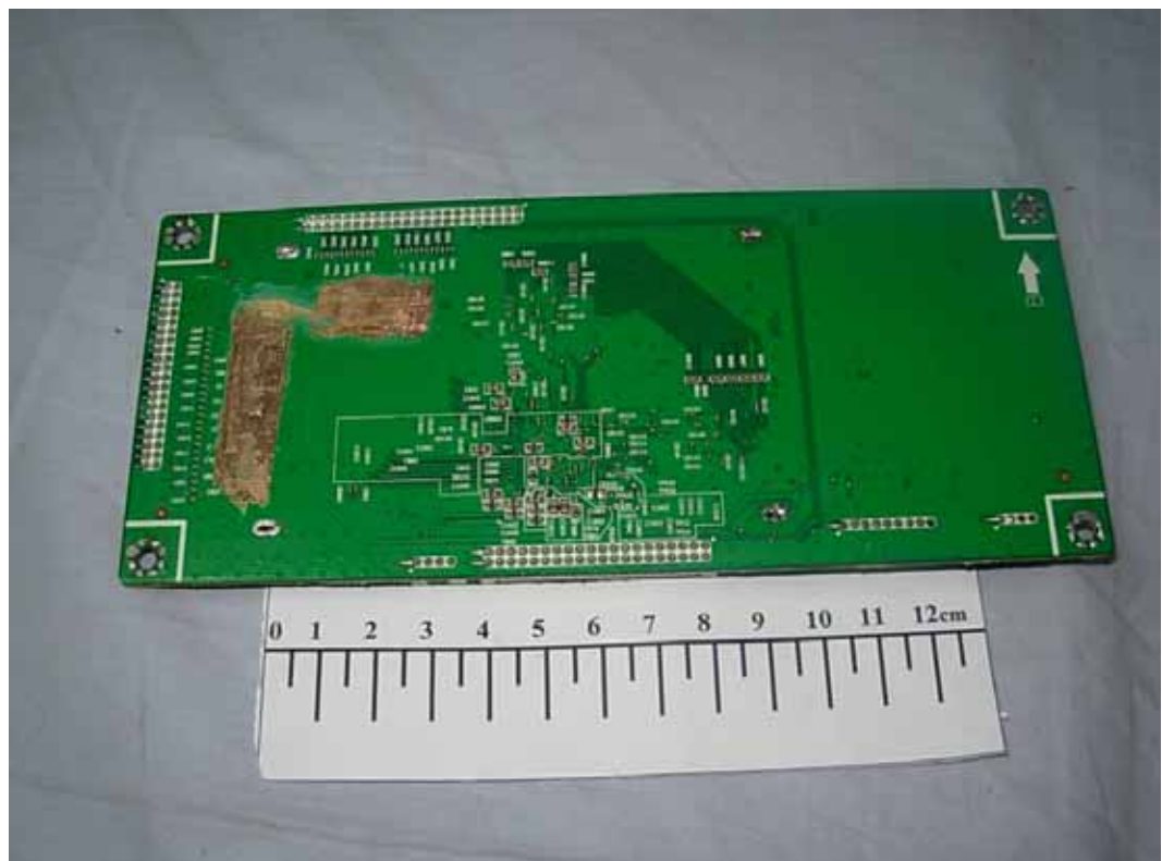
FIGURE 12 LCD TV (M/N: LTDN42V87XUS) LCD PANEL CONTROL BOARD #1 (SOLDERED SIDE)
