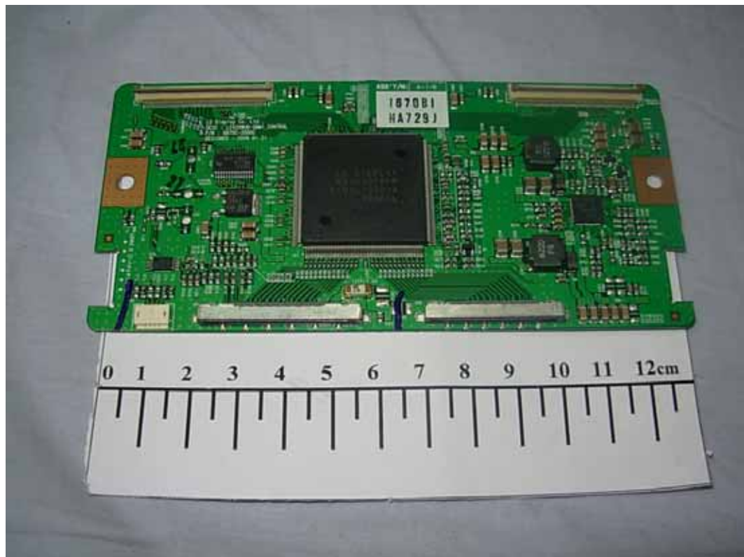
FIGURE 14 LCD TV (M/N: LTDN42V87XUS) LCD PANEL CONTROL BOARD #2 (COMPONENT SIDE)
