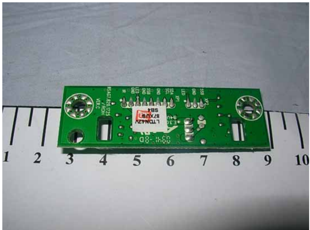
FIGURE 20 LCD TV (M/N: LTDN42V87XUS) LED BOARD (SOLDERED SIDE)
