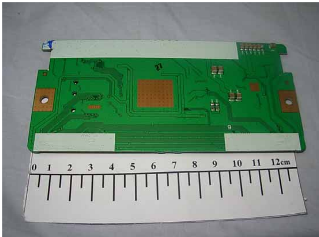
FIGURE 15 LCD TV (M/N: LTDN42V87XUS) LCD PANEL CONTROL BOARD #2 (SOLDERED SIDE)
