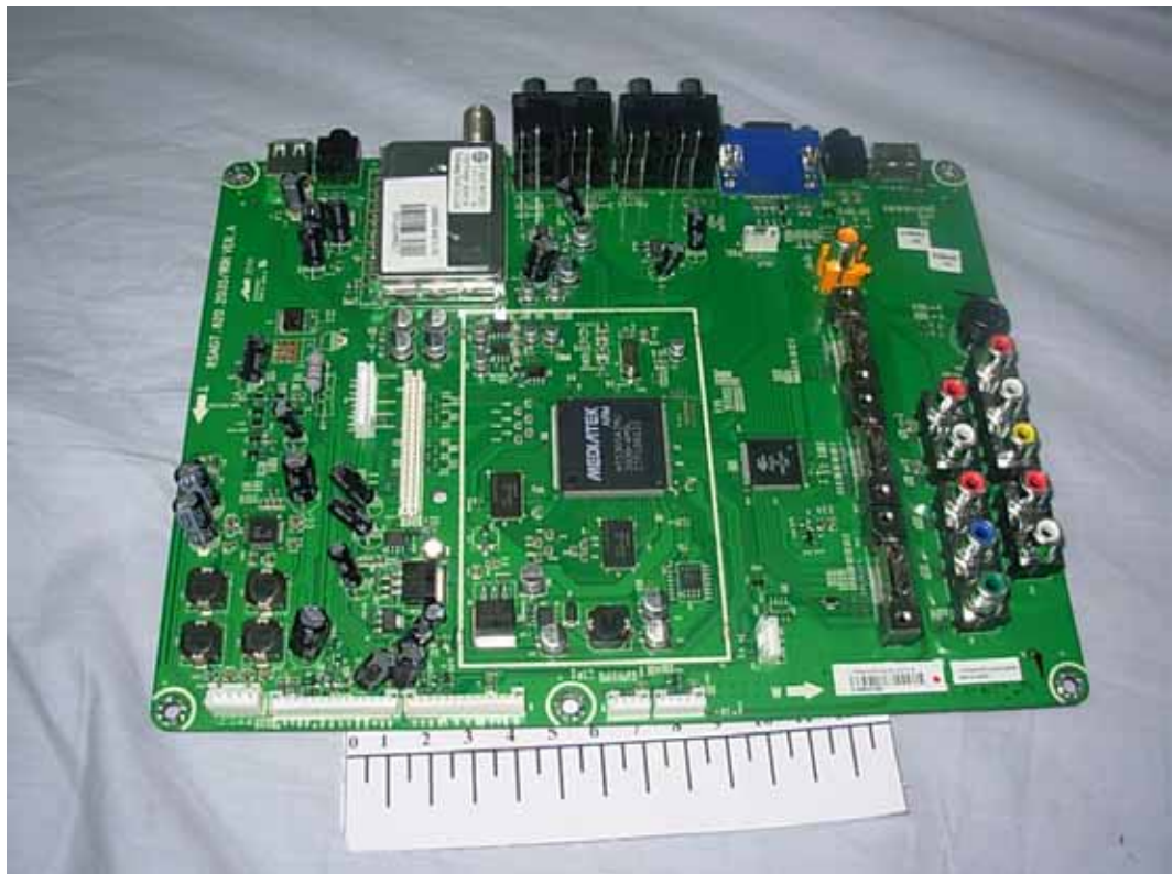
FIGURE 6 LCD TV (M/N: LTDN42V87XUS) MAIN BOARD (COMPONENT SIDE)
