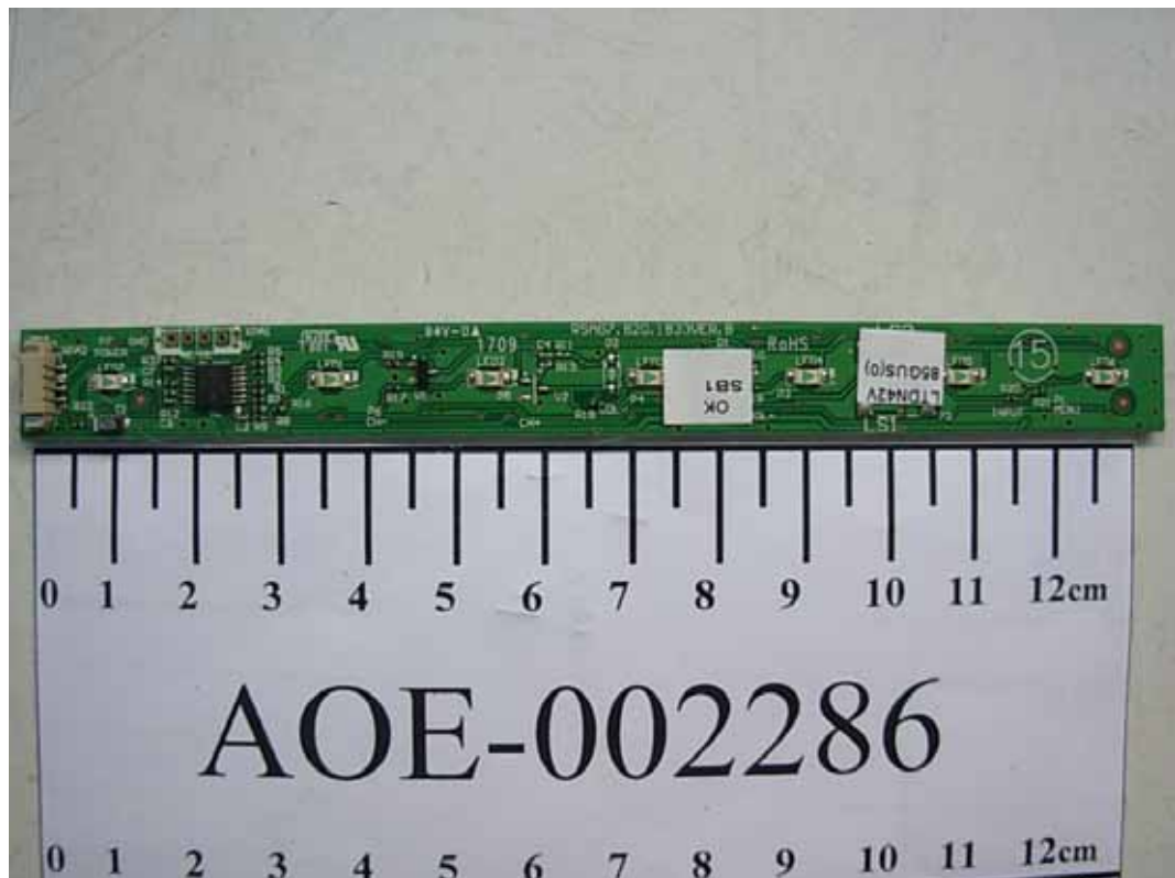
FIGURE 11 LCD TV (M/N: LTDN42V85GUS) BUTTON BOARD (COMPONENT SIDE)
