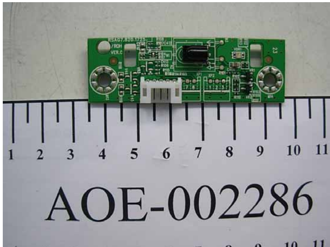
FIGURE 9 LCD TV (M/N: LTDN42V85GUS) LED BOARD (COMPONENT SIDE)
