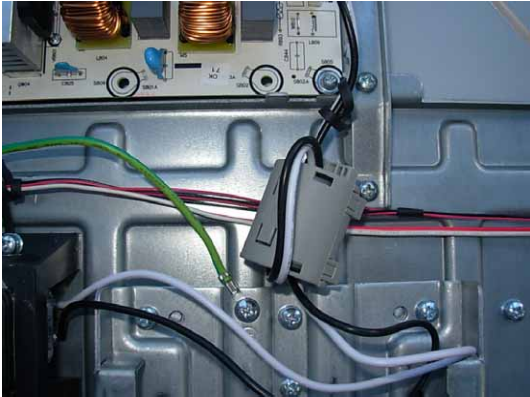
FIGURE 19 LCD TV (M/N: LTDN42V85GUS) DEBUG #4
