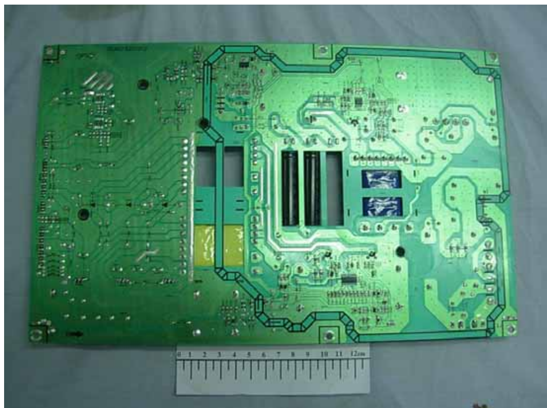
FIGURE 10 LCD TV (M/N: LTDN42T18GUS) POWER BOARD (SOLDERED SIDE)
