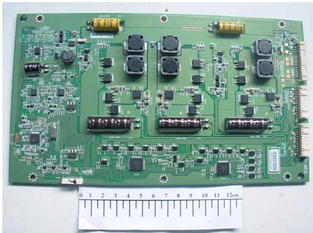
FIGURE 6 LCD TV (M/N: LTDN42T18GUS) INVERTER (COMPONENT SIDE)
