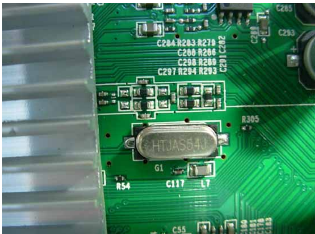
FIGURE 5 LCD TV (M/N: LTDN42T18GUS) CRYSTAL ON MAIN BOARD
