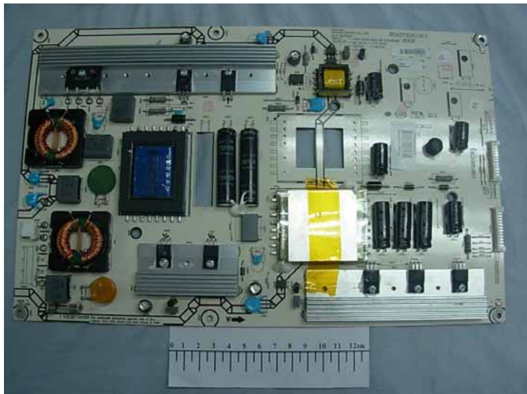
FIGURE 9 LCD TV (M/N: LTDN42T18GUS) POWER BOARD (COMPONENT SIDE)
