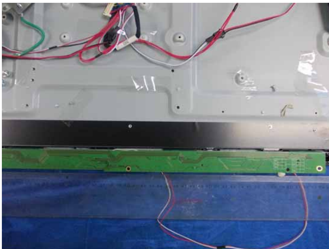
FIGURE 17 LED LCD TV (M/N: LHD32K366HS) LCD PANEL CONTROL BOARD (SOLDERED SIDE #2)
