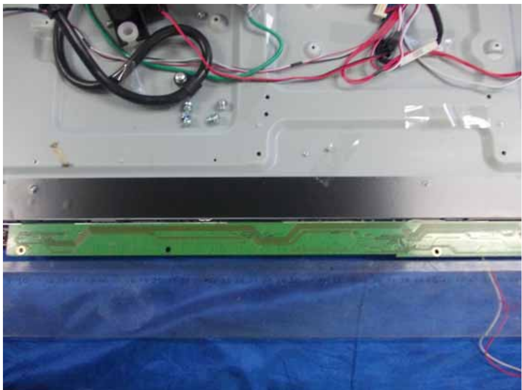
FIGURE 16 LED LCD TV (M/N: LHD32K366HS) LCD PANEL CONTROL BOARD (SOLDERED SIDE #1)
