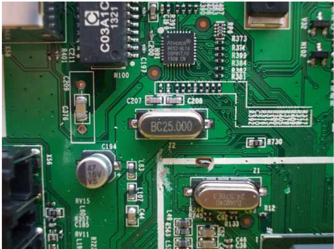
FIGURE 9 LED LCD TV (M/N: LHD32K366HS) CRYSTAL ON MAIN BOARD
