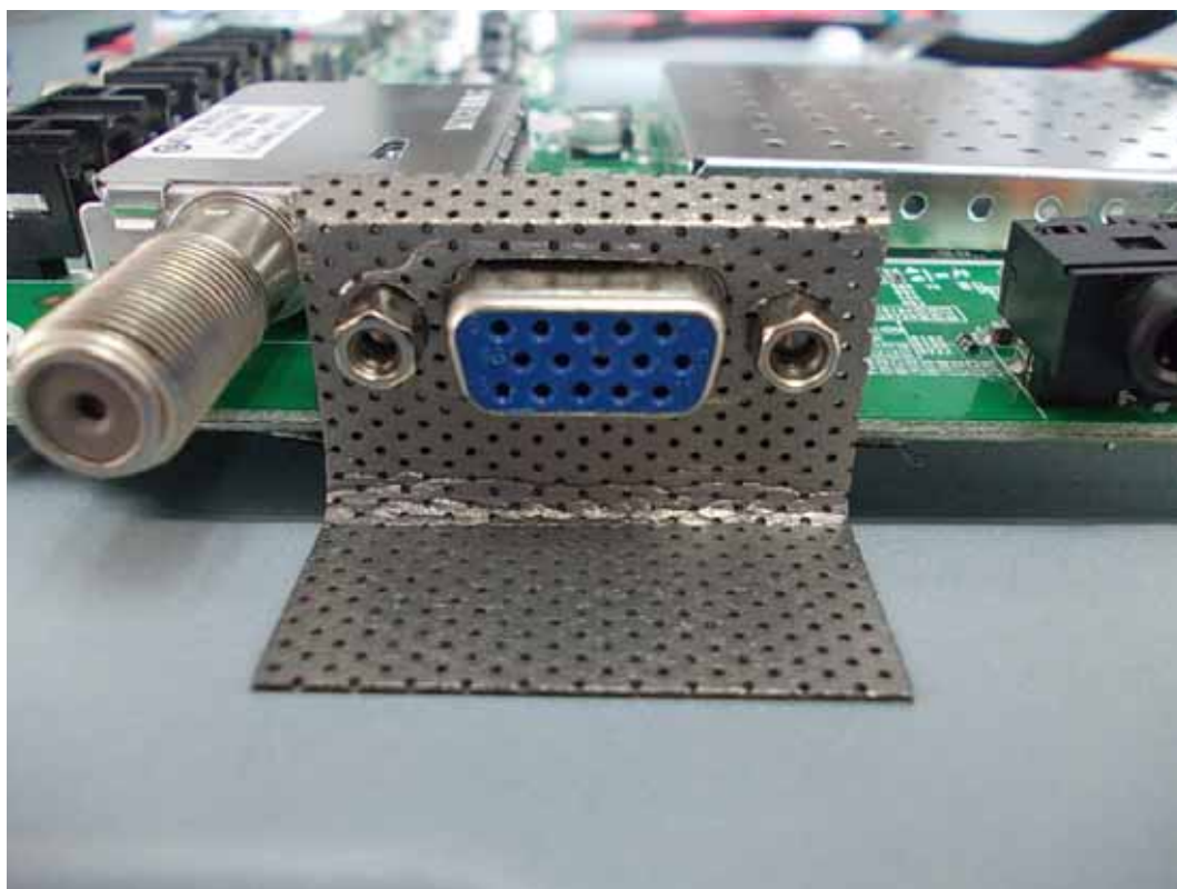
FIGURE 13 LED LCD TV (M/N: 32K360) DEBUG
