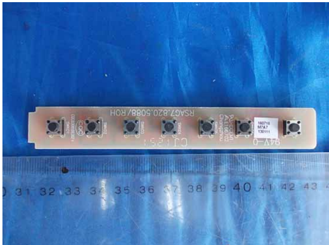
FIGURE 9 LED LCD TV (M/N: 32K360) KEY BOARD (COMPONENT SIDE)
