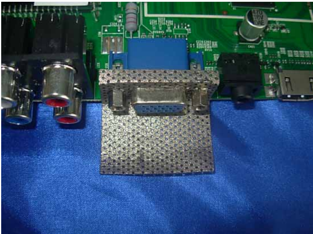
FIGURE 18 LCD TV (M/N: LHD32V77MH) DEBUG 4
