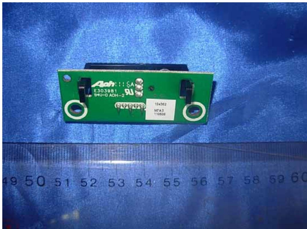
FIGURE 14 LCD TV (M/N: LHD32V77MH) IR BOARD (SOLDERED SIDE)
