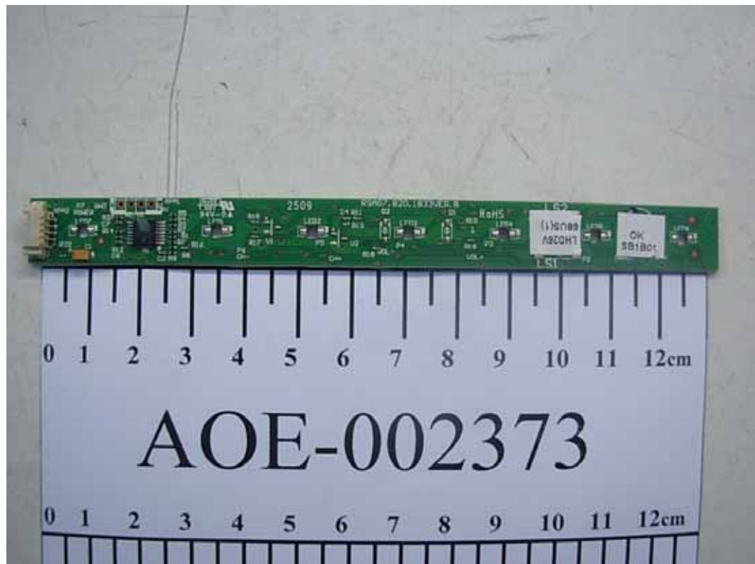
FIGURE 11 LCD TV (M/N: ELCHS262) BUTTON BOARD (COMPONENT SIDE)
