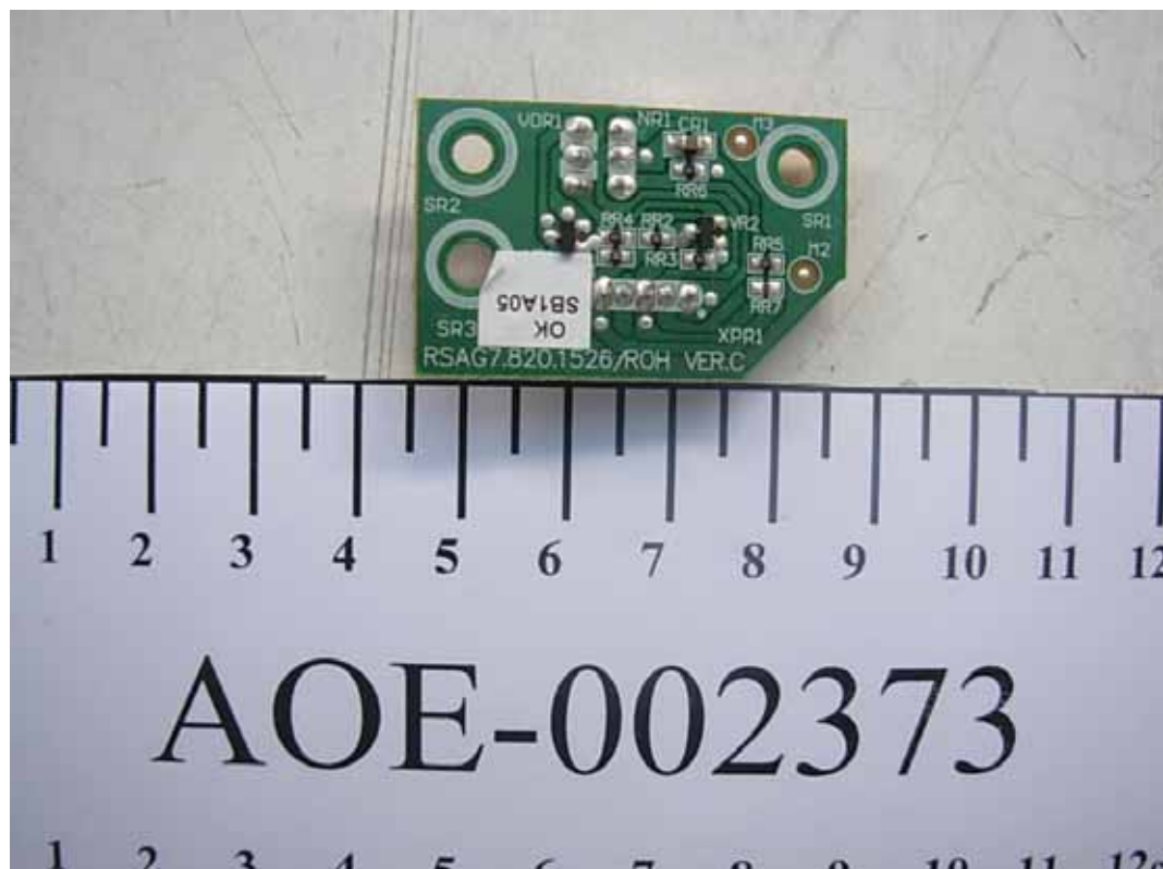
FIGURE 10 LCD TV (M/N: ELCHS262) LED BOARD (SOLDERED SIDE)
