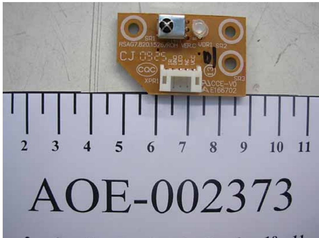
FIGURE 9 LCD TV (M/N: ELCHS262) LED BOARD (COMPONENT SIDE)
