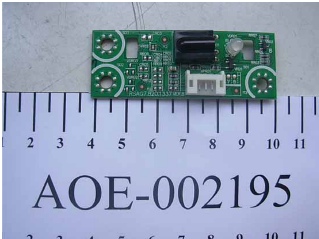
FIGURE 9 LCD TV (M/N: LHD32W57US) LED BOARD (COMPONENT SIDE)
