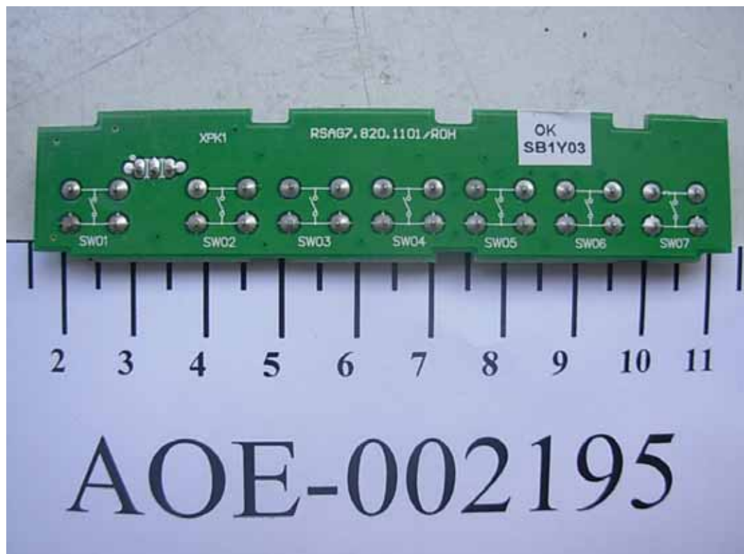
FIGURE 12 LCD TV (M/N: LHD32W57US) BUTTON BOARD (SOLDERED SIDE)
