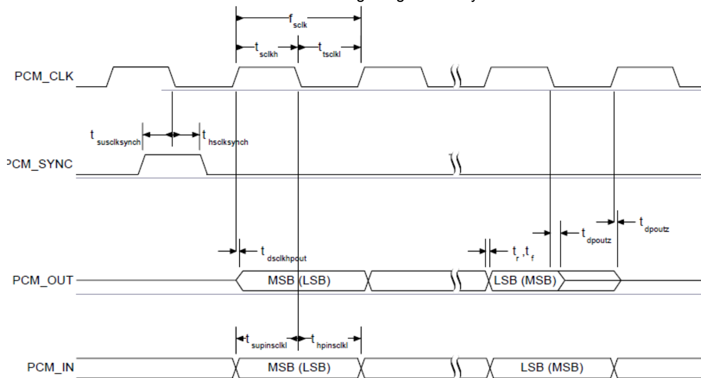
PCM Slave Timing Long Frame Sync
