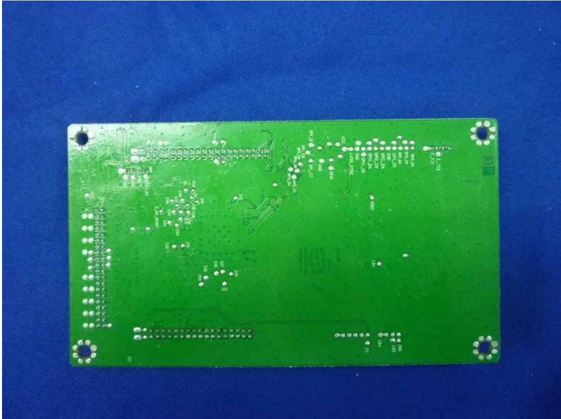
Figure 31 Backside of the PCB
