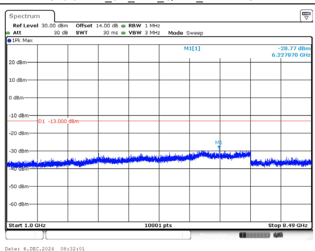
836.5 MHz_5M_1RB_QPSK_Above 1GHz
