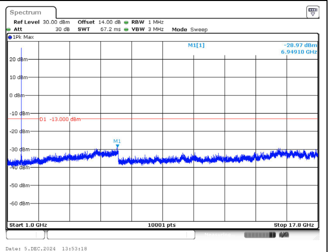
1745.0 MHz_15M_1RB_QPSK_Above 1GHz
