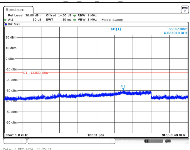
836.5 MHz_3M_1RB_QPSK_Above 1GHz
