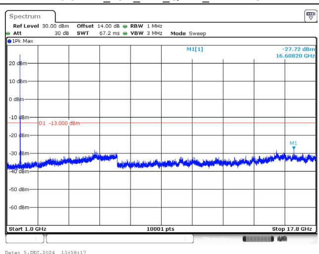
1745.0 MHz_20M_1RB_QPSK_Above 1GHz
