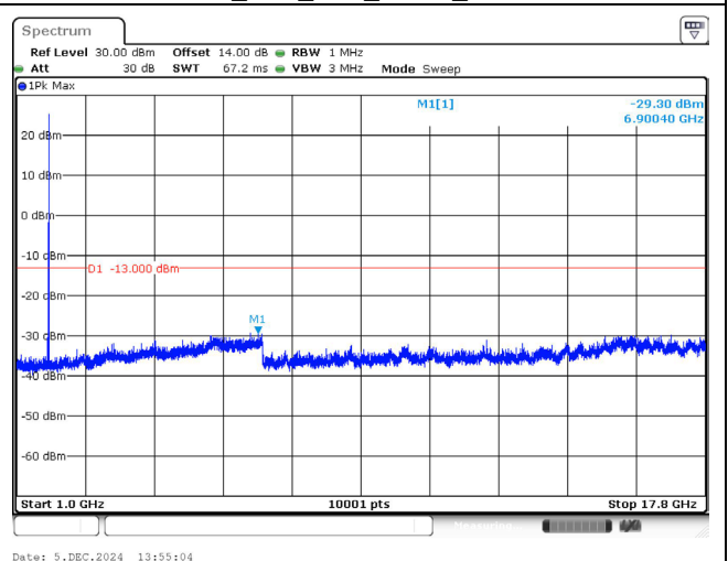
1772.5 MHz_15M_1RB_QPSK_Above 1GHz
