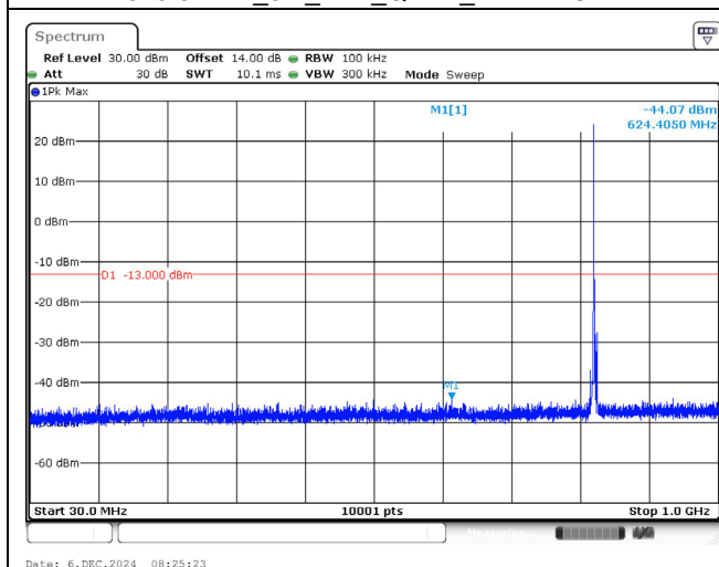
836.5 MHz_3M_1RB_QPSK_Below 1GHz
