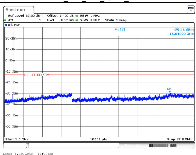
1770.0 MHz_20M_1RB_QPSK_Above 1GHz
