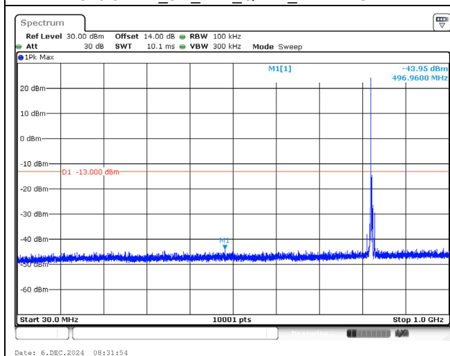
836.5 MHz_5M_1RB_QPSK_Below 1GHz
