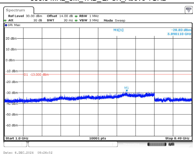
847.5 MHz_3M_1RB_QPSK_Above 1GHz
