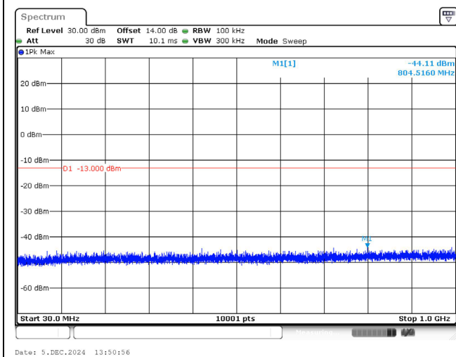
1745.0 MHz_15M_1RB_QPSK_Below 1GHz
