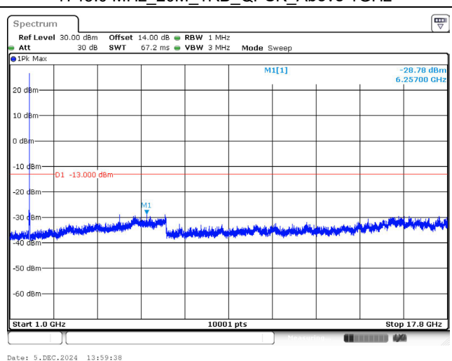
1770.0 MHz_20M_1RB_QPSK_Above 1GHz
