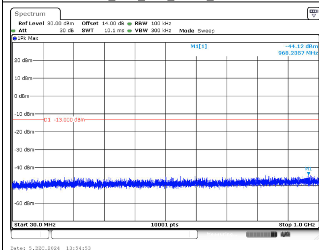
1772.5 MHz_15M_1RB_QPSK_Below 1GHz
