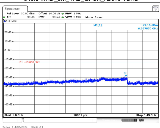
846.5 MHz_5M_1RB_QPSK_Above 1GHz
