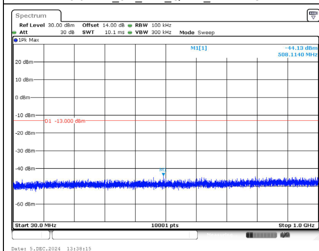
1745.0 MHz_5M_1RB_QPSK_Below 1GHz
