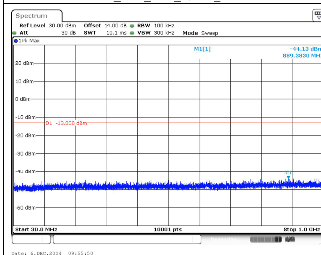
1900.0 MHz_20M_1RB_QPSK_Below 1GHz
