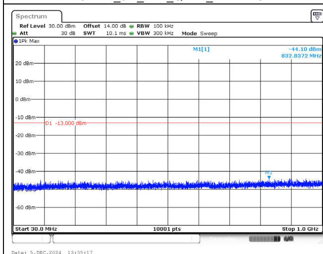
1712.5 MHz_5M_1RB_QPSK_Below 1GHz
