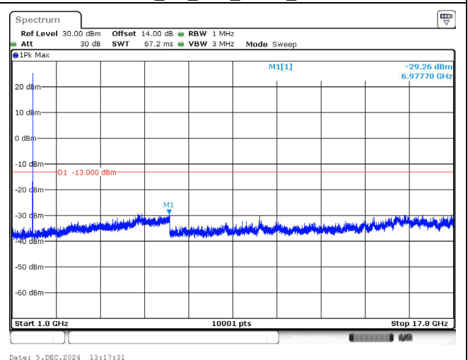
1778.5 MHz_3M_1RB_QPSK_Above 1GHz
