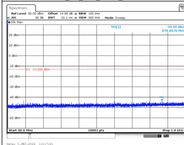
1778.5 MHz_3M_1RB_QPSK_Below 1GHz
