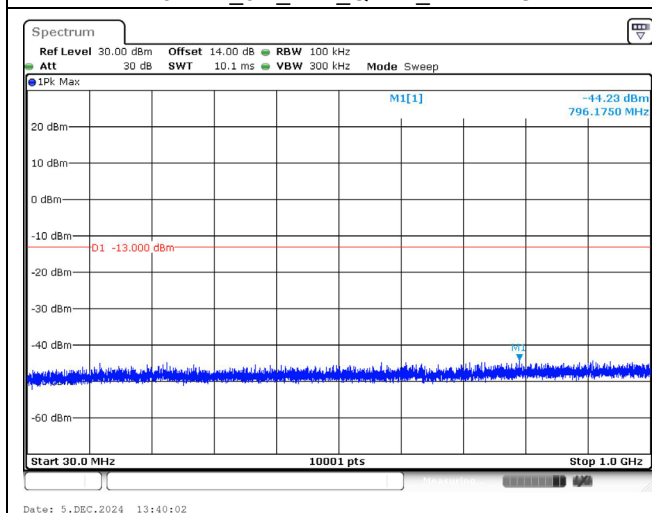
1777.5 MHz_5M_1RB_QPSK_Below 1GHz
