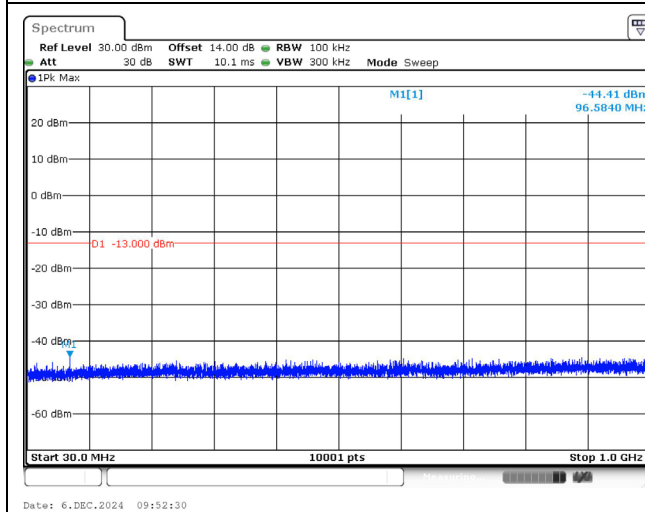
1880.0 MHz_20M_1RB_QPSK_Below 1GHz
