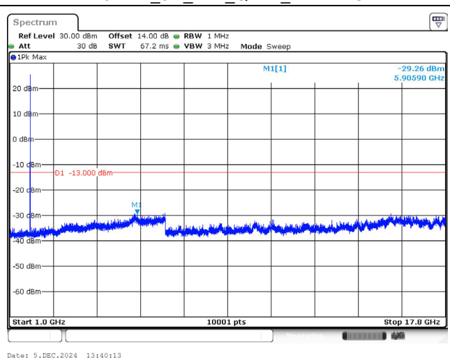
1777.5 MHz_5M_1RB_QPSK_Above 1GHz
