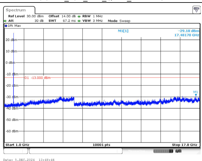
1775.0MHz_10M_1RB_QPSK_Above 1GHz
