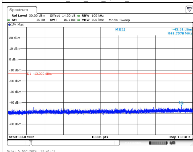
1745.0 MHz_10M_1RB_QPSK_Below 1GHz
