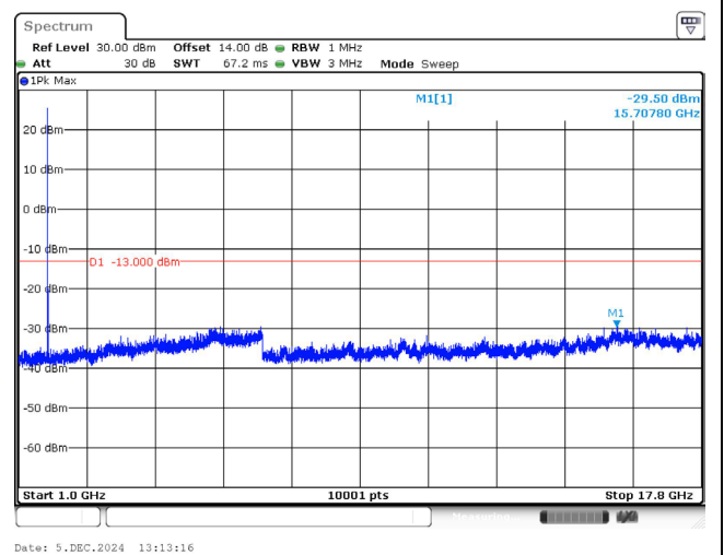
1745.0 MHz_3M_1RB_QPSK_Above 1GHz
