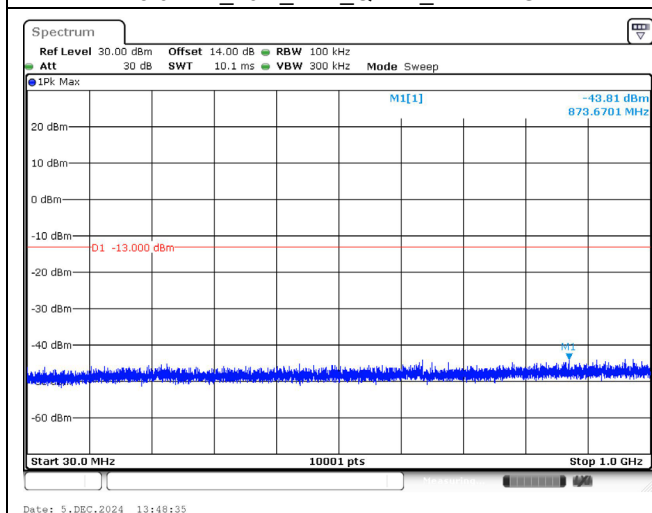
1775.0MHz_10M_1RB_QPSK_Below 1GHz
