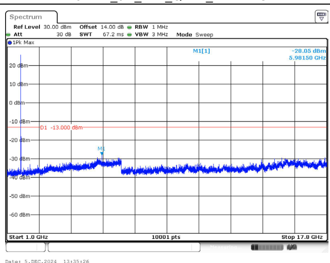
1712.5 MHz_5M_1RB_QPSK_Above 1GHz
