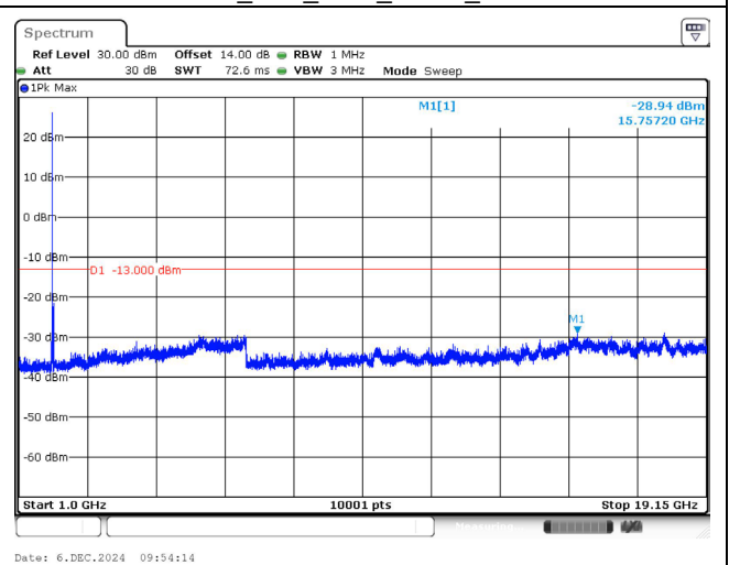
1900.0 MHz_20M_1RB_QPSK_Above 1GHz
