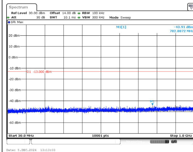
1745.0 MHz_3M_1RB_QPSK_Below 1GHz
