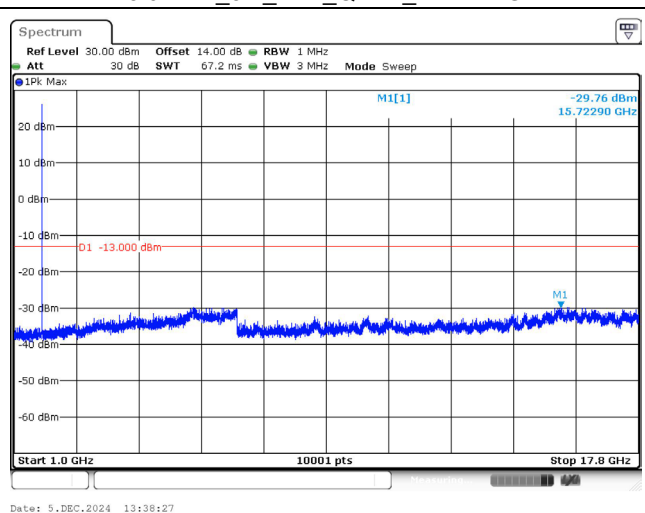
1745.0 MHz_5M_1RB_QPSK_Above 1GHz
