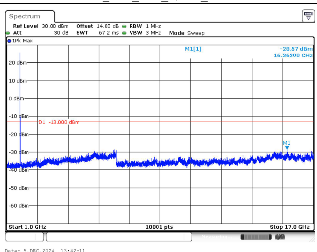
1745.0 MHz_10M_1RB_QPSK_Above 1GHz
