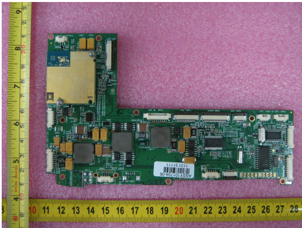
Power board (without GSM module) Top view
