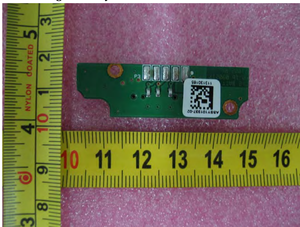
Right battery connector board Bottom view
