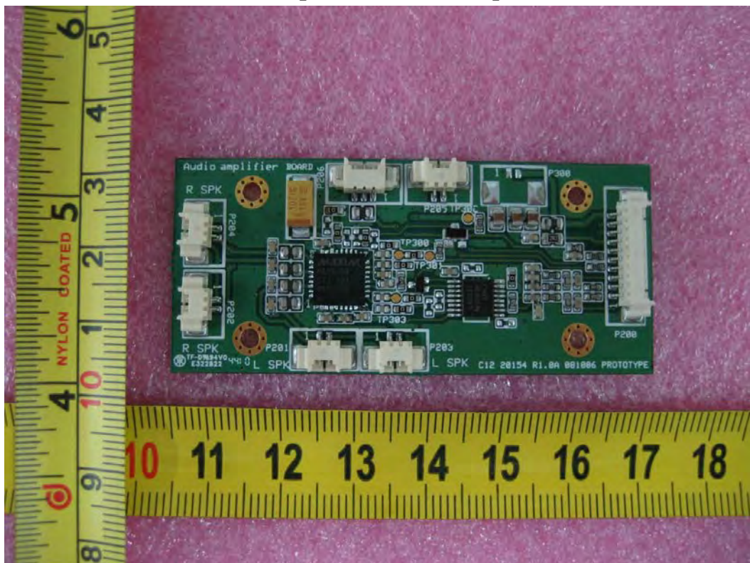
Audio amplifier board Top view
