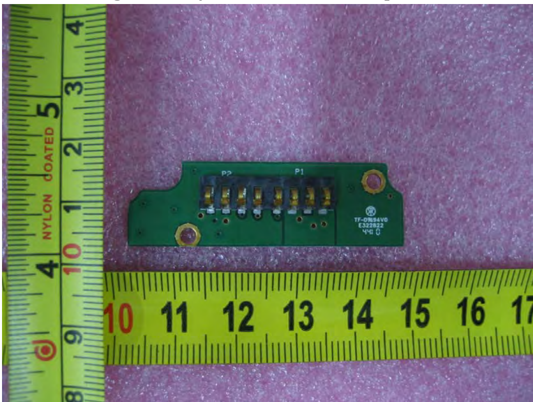
Right battery connector board Top view
