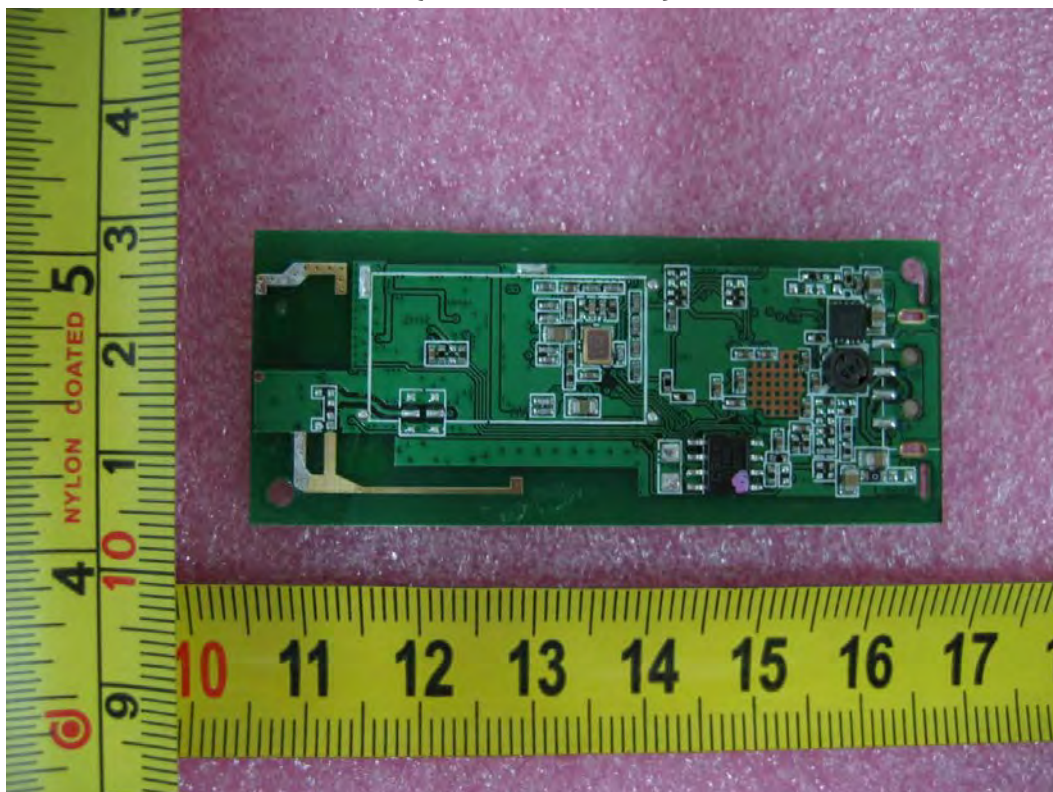
WLAN Module (without cover) Bottom view
