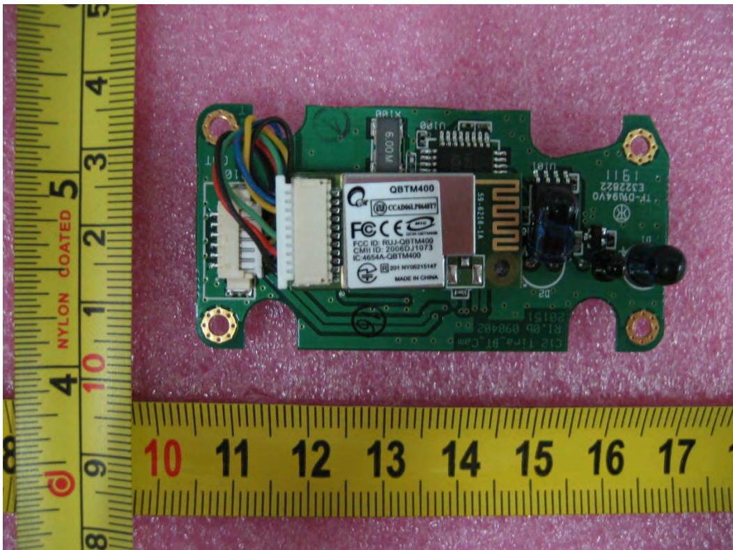
Tira/Bluetooth board (with Bluetooth module) Top view
