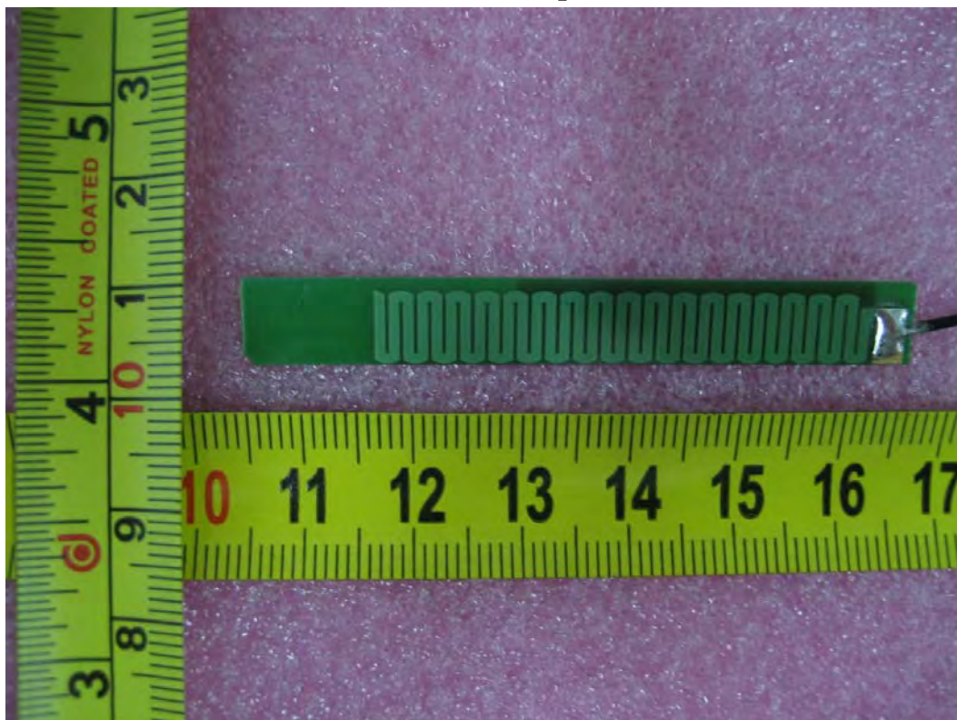
GSM antenna Top view
