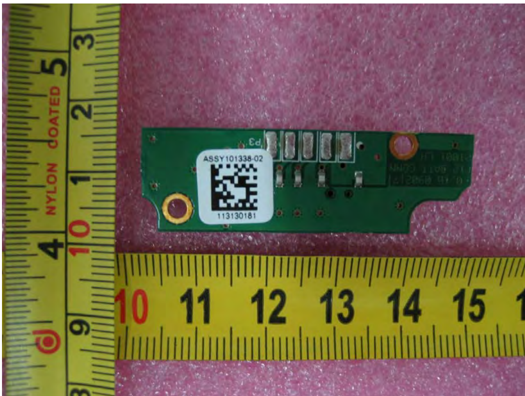
Left battery connector board Bottom view
