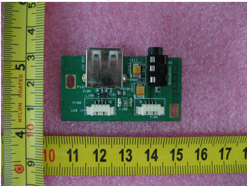
USB and Headphone board Top view
