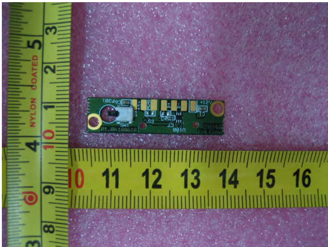
Extension connector board Bottom view
