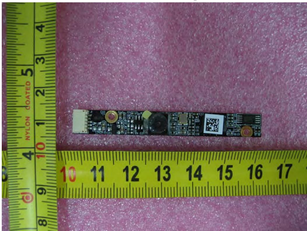
User camera board Top view
