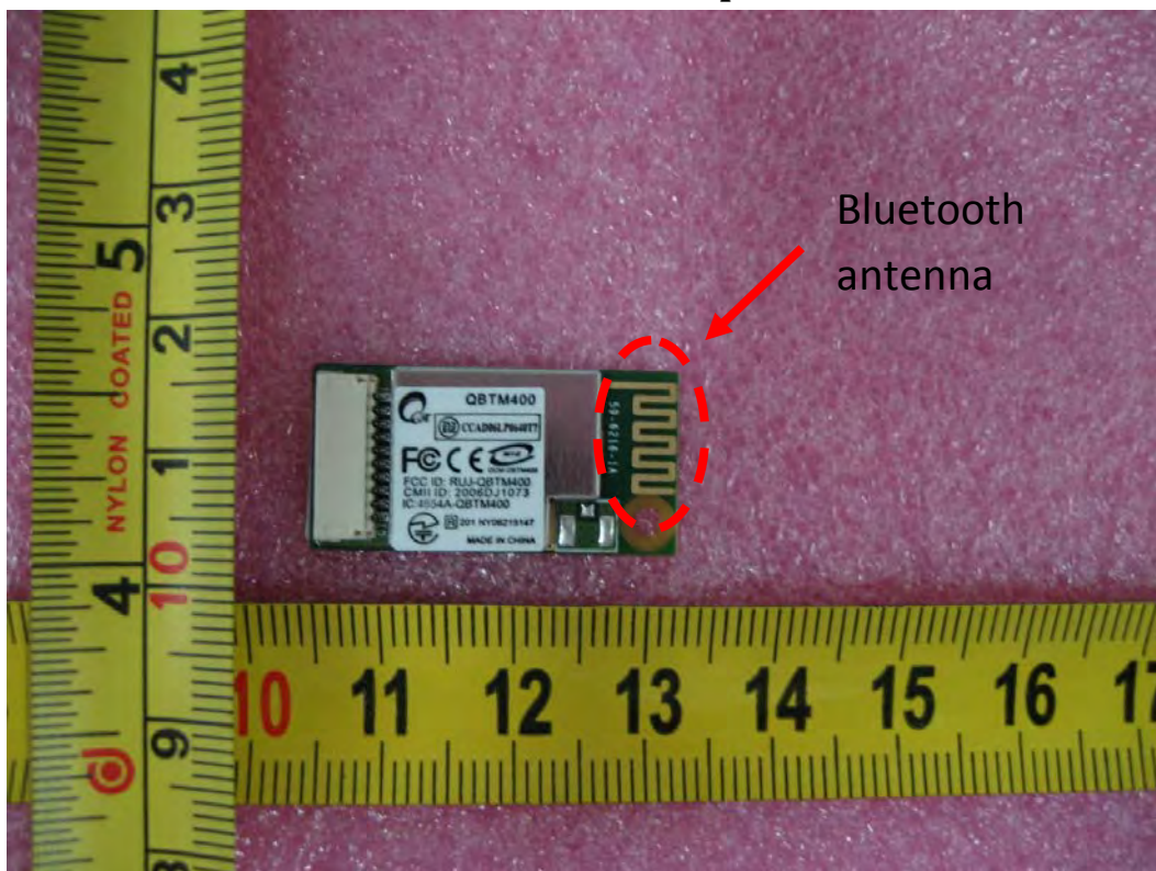
Bluetooth module Top view
