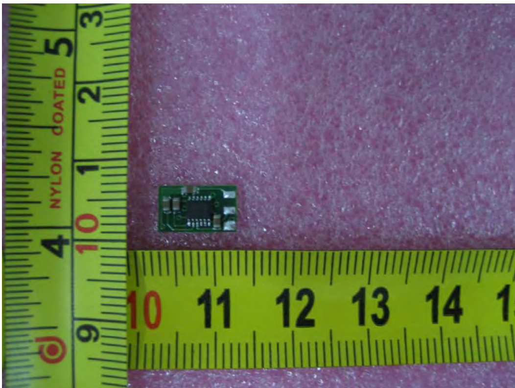
LED board Bottom view
