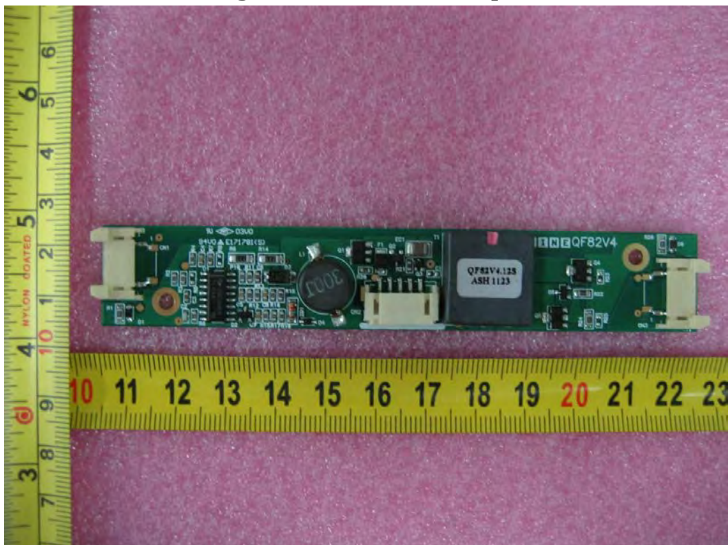
Backlight inverter board Top view
