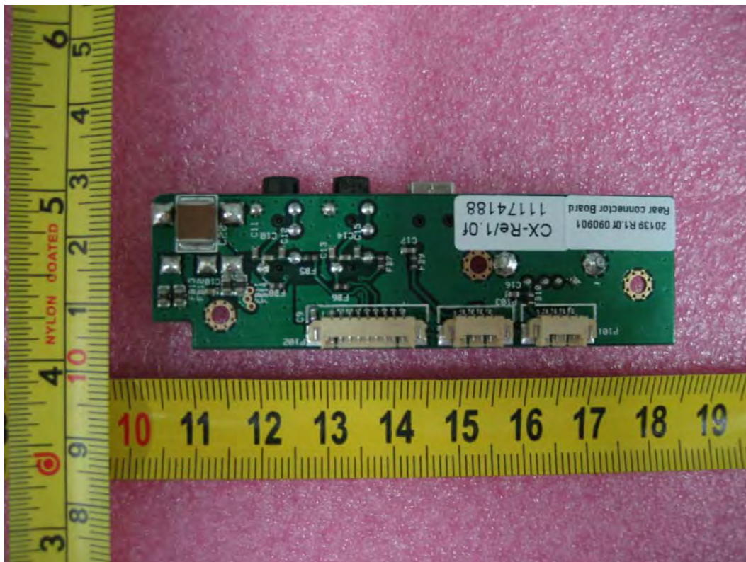
Rear connector board Bottom view
