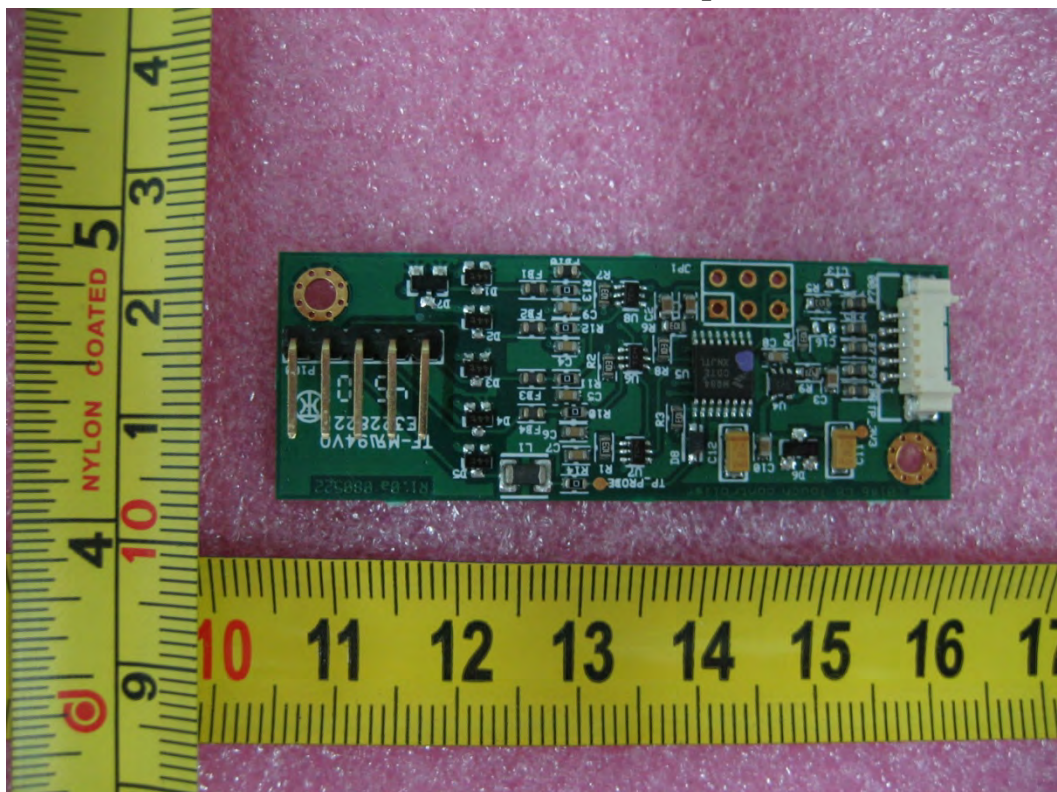
Touch controller board Top view
