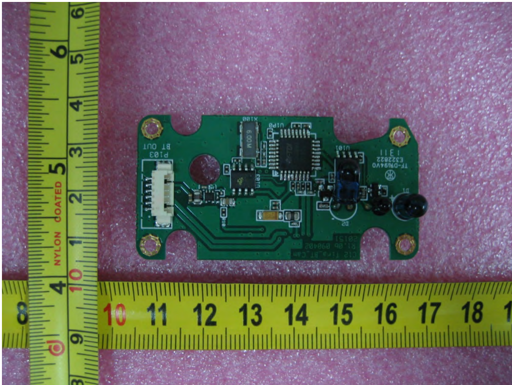
Tira/Bluetooth board (without Bluetooth module) Top view
