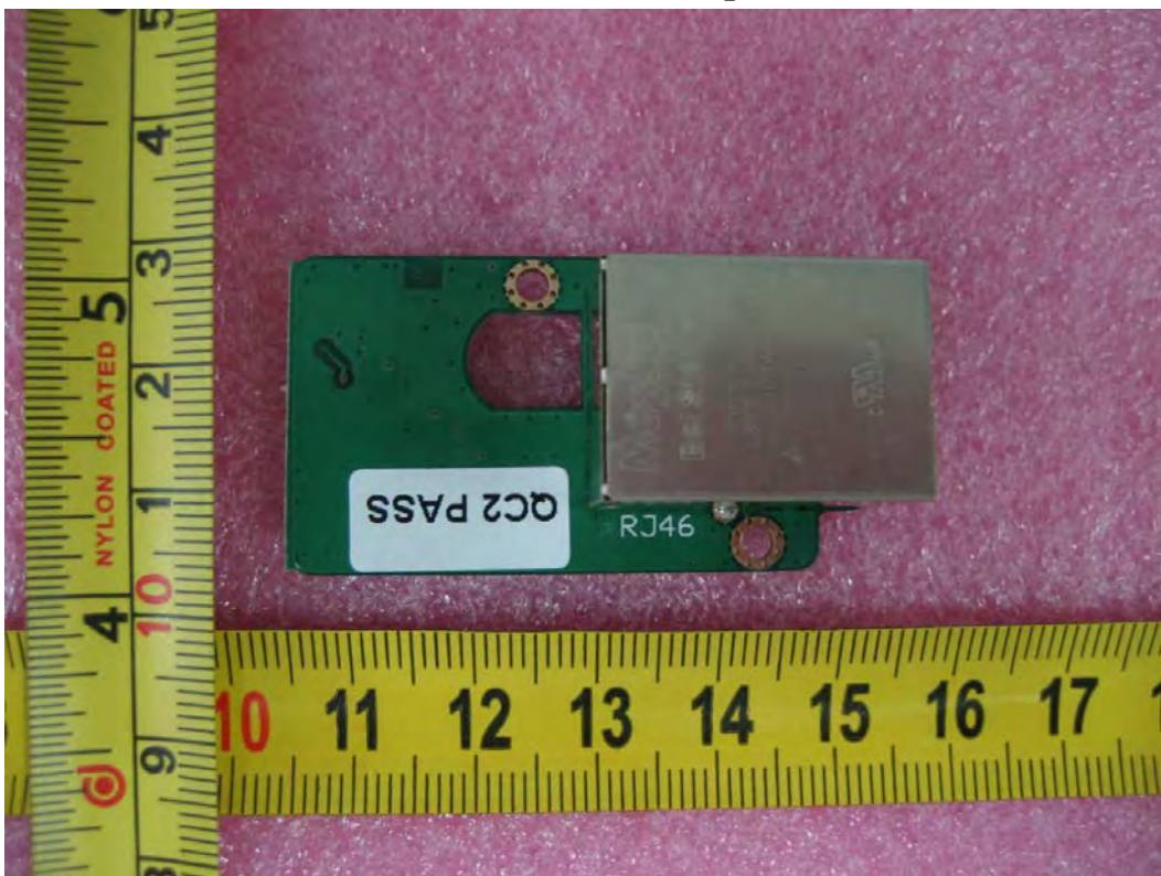
LAN section board Top view
