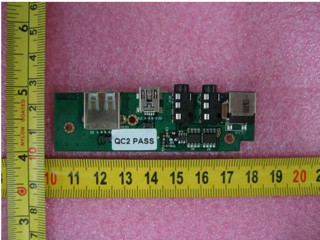
Rear connector board Top view
