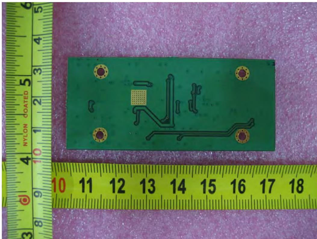
Audio amplifier board Bottom view
