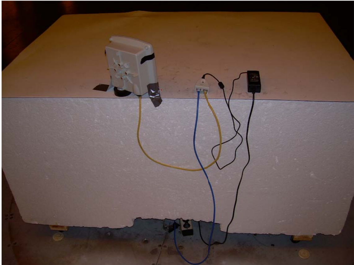
Back View Worst-Case Radiated Emissions Configuration
