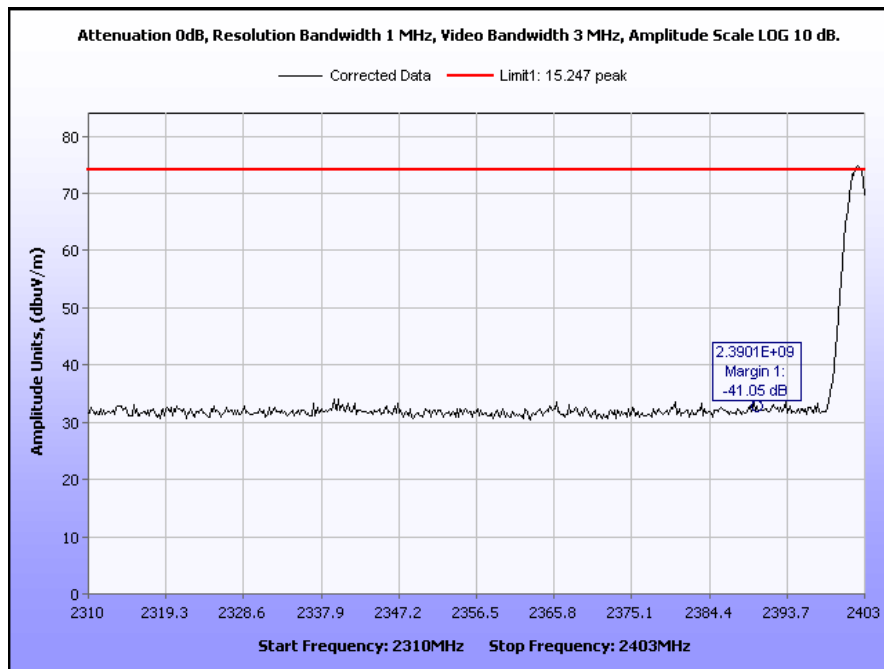
Plot 20. Lower Band Edge, Peak, Bluetooth
