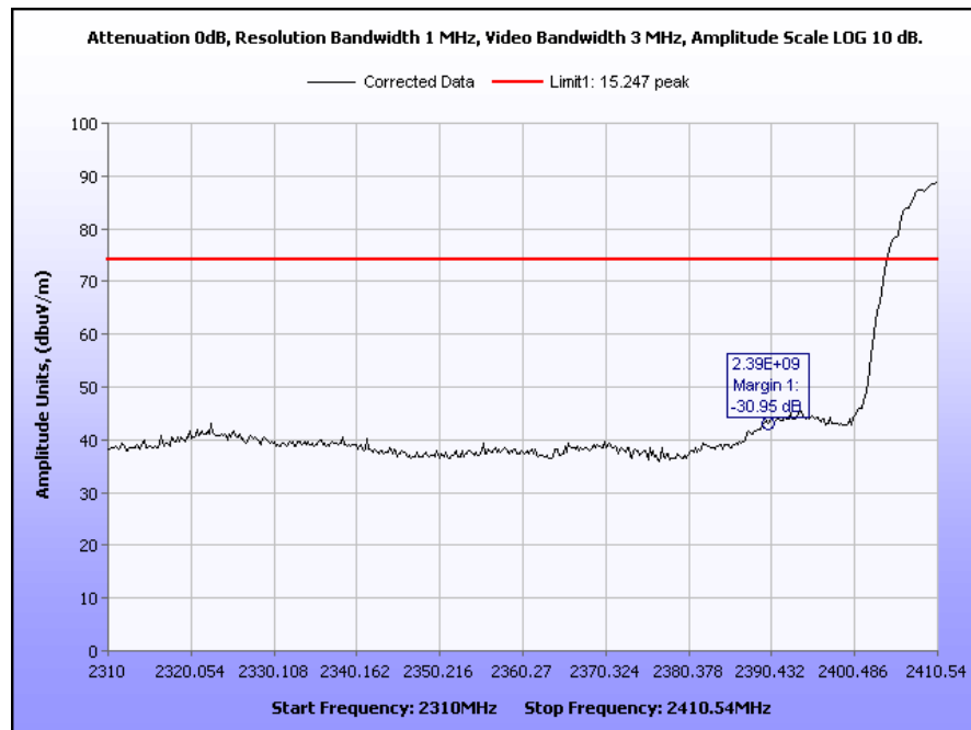
Plot 12. Lower Band Edge, Peak, 802.11b
