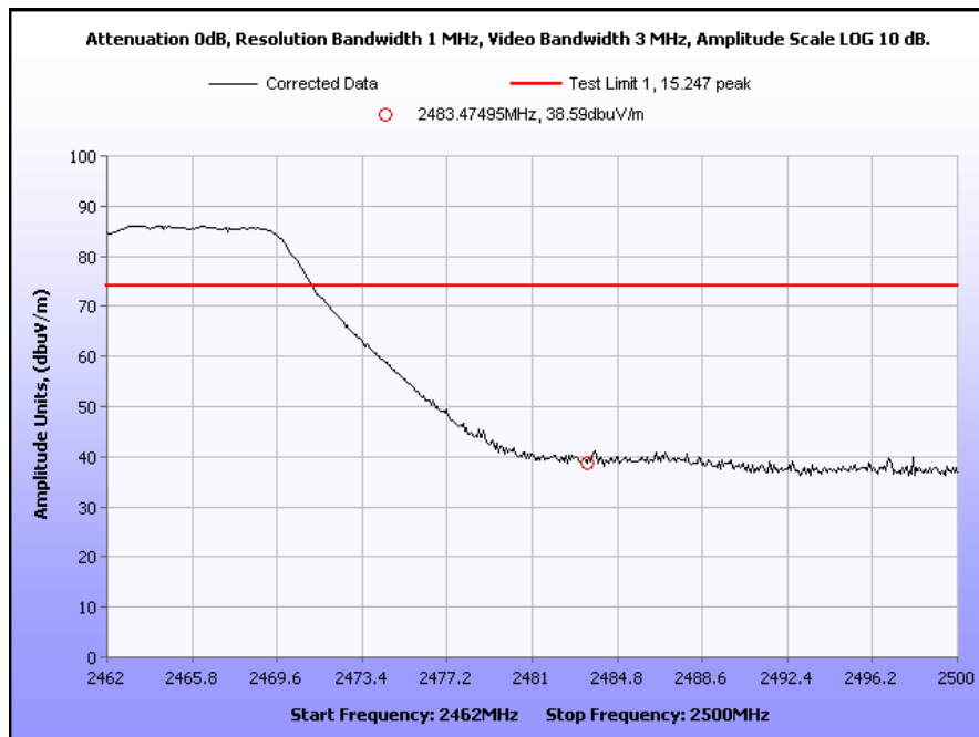
Plot 18. Upper Band Edge, Peak, 802.11g
