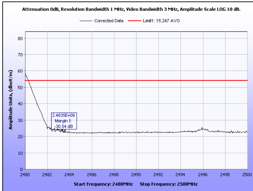
Plot 21. Upper Band Edge, Average Detector, Bluetooth
