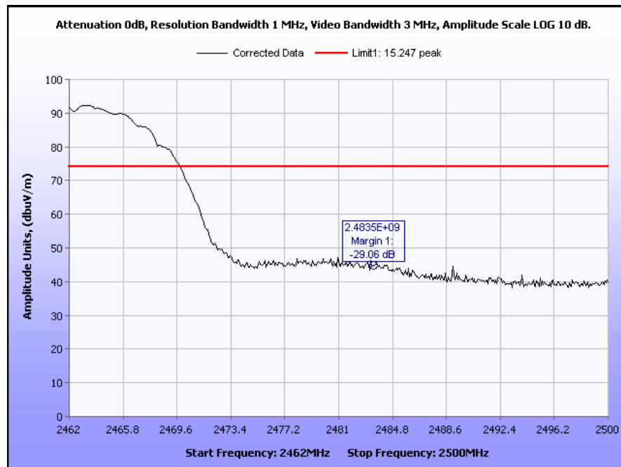
Plot 14. Upper Band Edge, Peak, 802.11b
