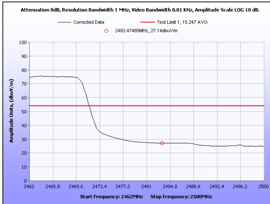
Plot 17. Upper Band Edge, Average, 802.11g
