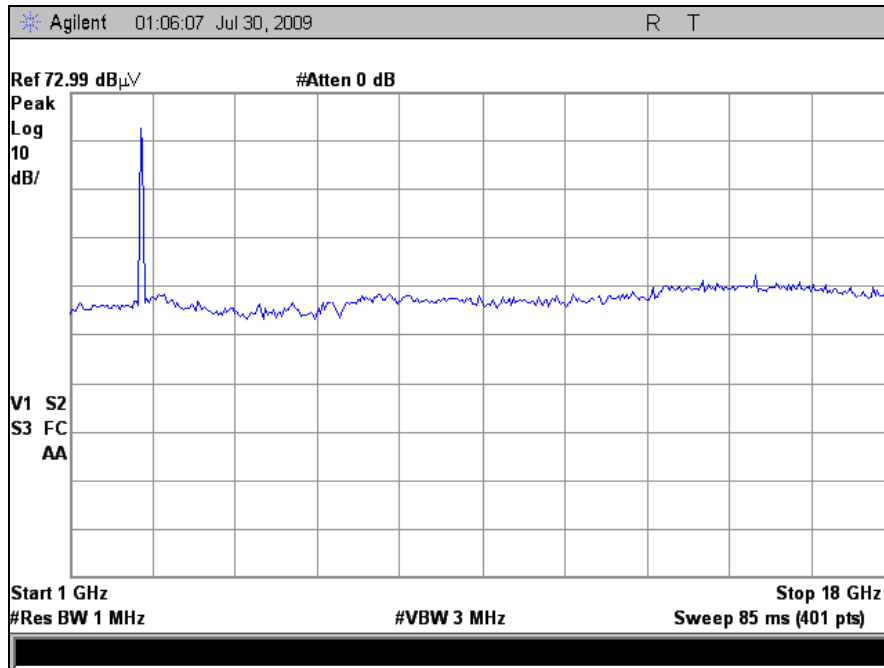
Plot 8. Radiated Spurious Emissions, 802.11g, Mid Channel
