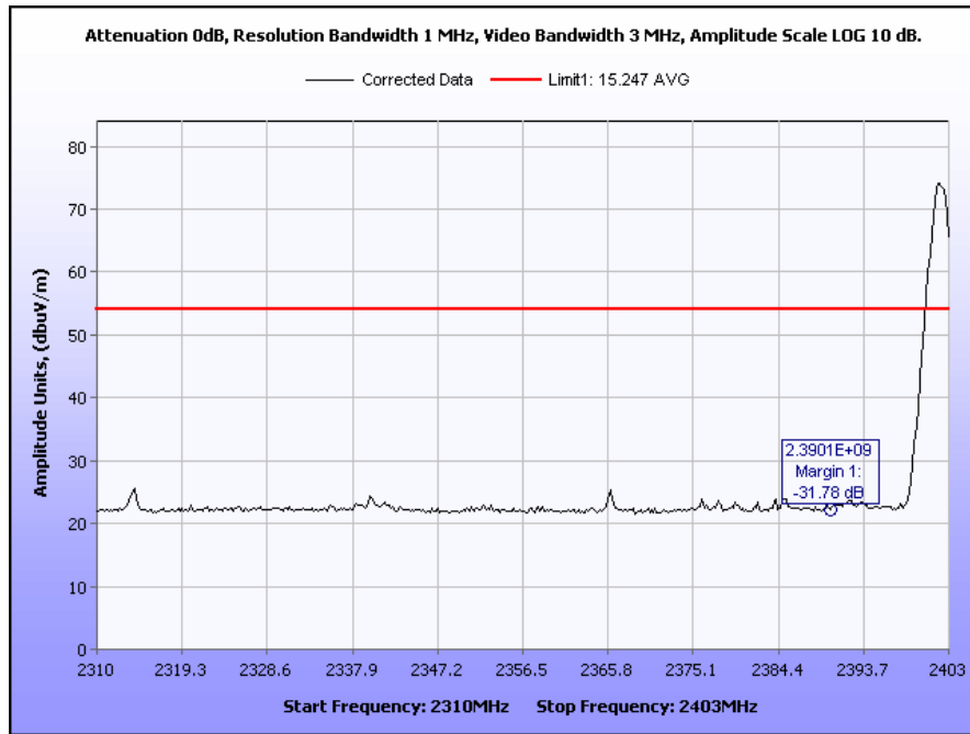
Plot 19. Lower Band Edge, Average Detector, Bluetooth
