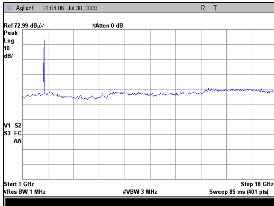
Plot 7. Radiated Spurious Emissions, 802.11g, Low Channel
