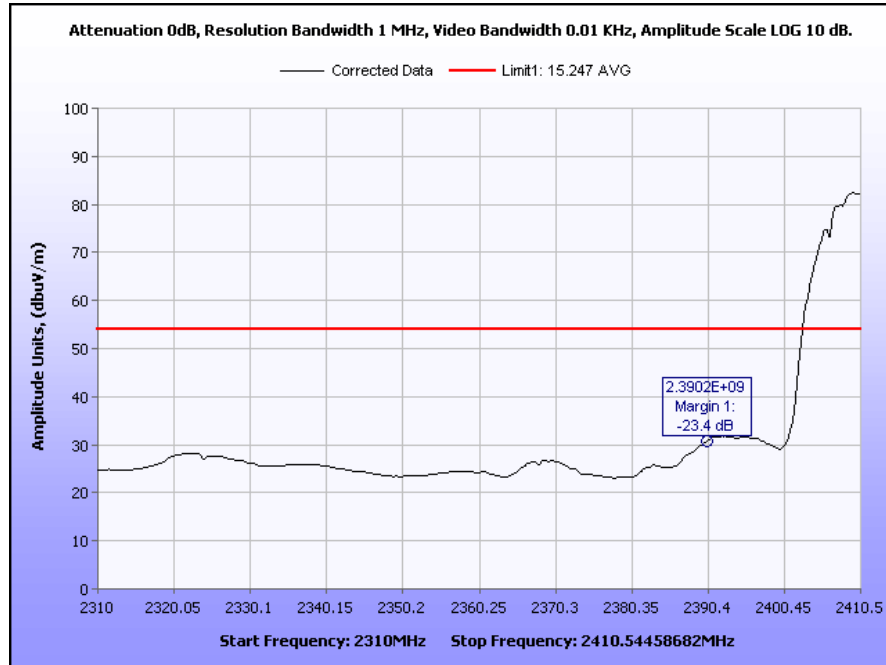
Plot 11. Lower Band Edge, Average, 802.11b
