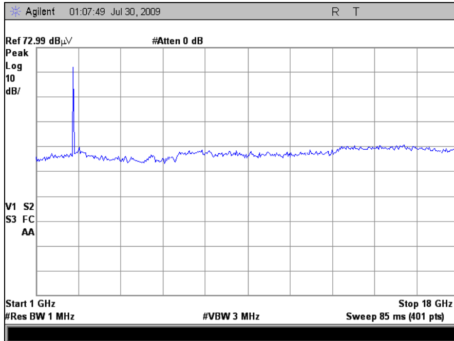
Plot 9. Radiated Spurious Emissions, 802.11g, High Channel
