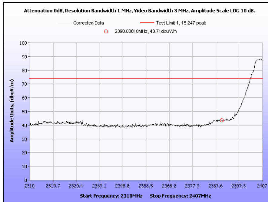
Plot 16. Lower Band Edge, Peak, 802.11g
