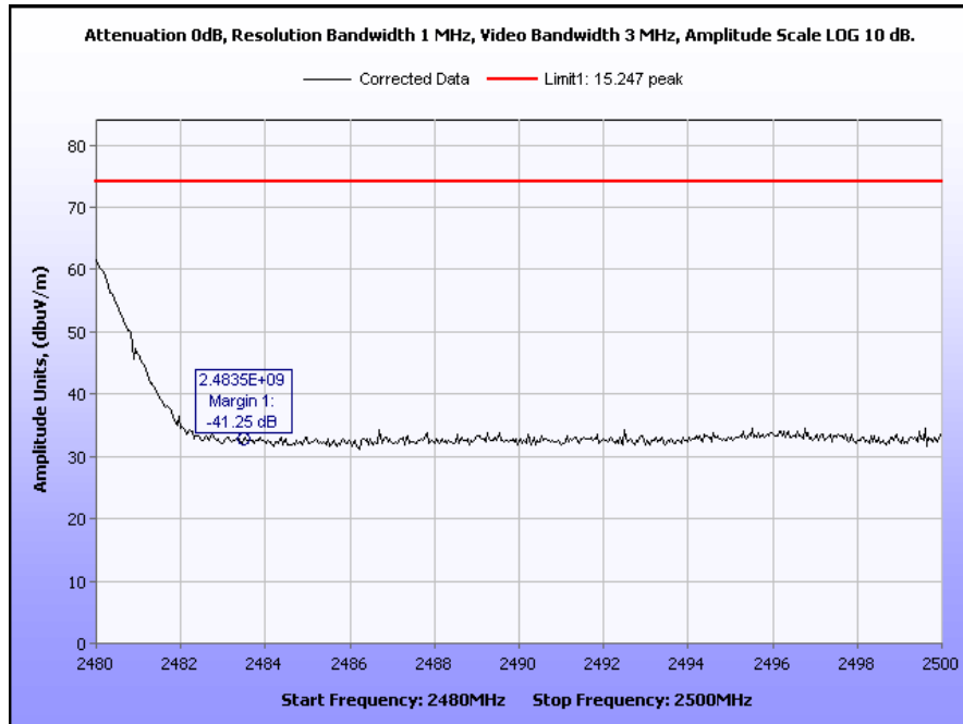
Plot 22. Upper Band Edge, Peak, Bluetooth
