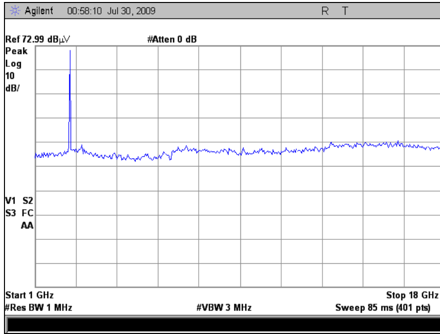
Plot 4. Radiated Spurious Emissions, 802.11b, Low Channel
