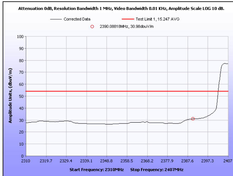
Plot 15. Lower Band Edge, Average, 802.11g
