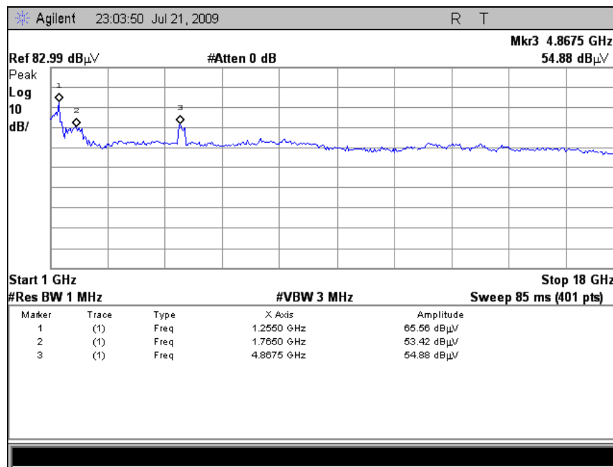
Plot 10. Radiated Spurious Emissions, Bluetooth
