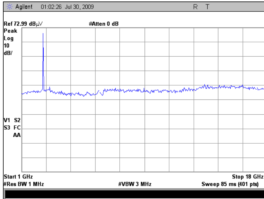
Plot 6. Radiated Spurious Emissions, 802.11b, High Channel
