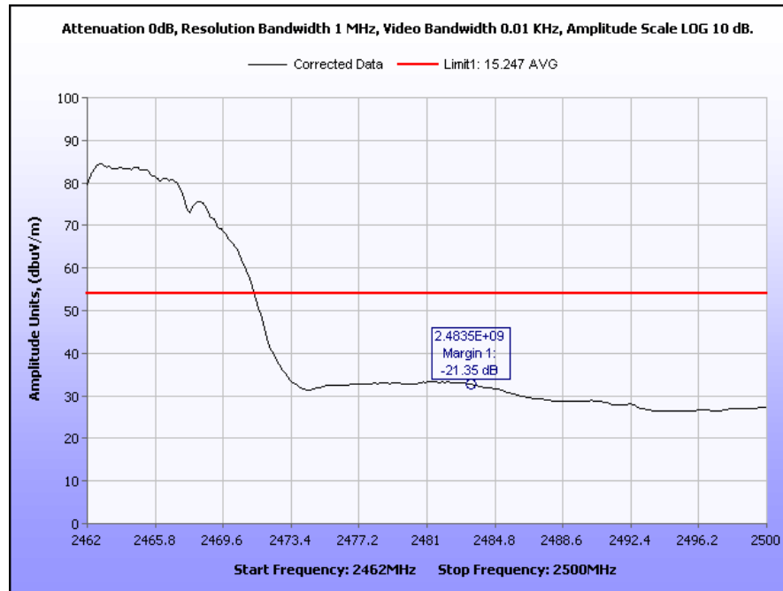
Plot 13. Upper Band Edge, Average, 802.11b
