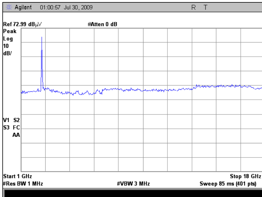
Plot 5. Radiated Spurious Emissions, 802.11b, Mid Channel
