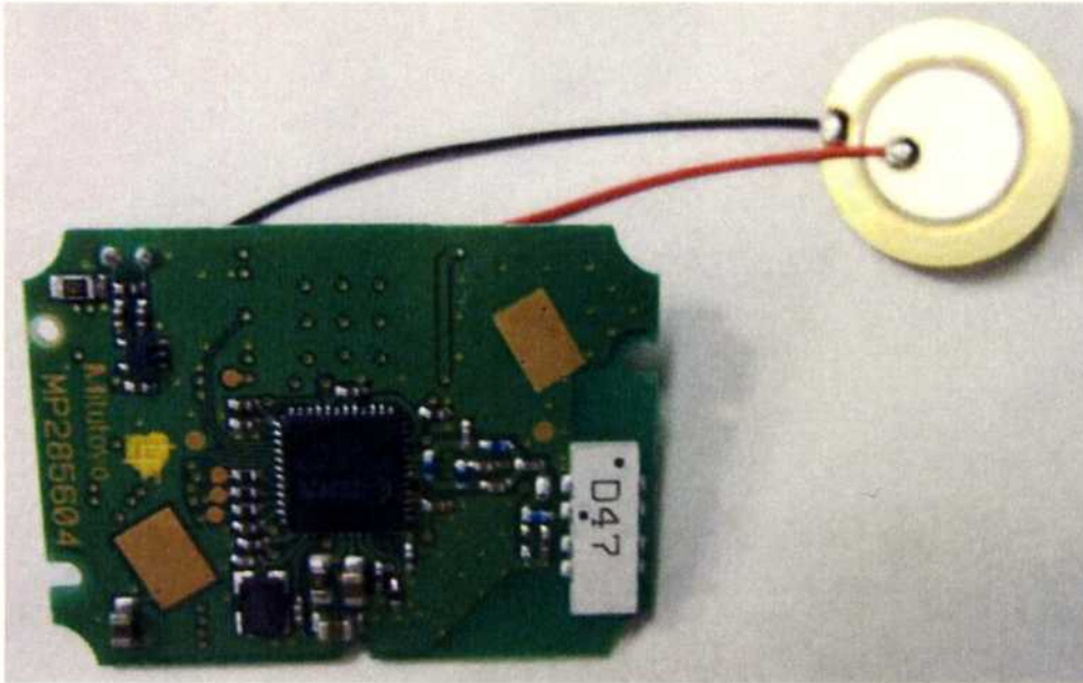
U-WAVE-T/ 02AZD880D without plastic material Internal Photos Surface
