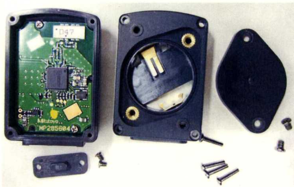
U-WAVE-T/ 02AZD880D Board with case Internal Photos1
