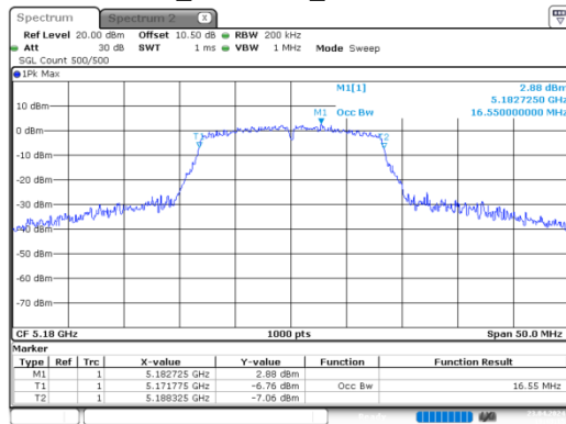
a_5180MHz_Chain 0
