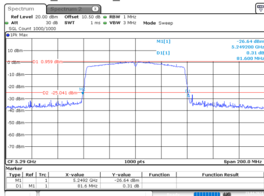
ac80_5290MHz_Chain 0 81.600 MHz
