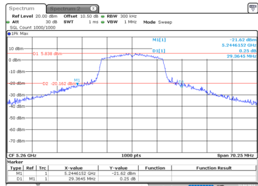
n20_5260MHz_Chain 0
