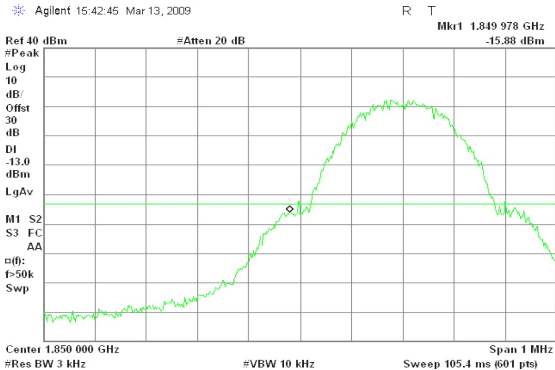
Figure 10-3: Band Edge emissions – GSM CH Low
