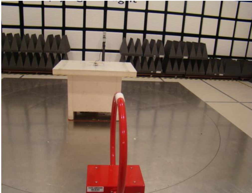
Test setup
