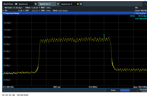
Channel 07 (5985MHz)
