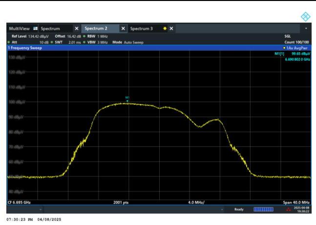
Channel 149 (6695MHz)
