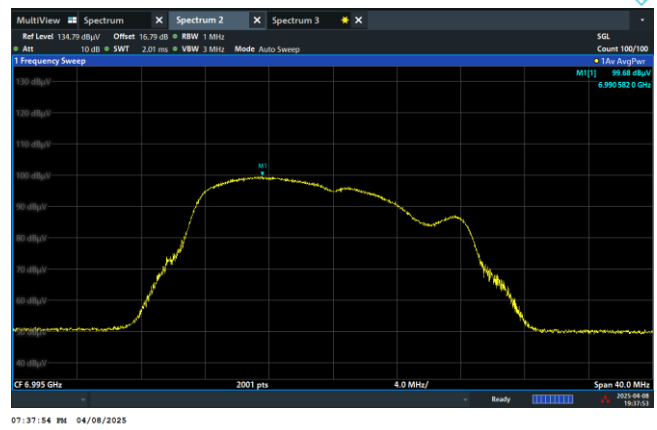
Channel 209 (6995MHz)
