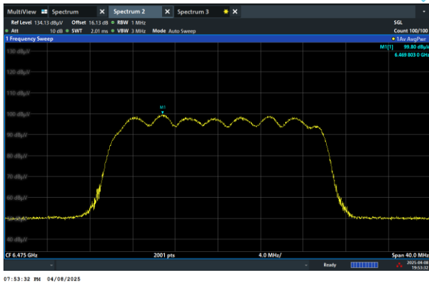
Channel 105 (6475MHz)
