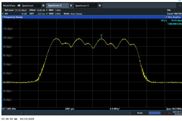
Channel 229 (7095MHz)
