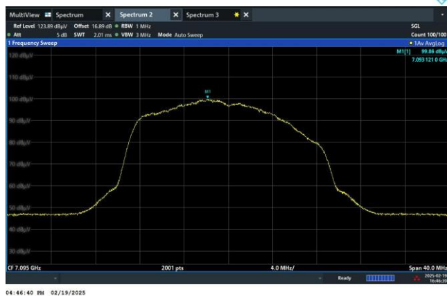
Channel 229 (7095MHz)
