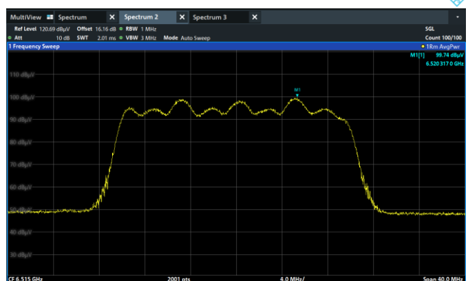
Channel 113 (6515MHz)
