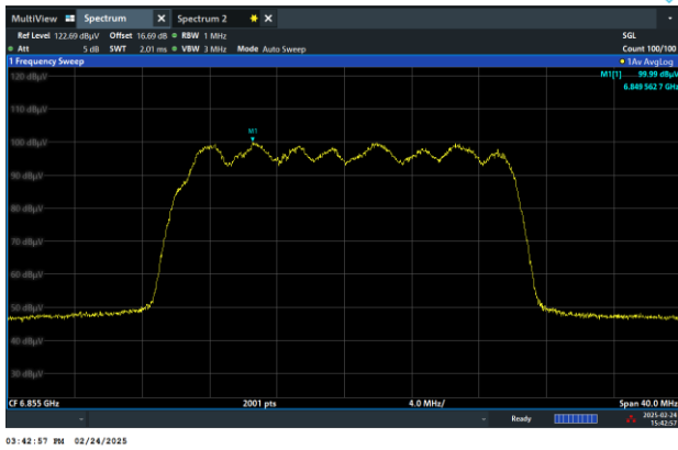
Channel 181 (6855MHz)
