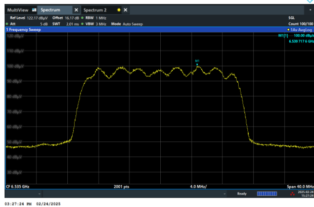
Channel 117 (6535MHz)
