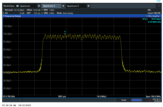
Channel 167 (6785MHz)
