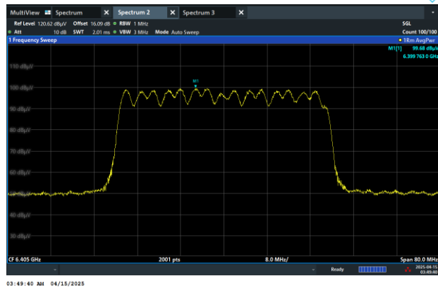
Channel 91 (6405MHz)
