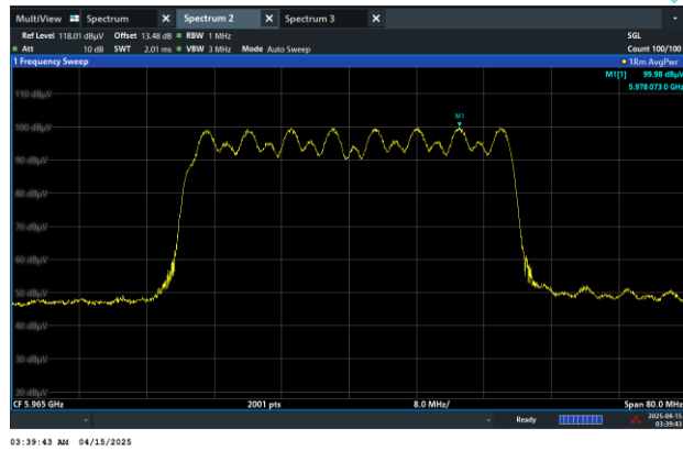
Channel 03 (5965MHz)
