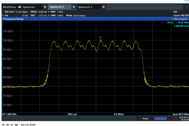
Channel 227 (7085MHz)
