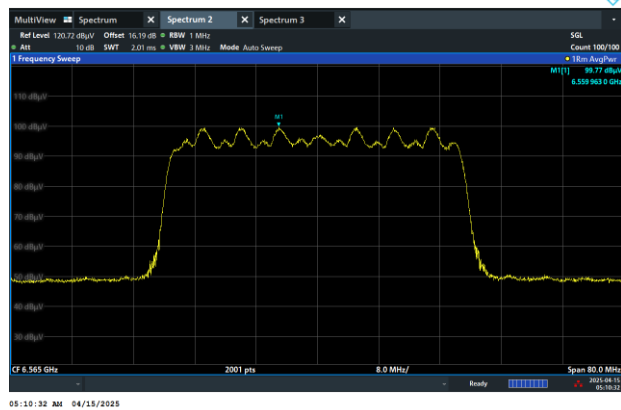
Channel 123 (6565MHz)
