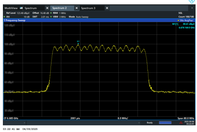
Channel 147 (6685MHz)
