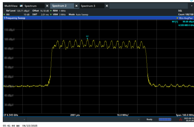
Channel 119 (6545MHz)
