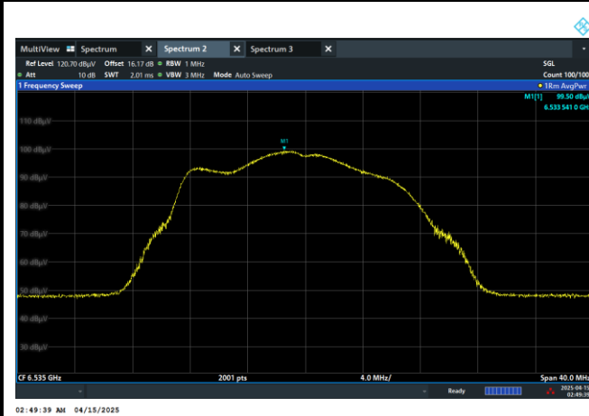
Channel 117 (6535MHz)
