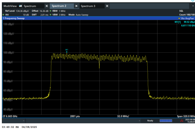
Channel 143 (6665MHz)
