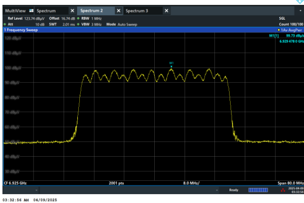
Channel 195 (6925MHz)
