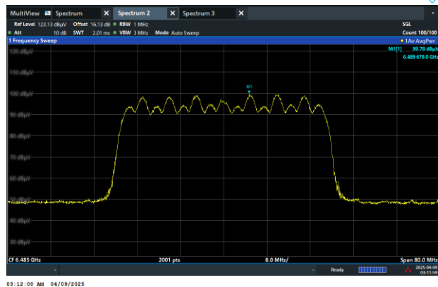
Channel 107 (6485MHz)
