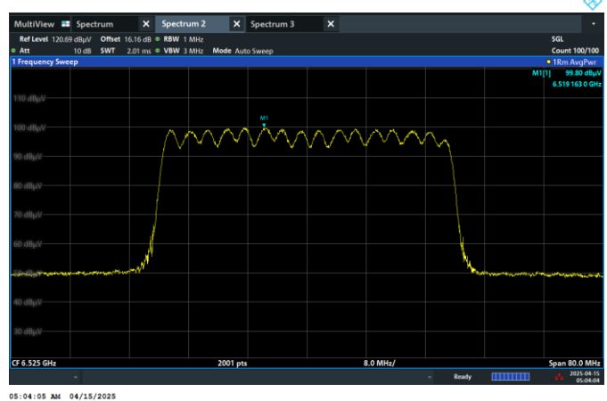
Channel 115 (6525MHz)
