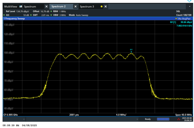
Channel 209 (6995MHz)
