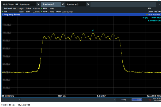
Channel 179 (6845MHz)
