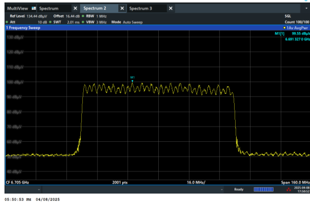
Channel 151 (6705MHz)
