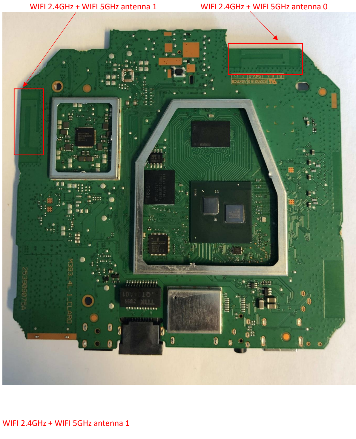
Electronic Card verso View without shielding
