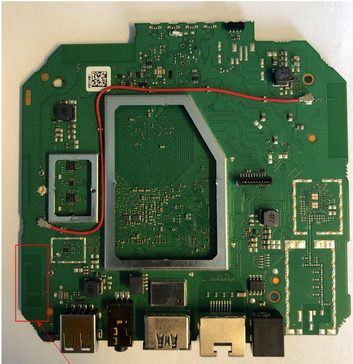
Bluetooth Low Energy + Bluetooth Classic antenna
