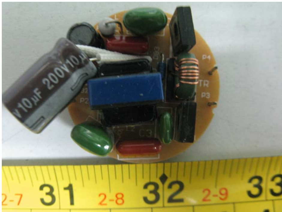
ESS-13W: EUT – Main Board Top View
