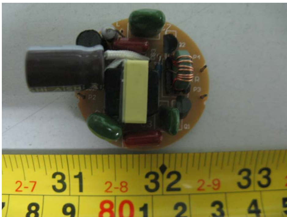
ESS-9W: EUT – Main Board Top View
