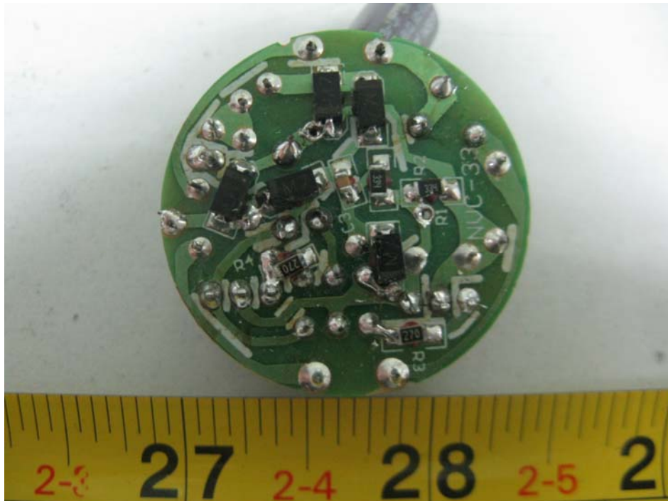
ESS-15W: EUT – Main Board Bottom View
