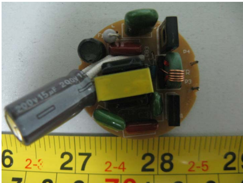
ESS-15W: EUT – Main Board Top View
