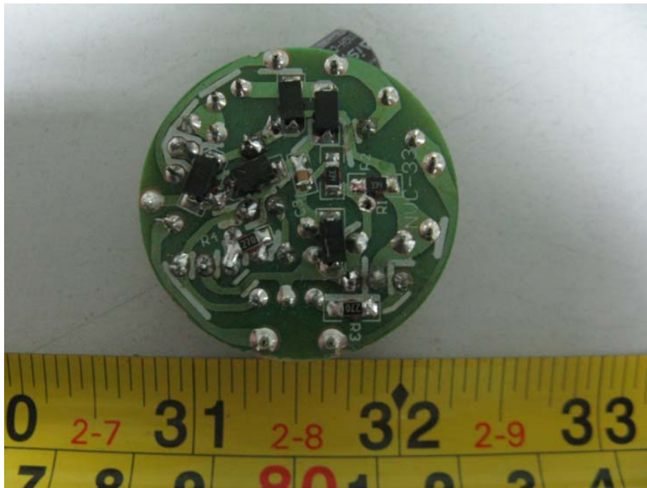
ESS-13W: EUT – Main Board Bottom View
