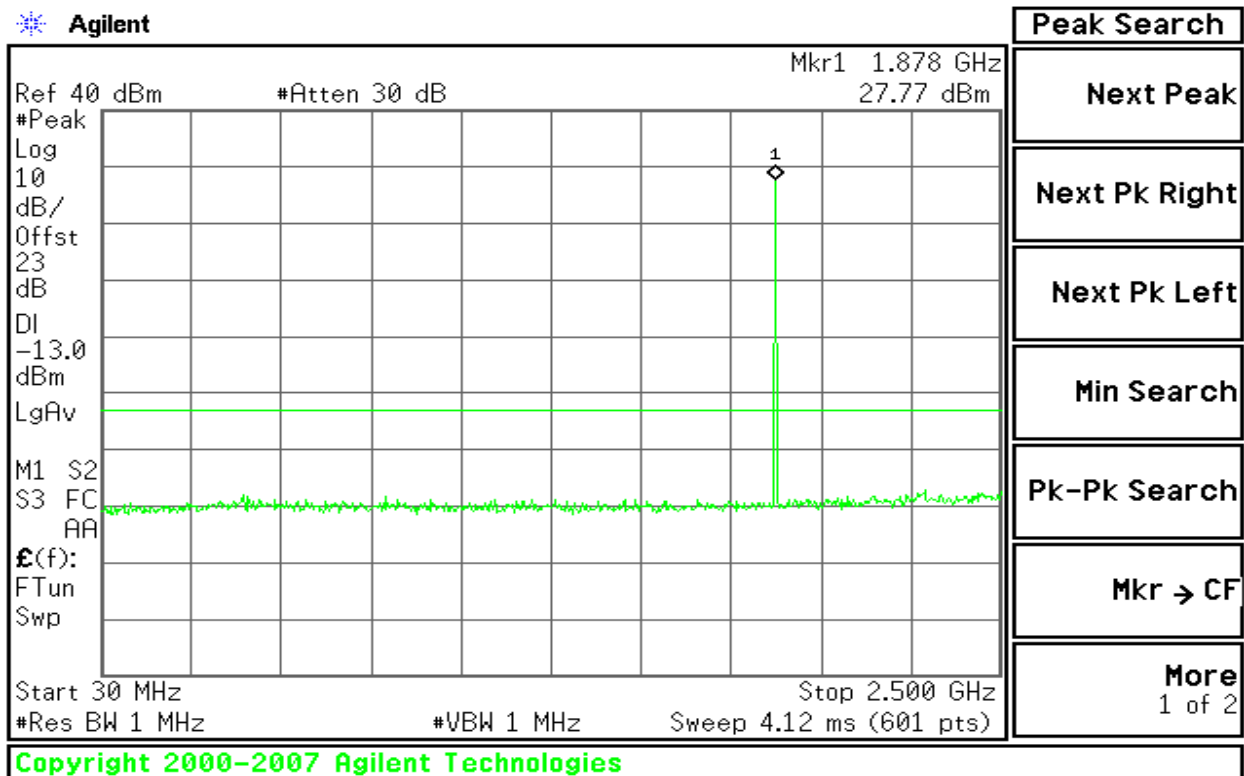
Figure 8-3: Out of Band emission at antenna terminals – GPRS CH Mid
