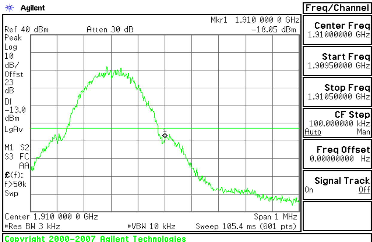
Figure 9-8: Band Edge emissions – EDGE CH High
