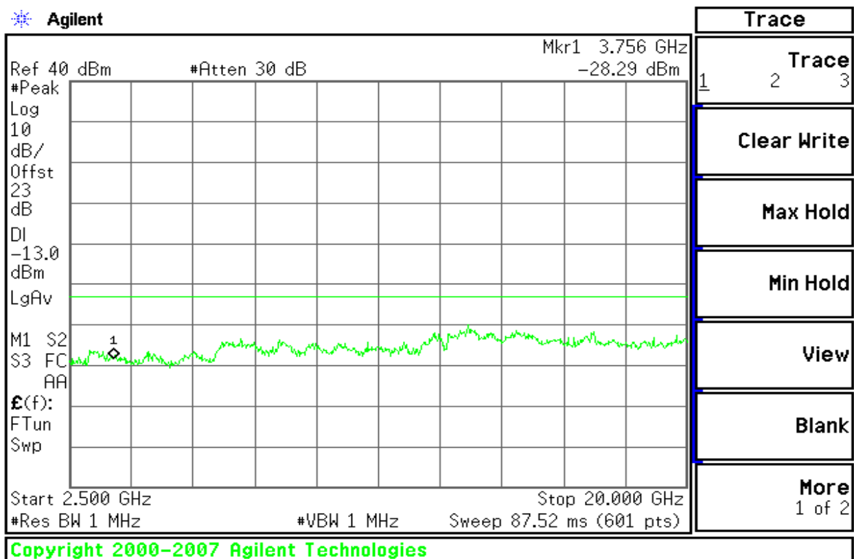
Figure 9-4: Out of Band emission at antenna terminals – EDGE CH Mid
