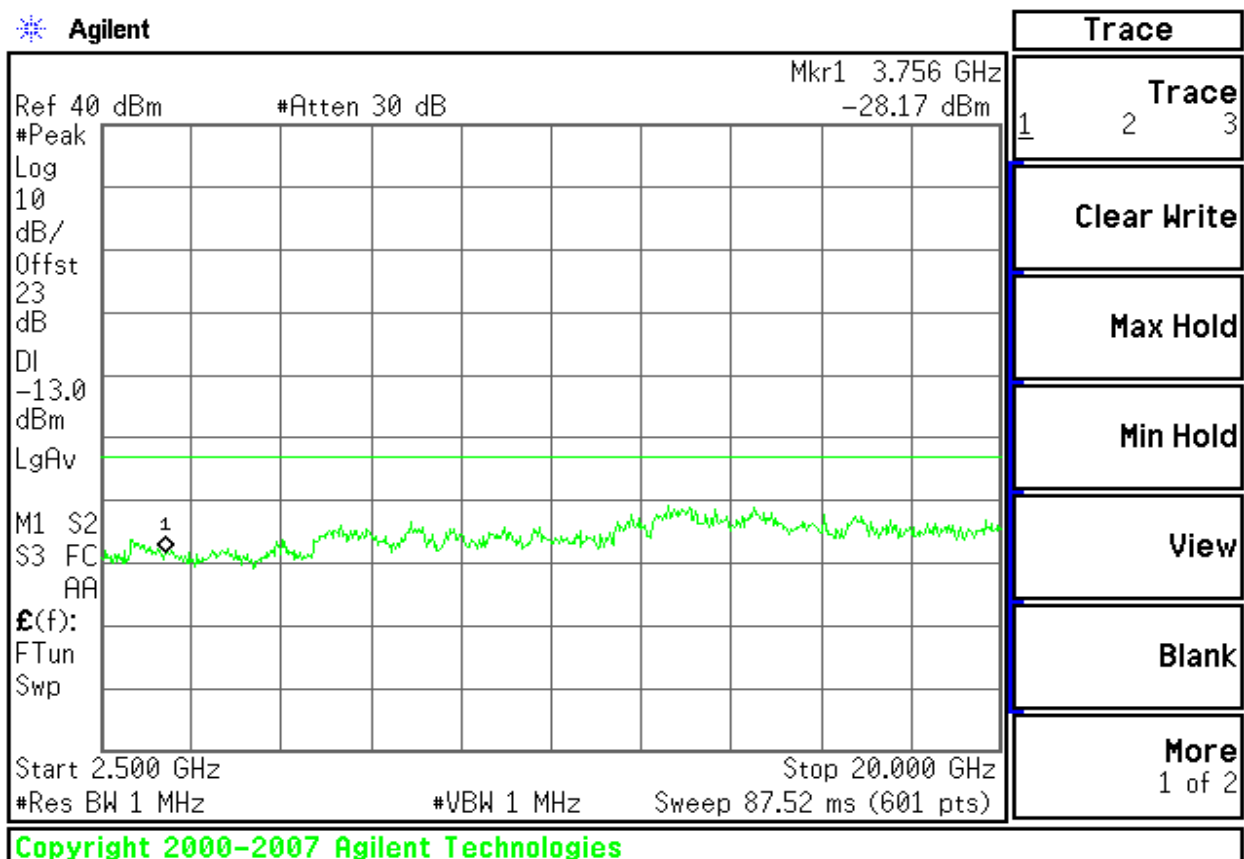
Figure 8-4: Out of Band emission at antenna terminals – GPRS CH Mid
