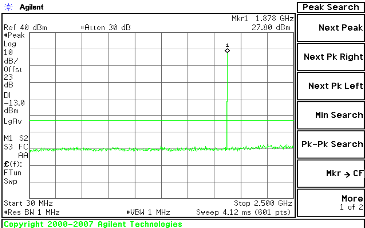
Figure 9-3: Out of Band emission at antenna terminals – EDGE CH Mid
