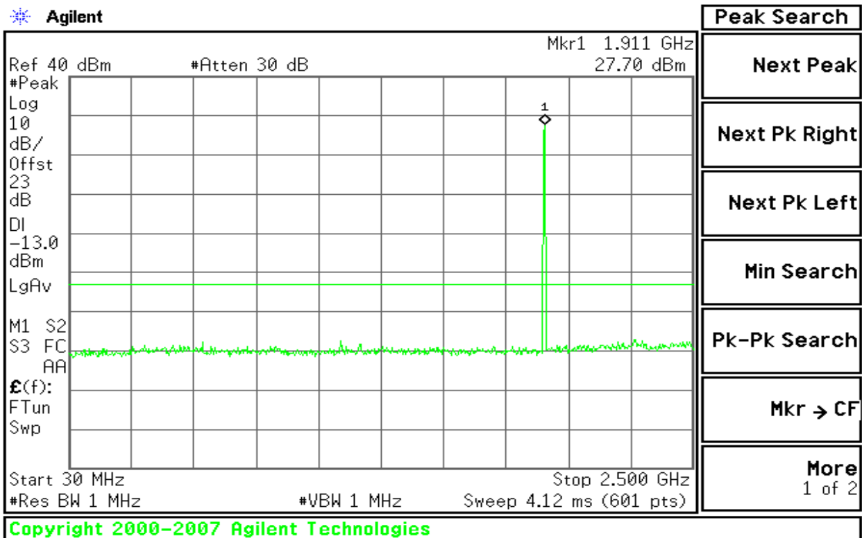
Figure 9-5: Out of Band emission at antenna terminals – EDGE CH High
