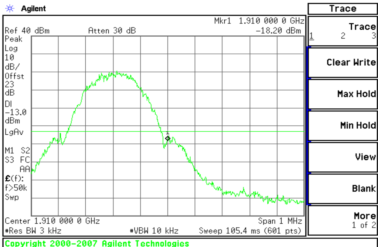
Figure 8-8: Band Edge emissions – GPRS CH High
