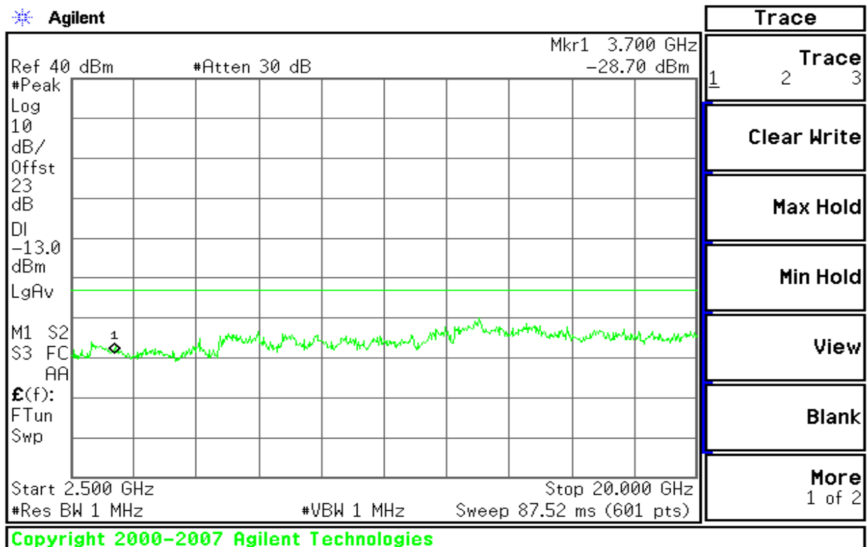
Figure 8-2: Out of Band emission at antenna terminals – GPRS CH Low
