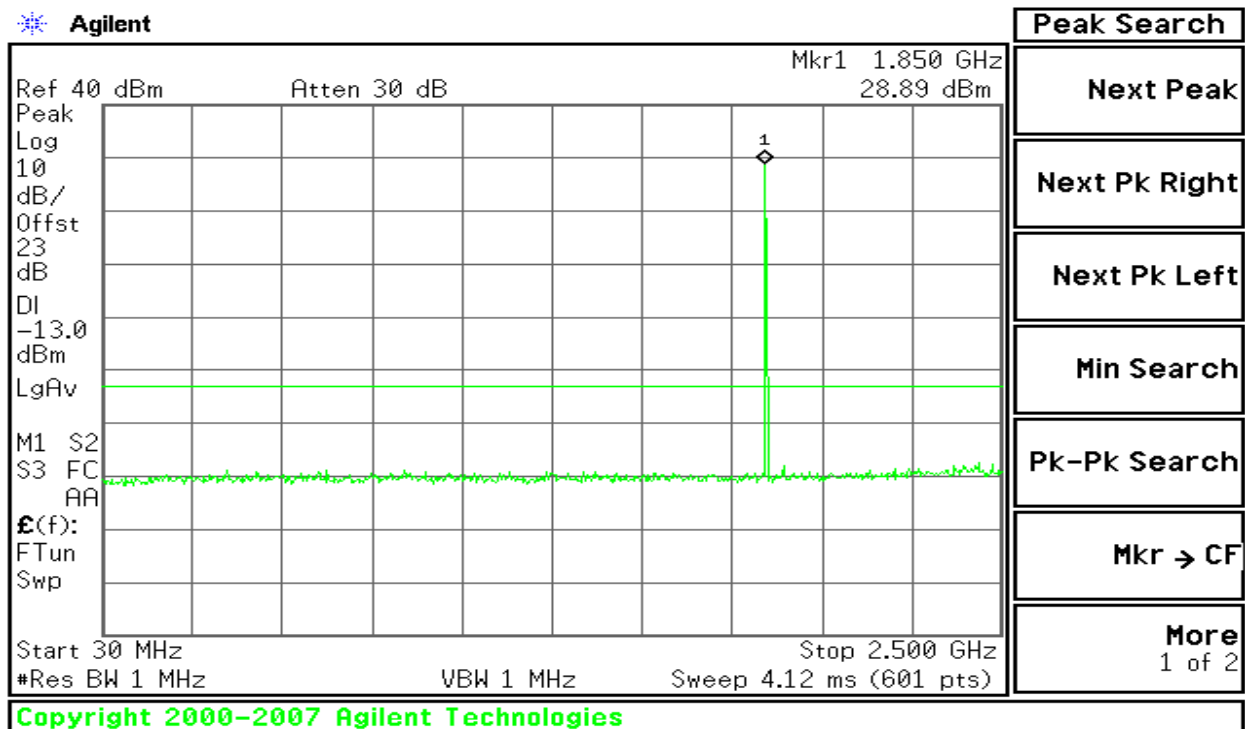
Figure 7-1: Out of Band emission at antenna terminals – GSM CH Low
