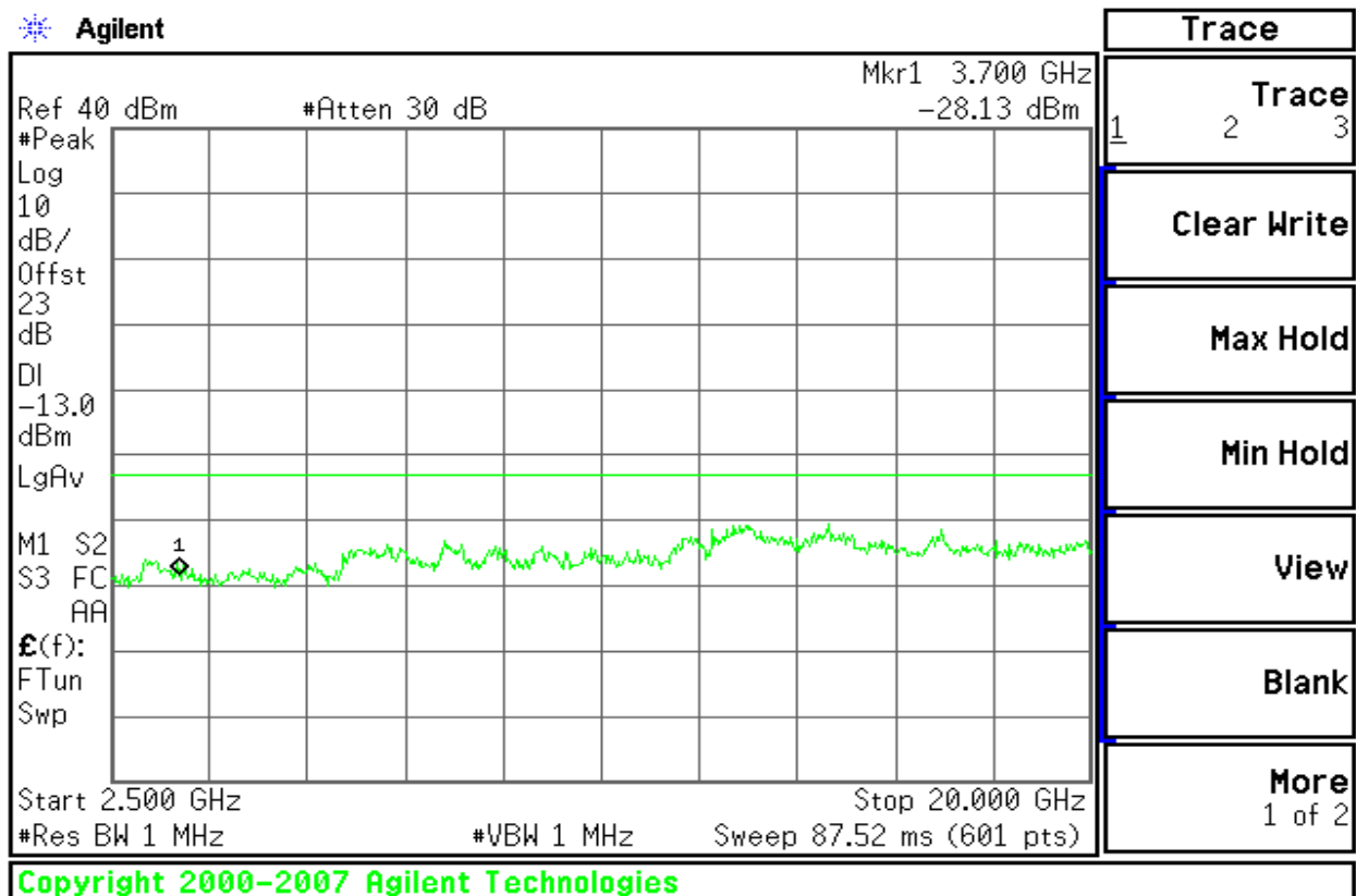
Figure 9-2: Out of Band emission at antenna terminals –EDGE CH Low
