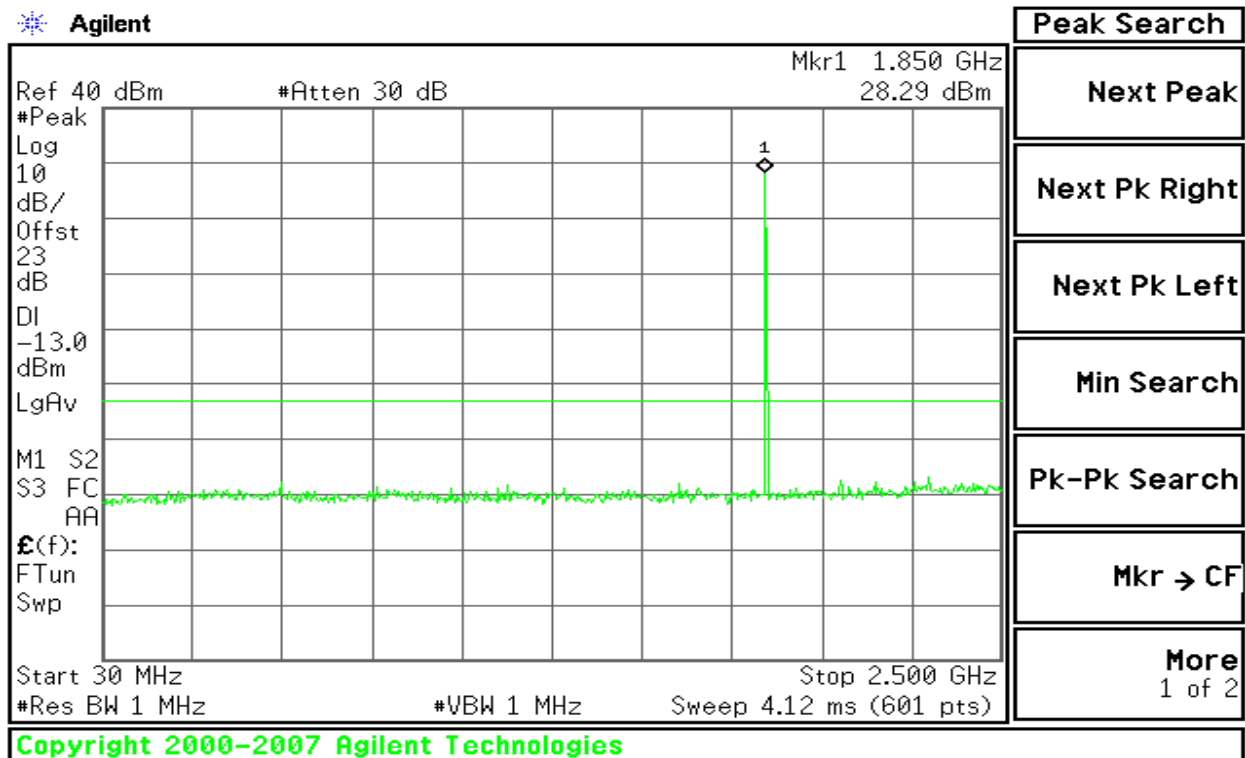
Figure 9-2: Out of Band emission at antenna terminals –EDGE CH Low
