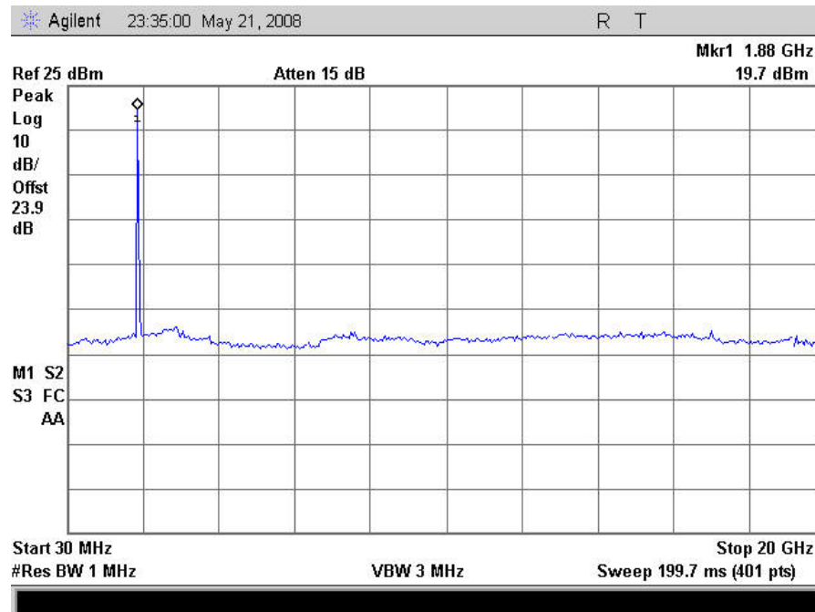
Plot 56. Conducted Spurious Emissions, CDMA Mid Channel Uplink
