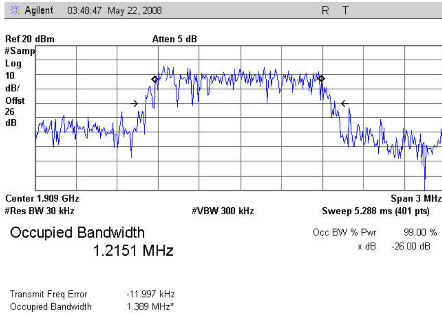
Plot 25. Occupied Bandwidth, CDMA Uplink, High Channel Output
