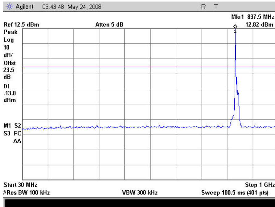
Plot 43. Conducted Spurious Emissions, CDMA Mid Channel Uplink, 30MHz – 1GHz
