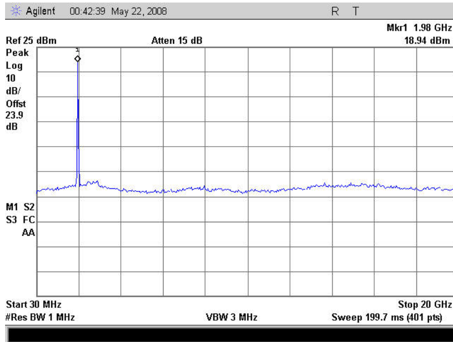
Plot 57. Conducted Spurious Emissions, CDMA High Channel Downlink
