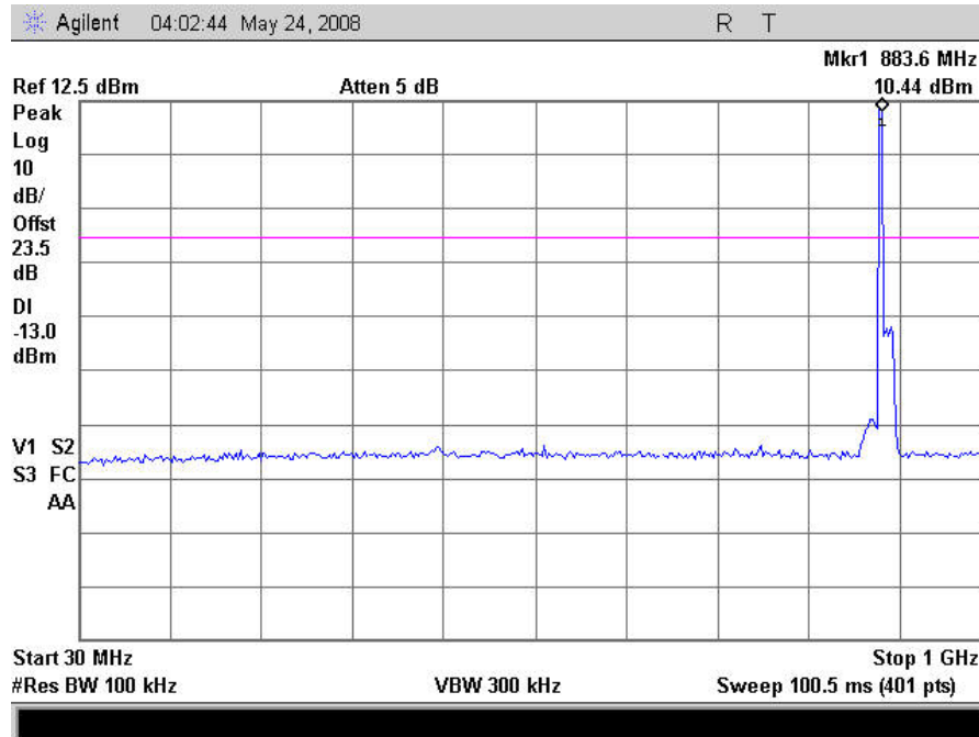
Plot 41. Conducted Spurious Emissions, CDMA Mid Channel Downlink, 30MHz – 1GHz
