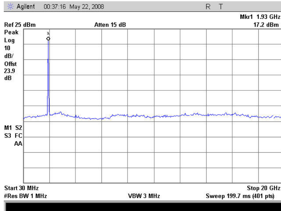
Plot 53. Conducted Spurious Emissions, CDMA Low Channel Downlink
