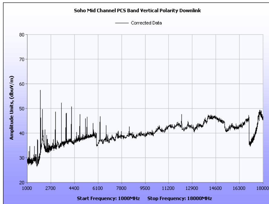
Plot 32. Radiated Spurious Emissions – Mid Channel, Vertical, Downlink, Corrected
