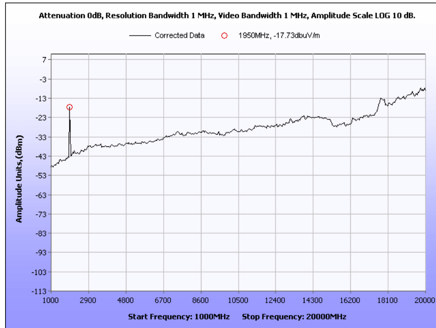
Plot 31. Radiated Spurious Emissions – Low Channel, Downlink, Corrected
