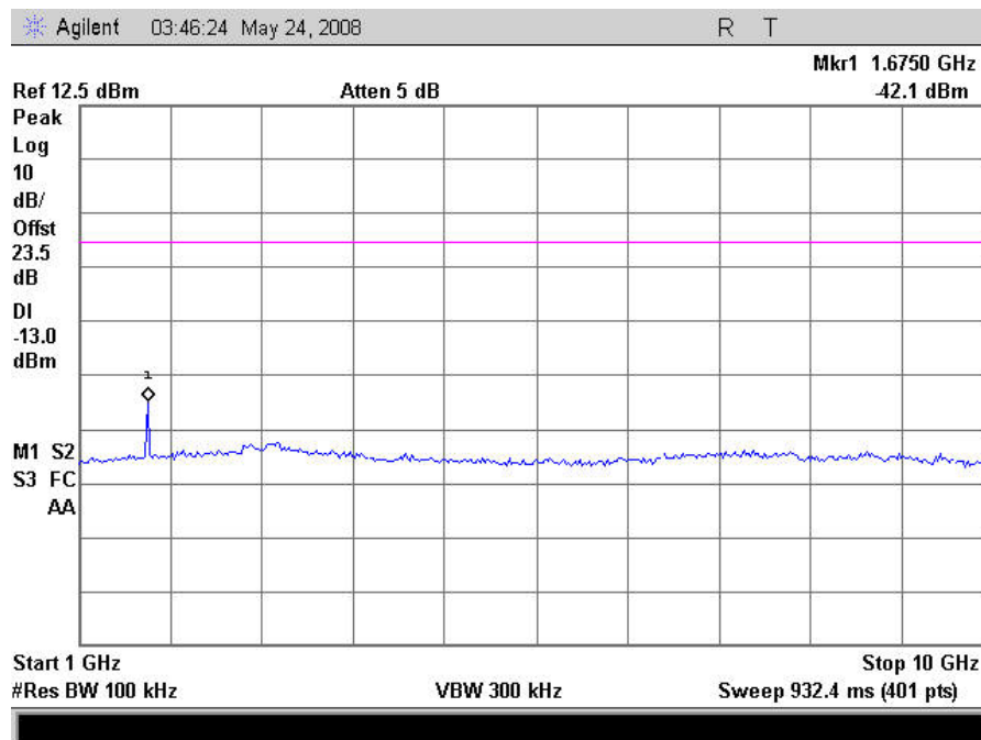
Plot 44. Conducted Spurious Emissions, CDMA Mid Channel Uplink, 1GHz – 10GHz
