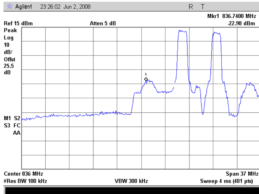
Plot 52. CDMA Intermodulation, Uplink High End
