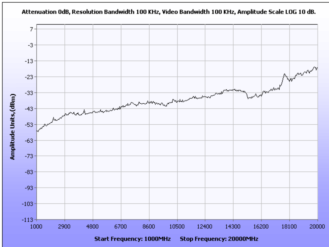
Plot 27. Radiated Spurious Emissions – High Channel, Downlink, Corrected
