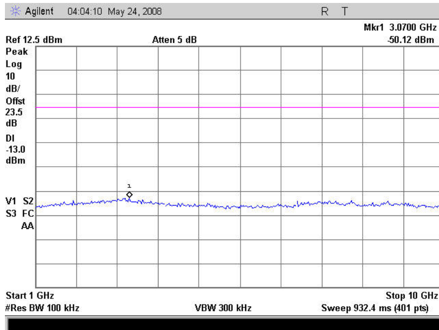
Plot 42. Conducted Spurious Emissions, CDMA Mid Channel Downlink, 1GHz – 10GHz
