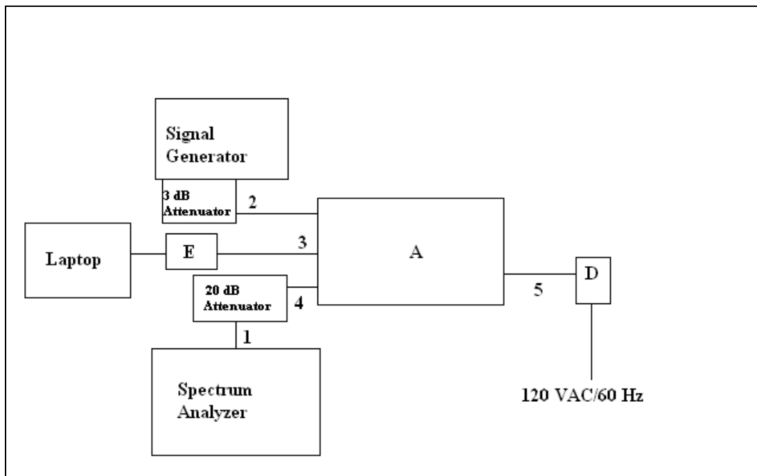
Figure 2. Block Diagram of Test Configuration (Downlink Conducted Measurement)
