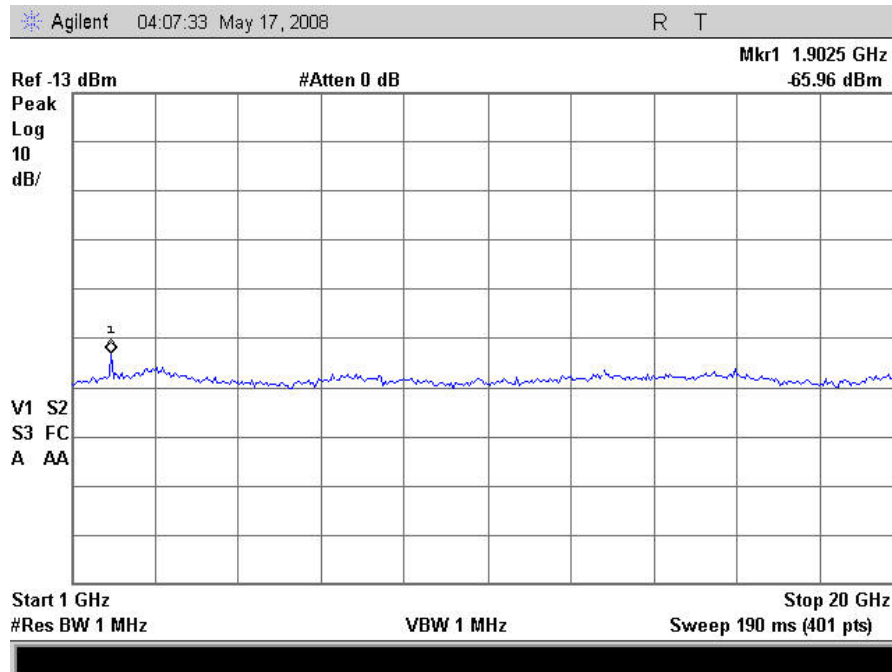
Plot 35. Radiated Spurious Emissions – Mid Channel, Uplink, Uncorrected
