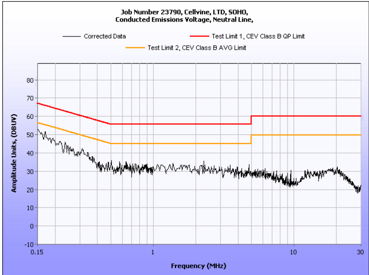
Conducted Emission, Neutral Line Peak Plot
