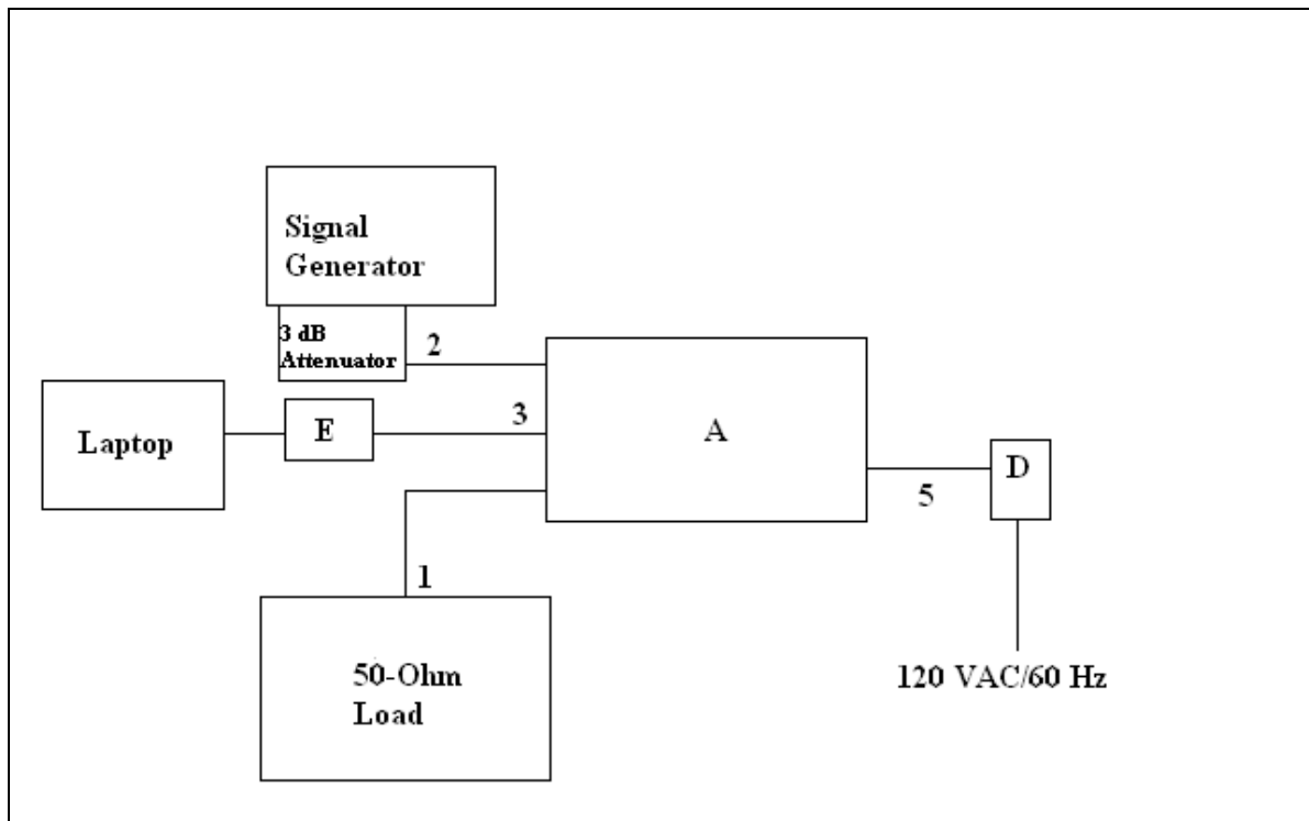
Figure 4. Block Diagram of Test Configuration (Downlink Radiated Measurement)
