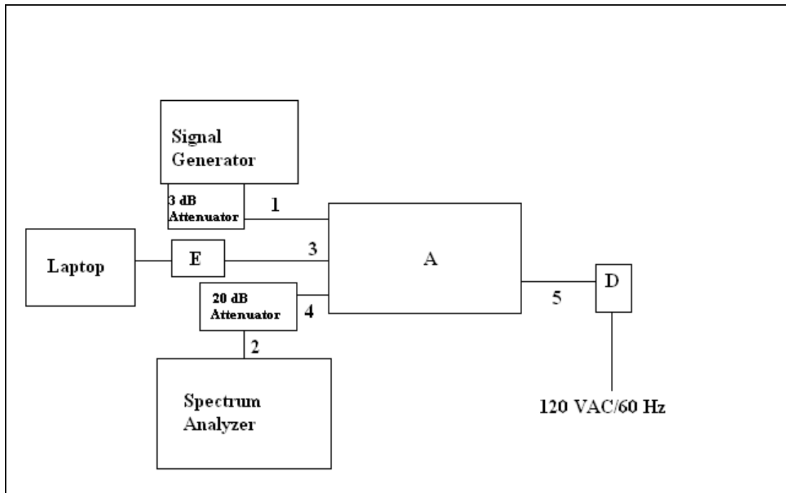
Figure 1. Block Diagram of Test Configuration (Uplink Conducted Measurement)
