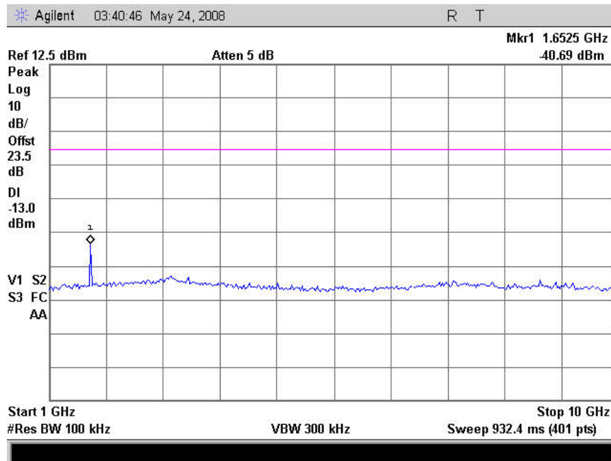
Plot 40. Conducted Spurious Emissions, CDMA Low Channel Uplink, 1GHz – 10GHz
