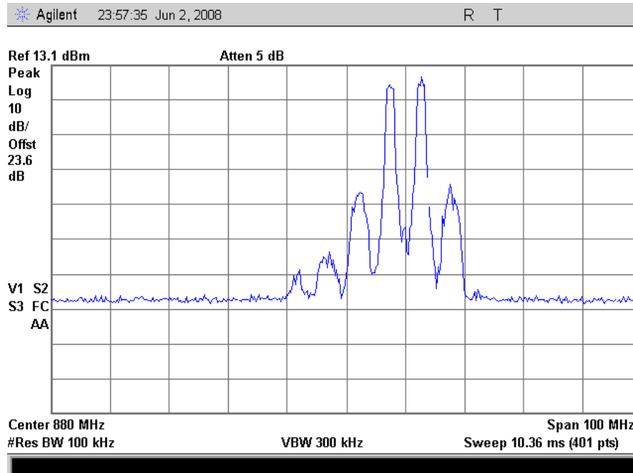
Plot 50. CDMA Intermodulation, Downlink High End
