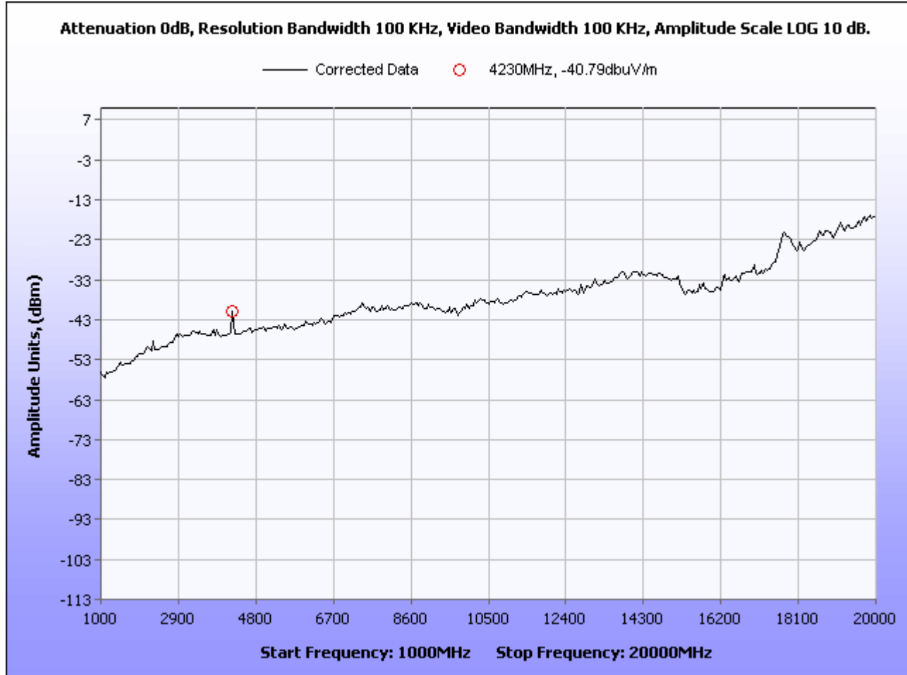
Plot 26. Radiated Spurious Emissions – Low Channel, Downlink, Corrected
