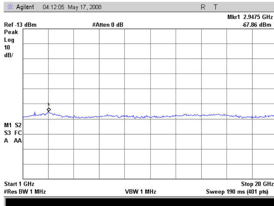
Plot 36. Radiated Spurious Emissions – High Channel, Uplink, Uncorrected
