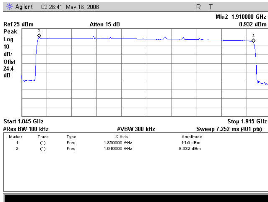
Plot 66. Out of Band Rejection, Uplink
