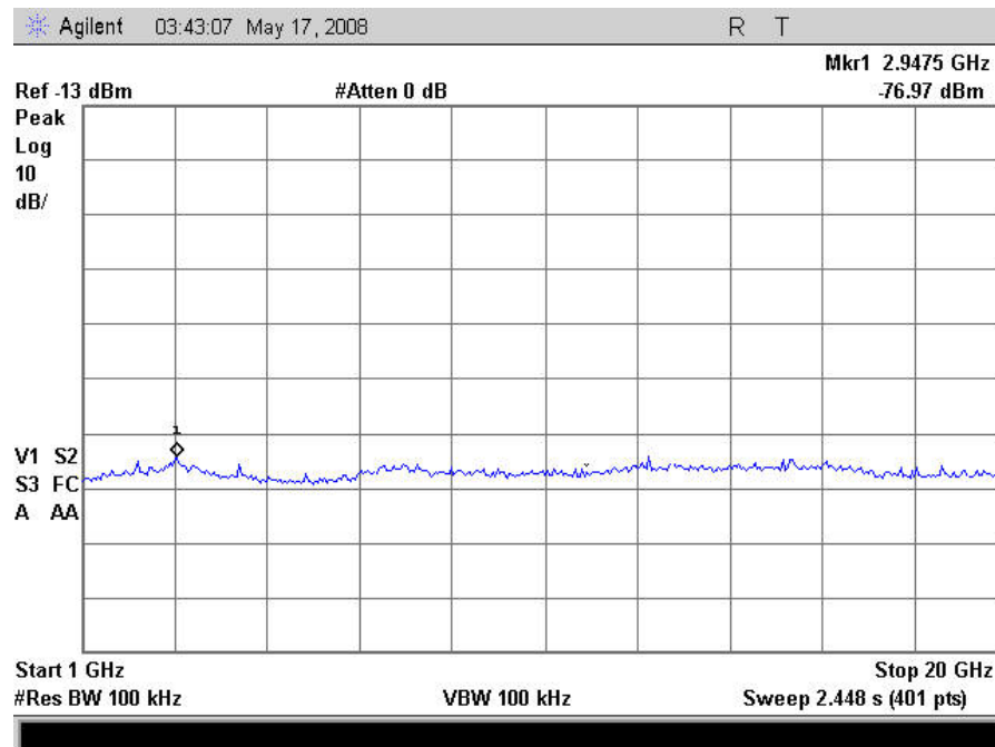
Plot 29. Radiated Spurious Emissions – Mid Channel, Uplink, Uncorrected
