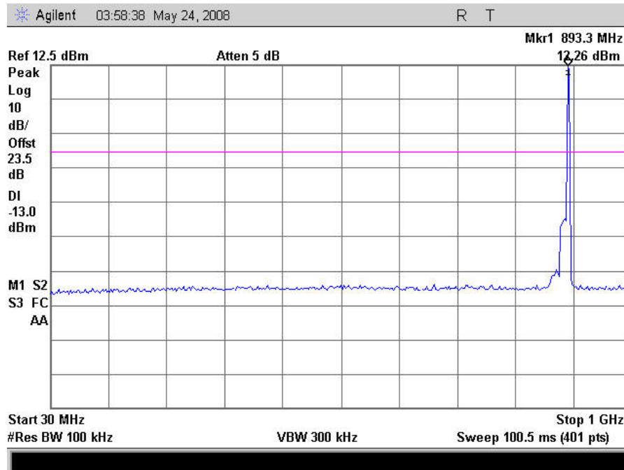
Plot 45. Conducted Spurious Emissions, CDMA High Channel Downlink, 30MHz – 1GHz
