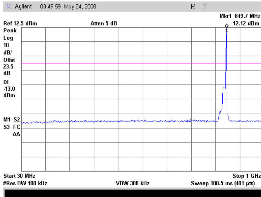
Plot 47. Conducted Spurious Emissions, CDMA High Channel Uplink, 30MHz – 1GHz
