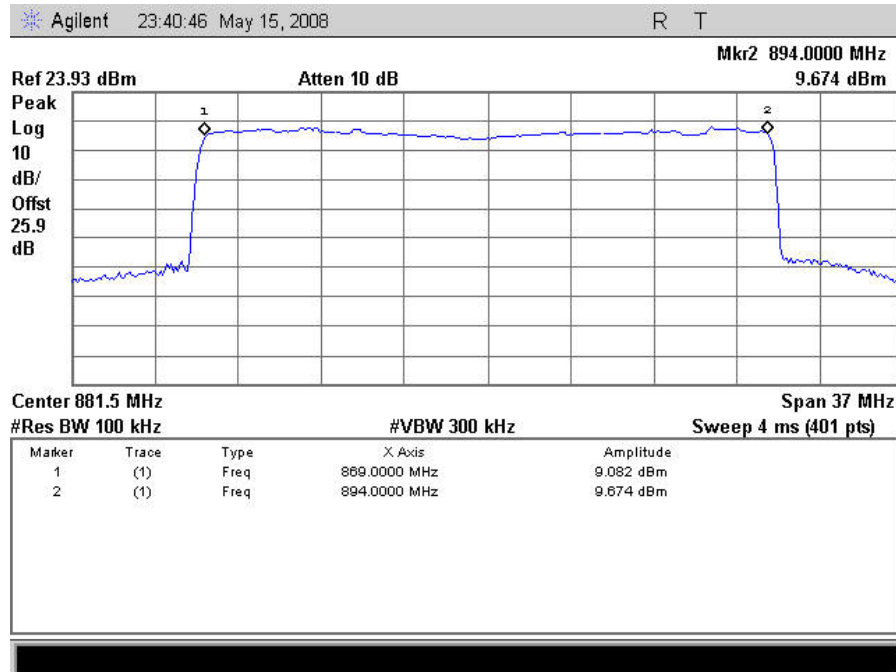
Plot 63. Out of Band Rejection, Downlink
