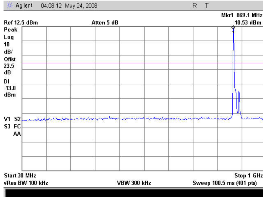
Plot 37. Conducted Spurious Emissions, CDMA Low Channel Downlink, 30MHz – 1GHz
