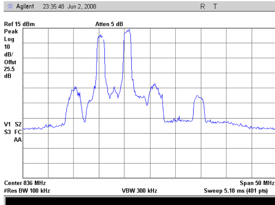
Plot 51. CDMA Intermodulation, Uplink Low End
