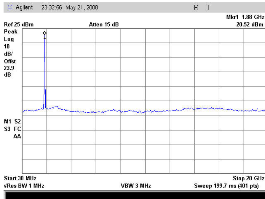
Plot 54. Conducted Spurious Emissions, CDMA Low Channel Uplink
