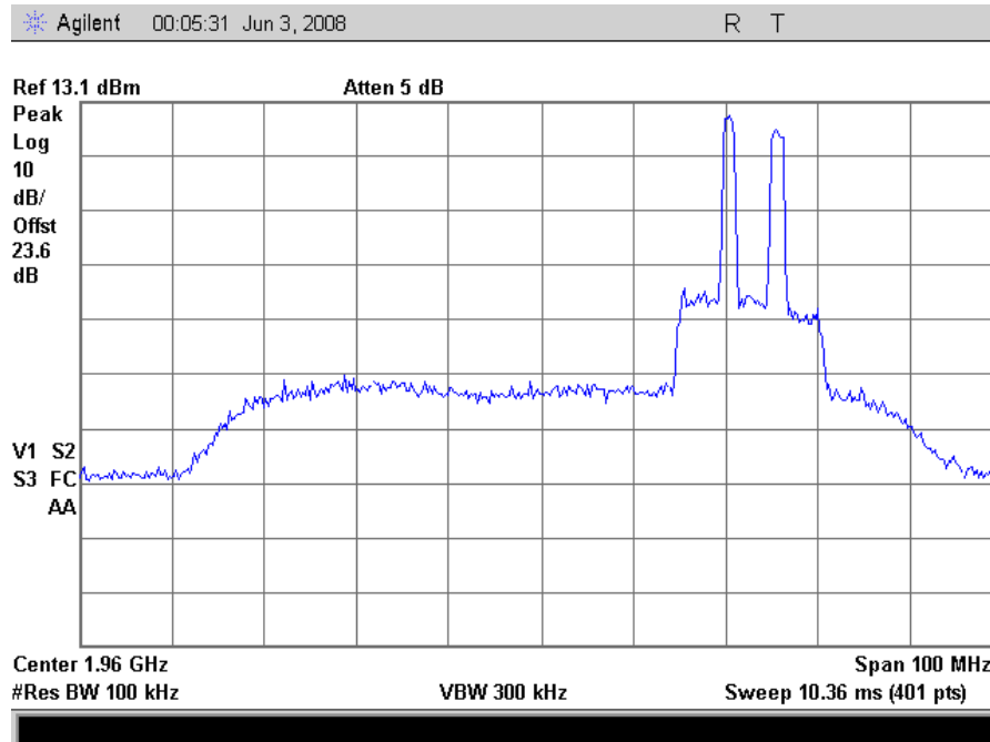
Plot 60. CDMA Intermodulation, Downlink High End
