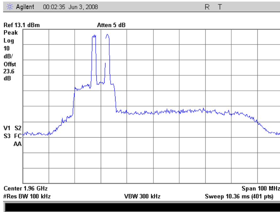
Plot 59. CDMA Intermodulation, Downlink Low End
