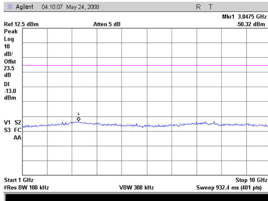
Plot 38. Conducted Spurious Emissions, CDMA Low Channel Downlink, 1GHz – 10GHz
