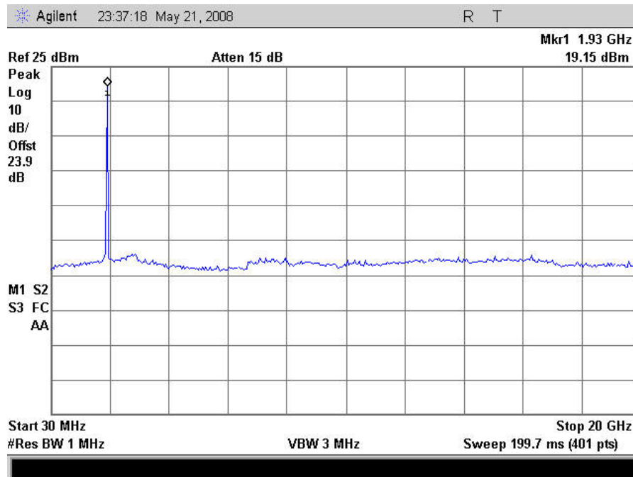
Plot 58. Conducted Spurious Emissions, CDMA High Channel Uplink
