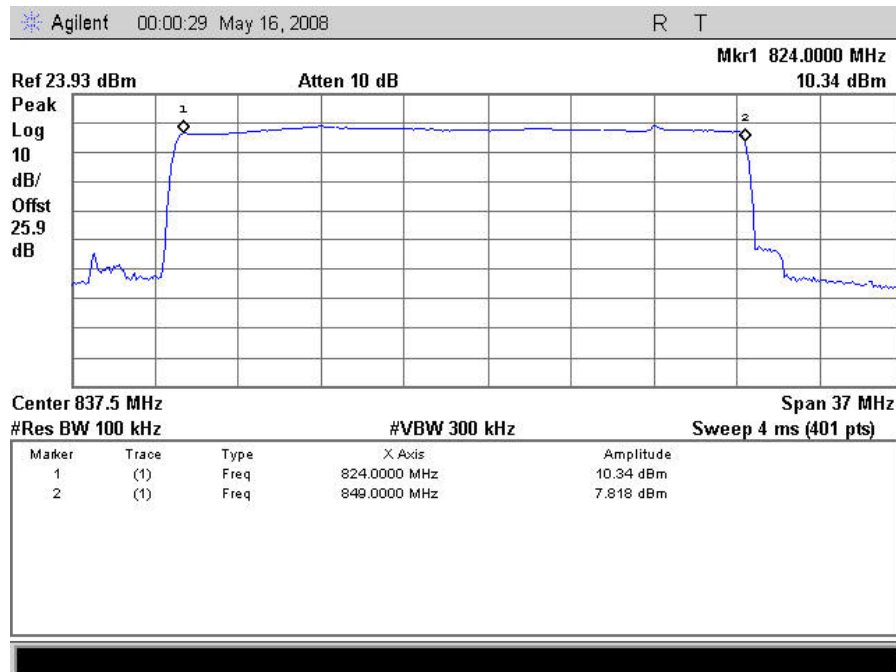
Plot 64. Out of Band Rejection, Uplink
