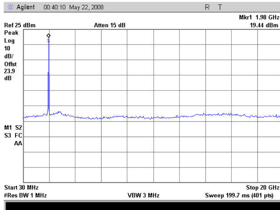
Plot 55. Conducted Spurious Emissions, CDMA Mid Channel Downlink
