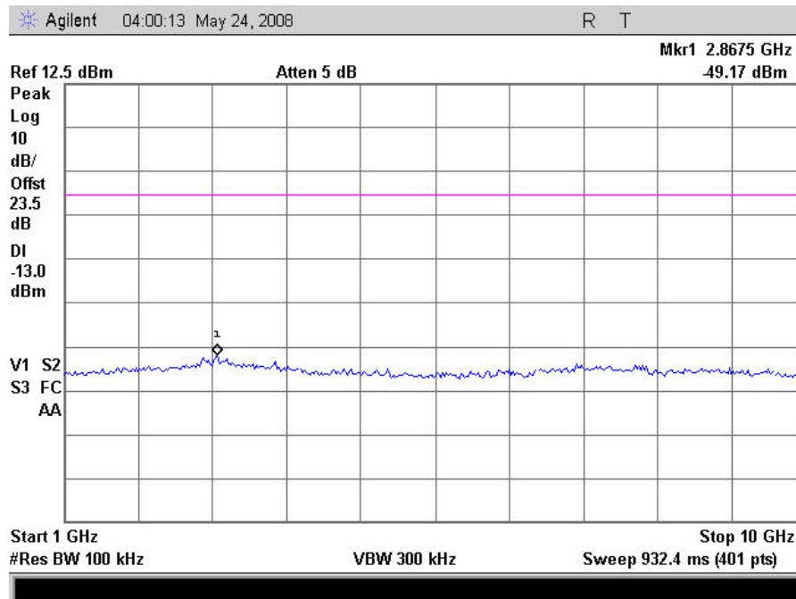
Plot 46. Conducted Spurious Emissions, CDMA High Channel Downlink, 1GHz – 10GHz
