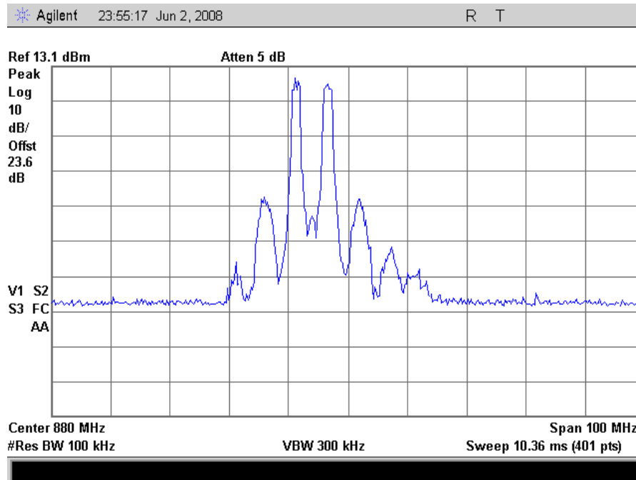
Plot 49. CDMA Intermodulation, Downlink Low End
