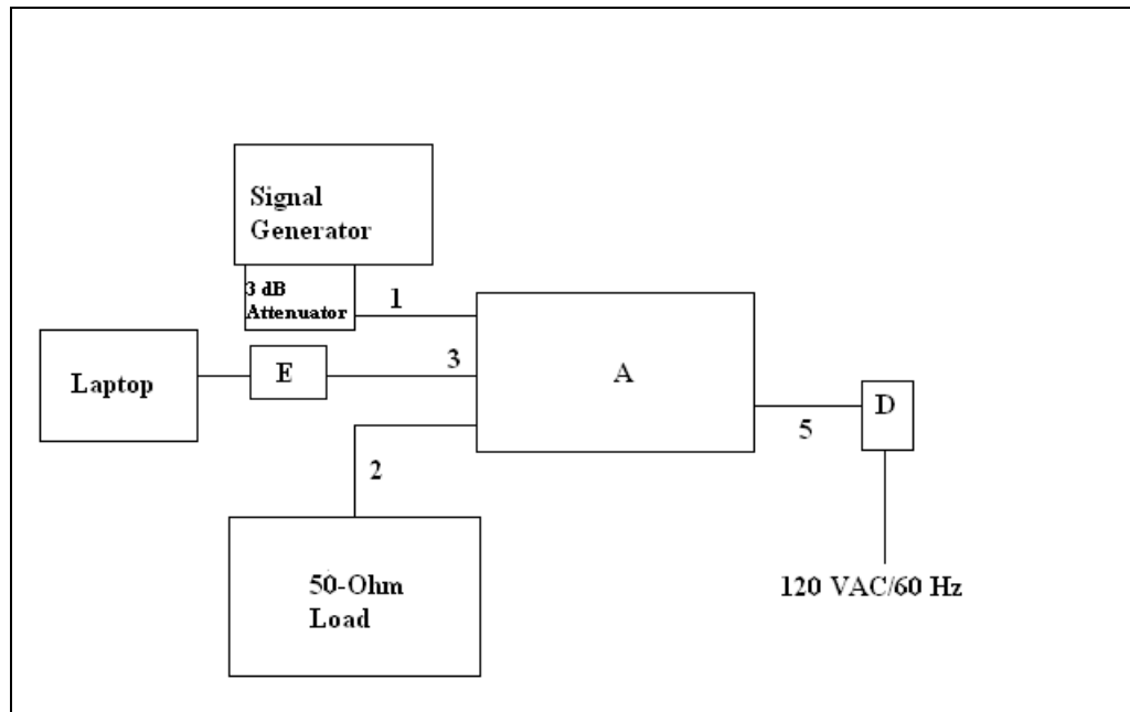
Figure 3. Block Diagram of Test Configuration (Uplink Radiated Measurement)
