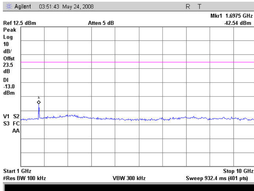
Plot 48. Conducted Spurious Emissions, CDMA High Channel Uplink, 1GHz – 10GHz
