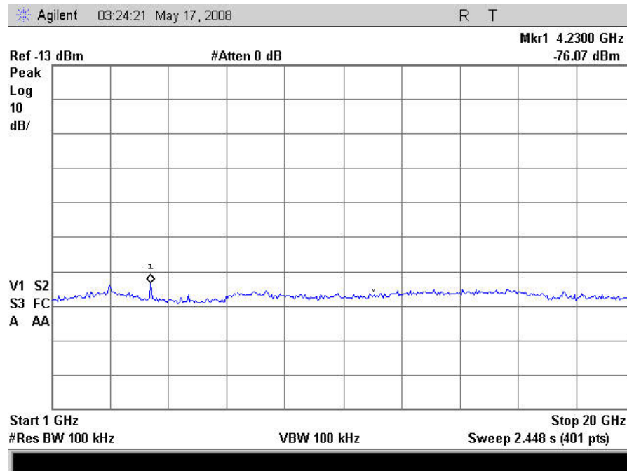
Plot 28. Radiated Spurious Emissions – Low Channel, Uplink, Uncorrected
