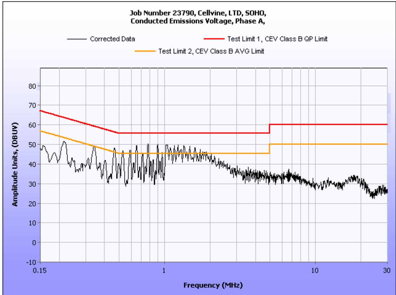
Conducted Emission, Phase Line Peak Plot
