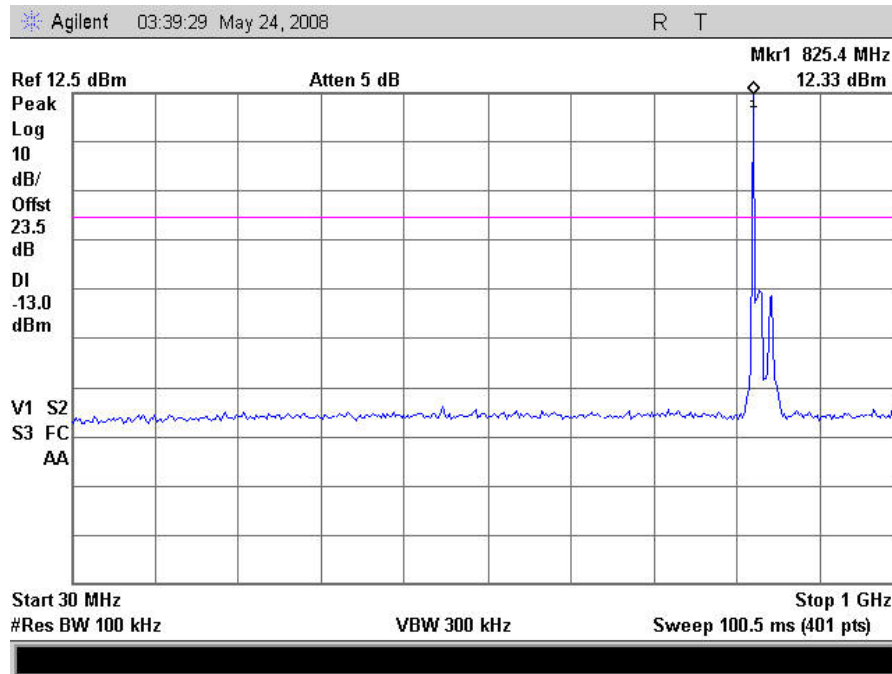
Plot 39. Conducted Spurious Emissions, CDMA Low Channel Uplink, 30MHz – 1GHz
