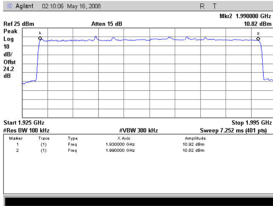
Plot 65. Out of Band Rejection, Downlink
