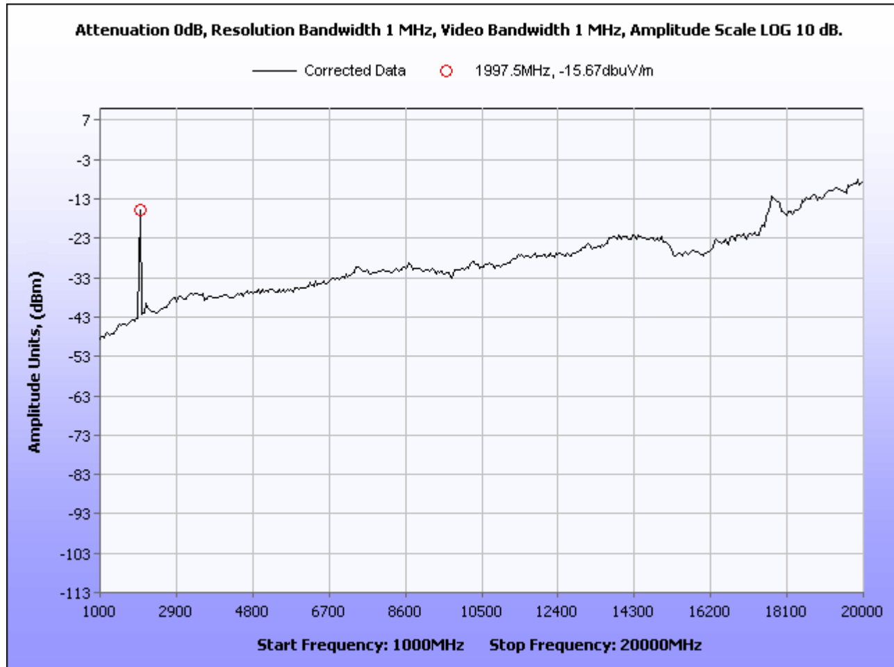
Plot 33. Radiated Spurious Emissions – High Channel, Downlink, Corrected, Uncorrected
