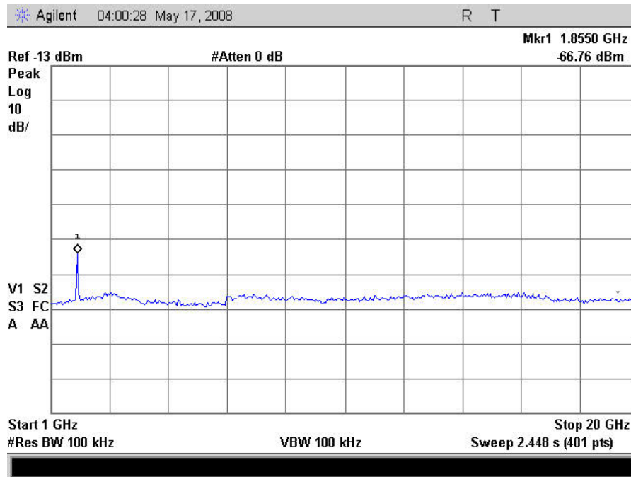
Plot 34. Radiated Spurious Emissions – Low Channel, , Uplink, Uncorrected
