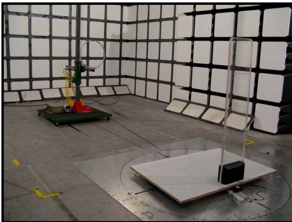
Radiated Emissions - Rear View (Below 30 MHz)
