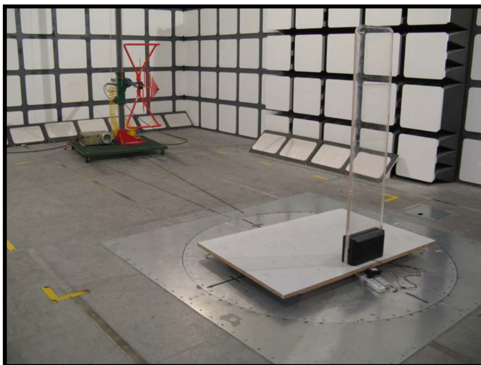
Radiated Emissions - Rear View (Above 30 MHz)
