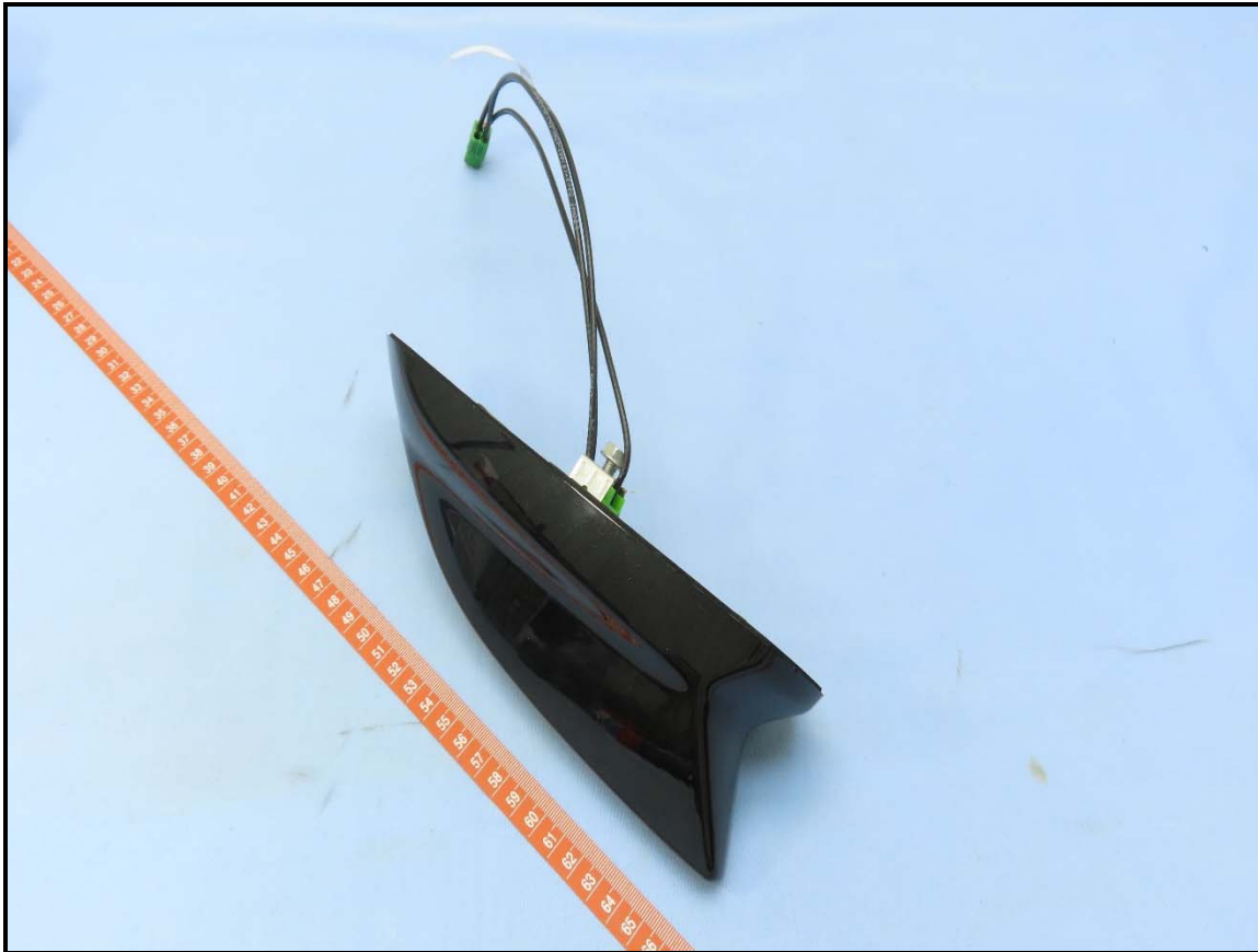
Antenna_LTE/GNSS (Model: 85004261)
