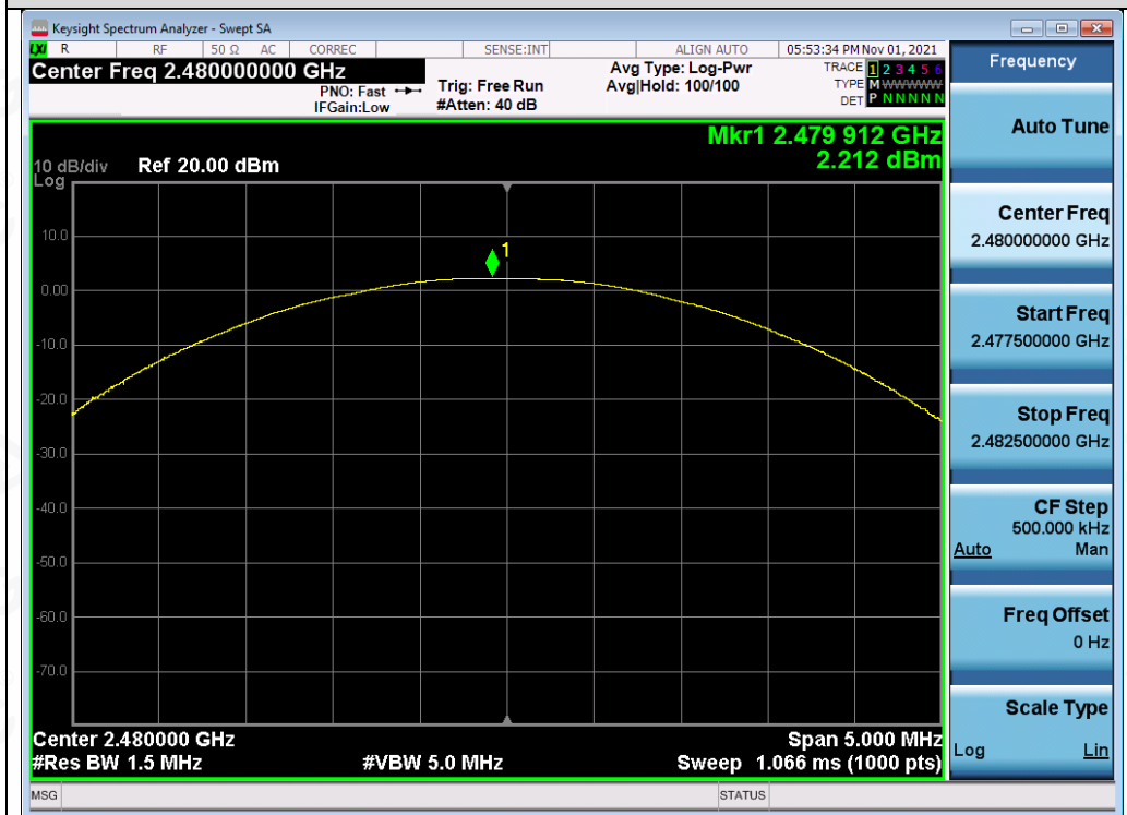
Test_Graph_EDR_ANT1_2480_3Mbps_Peak Power
