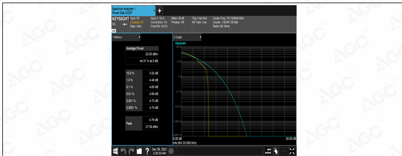
Band12-5MHz-16QAM-23095-25RB#0
