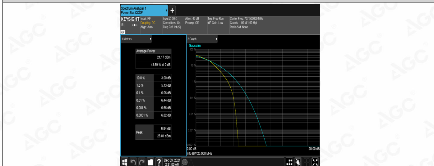
Band12-5MHz-16QAM-23155-1RB#0
